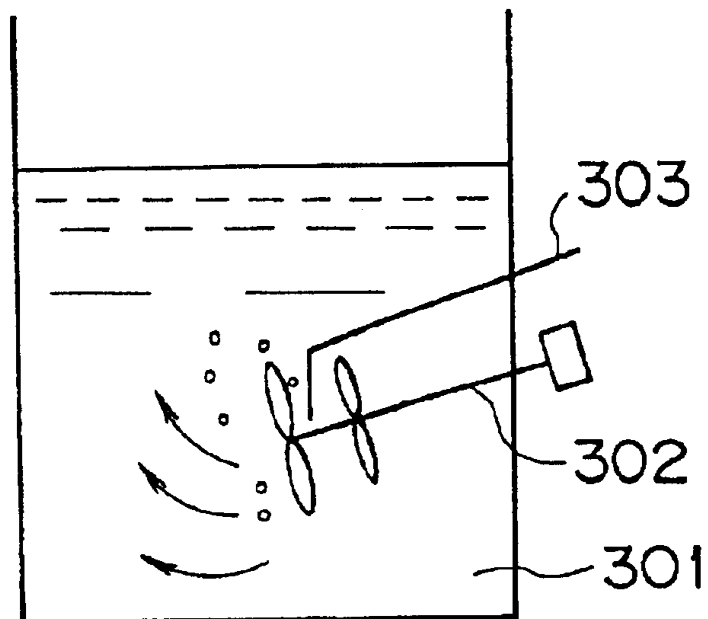
FIG. 8 (PRIOR ART)
