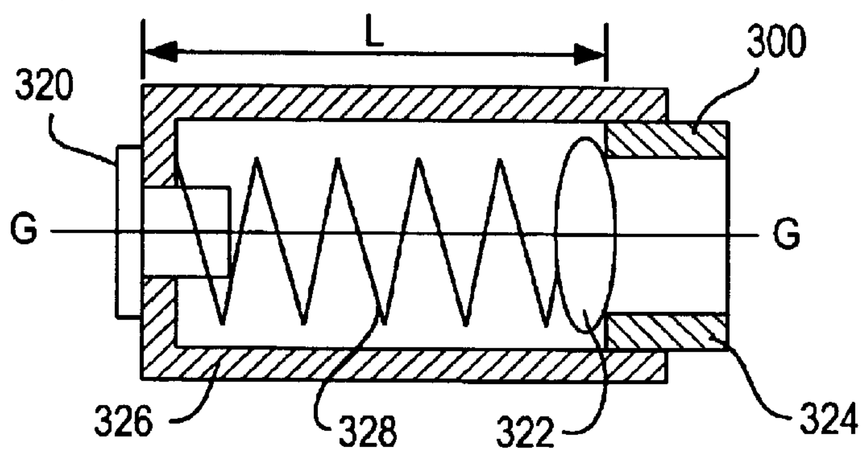
Figure 16 (PRIOR ART)
