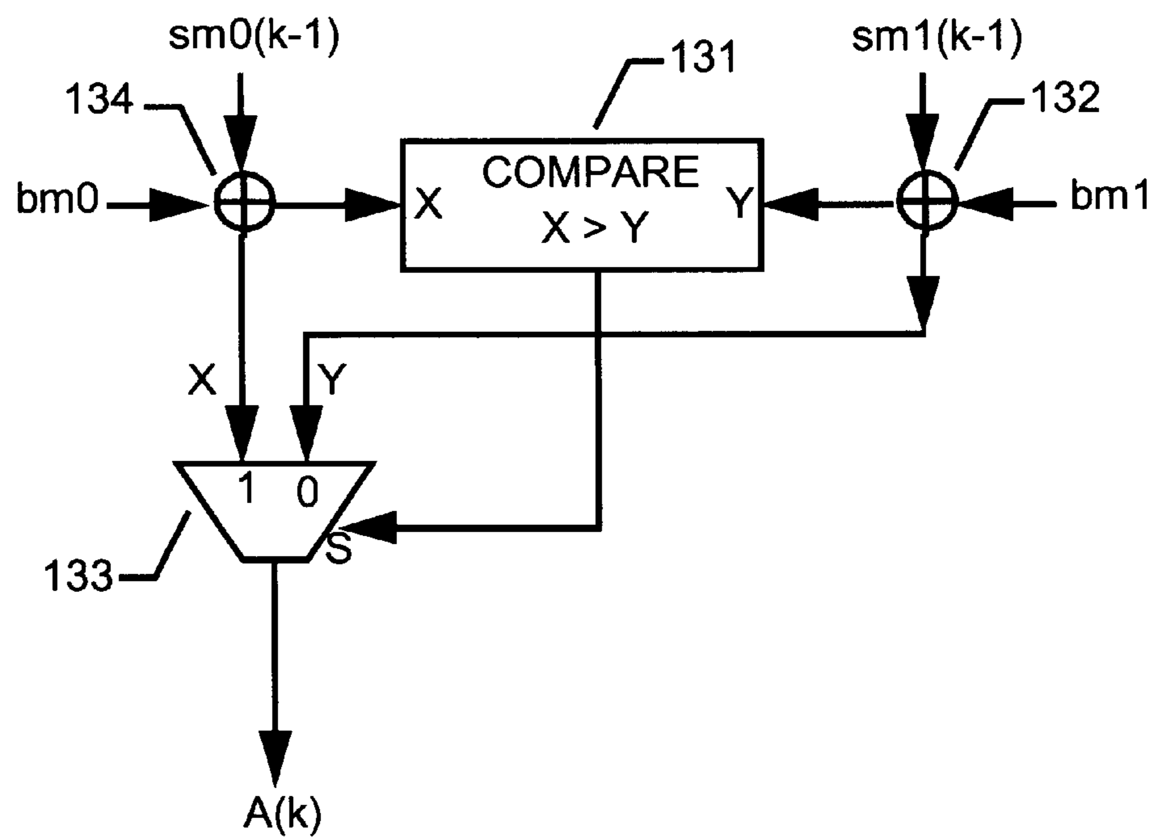
FIGURE 13. Computation of Forward Recursion of state-metric (ACS)
