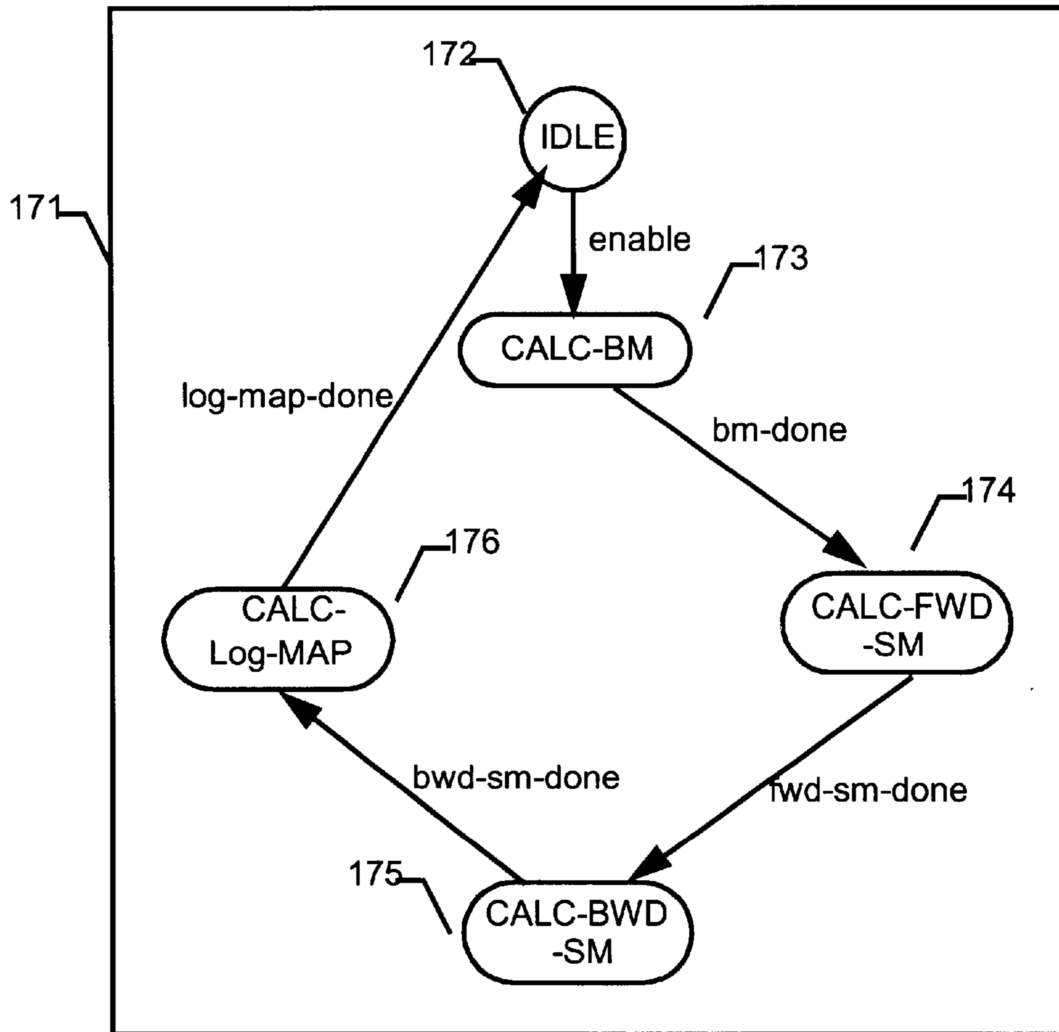
FIGURE 17. State machine operations of Log-MAP Decoder
