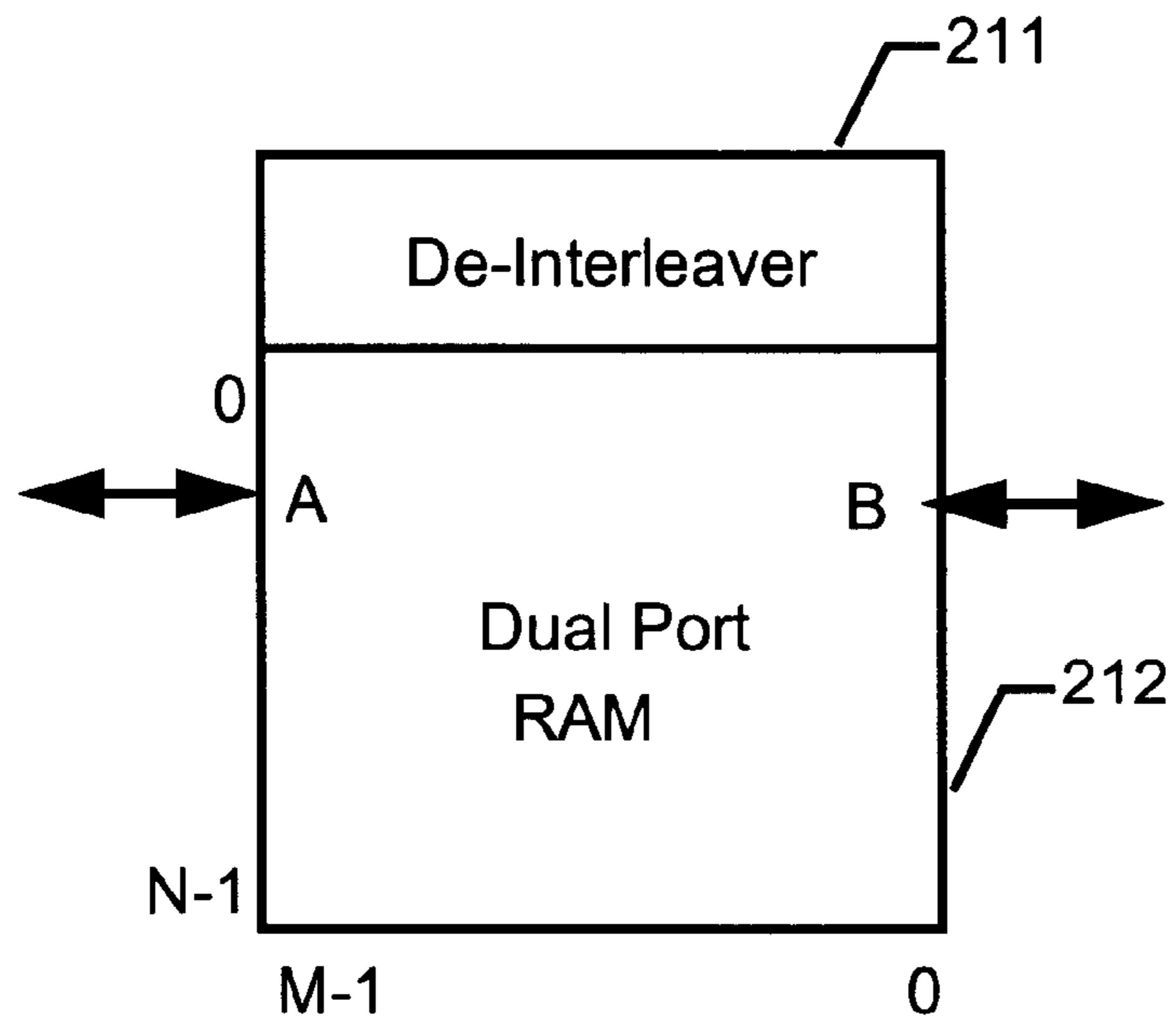
FIGURE 21. De-Interleaver RAM Memory Module
