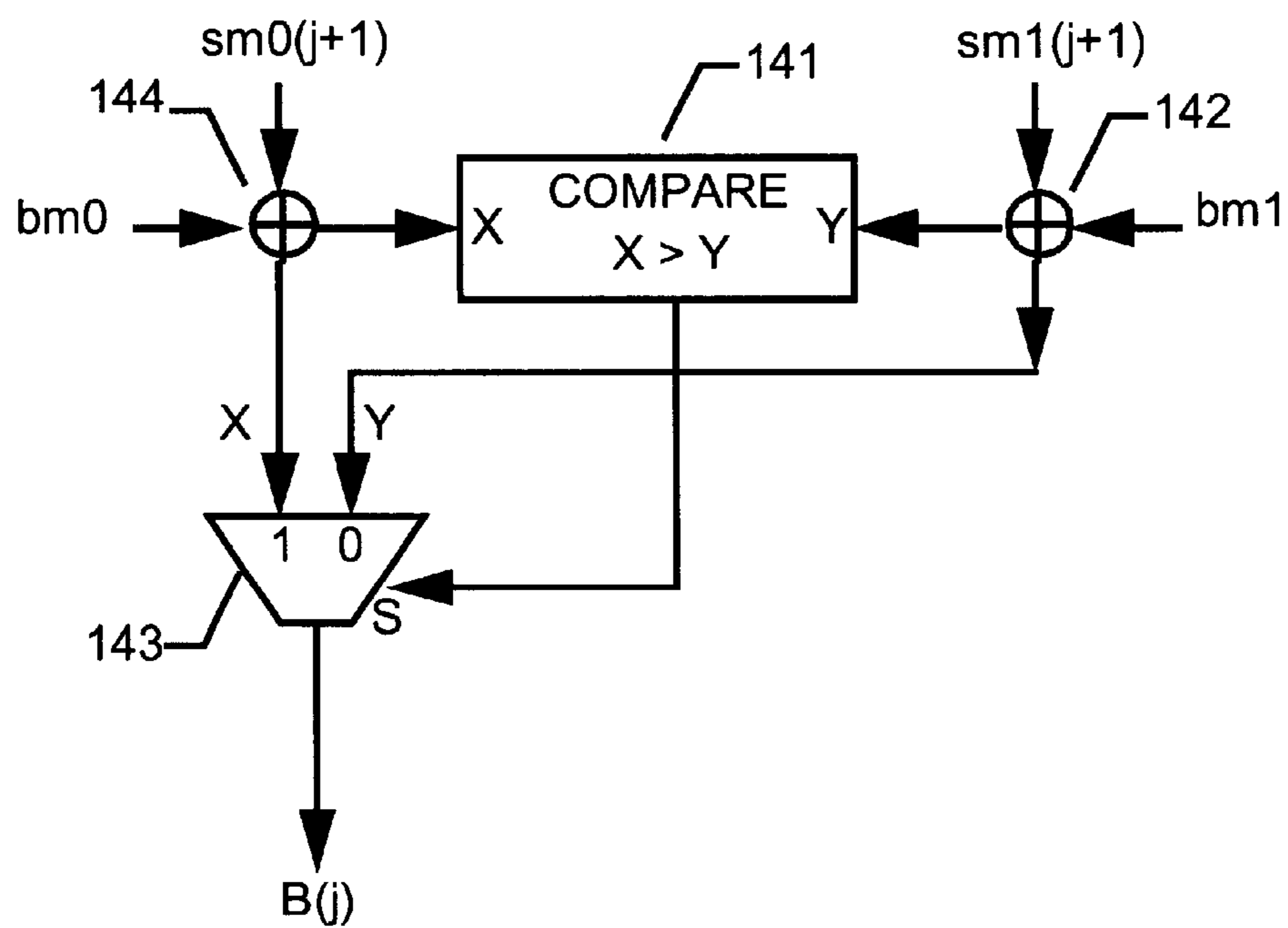
FIGURE 14. Computation of Backward Recursion of state-metric (ACS)
