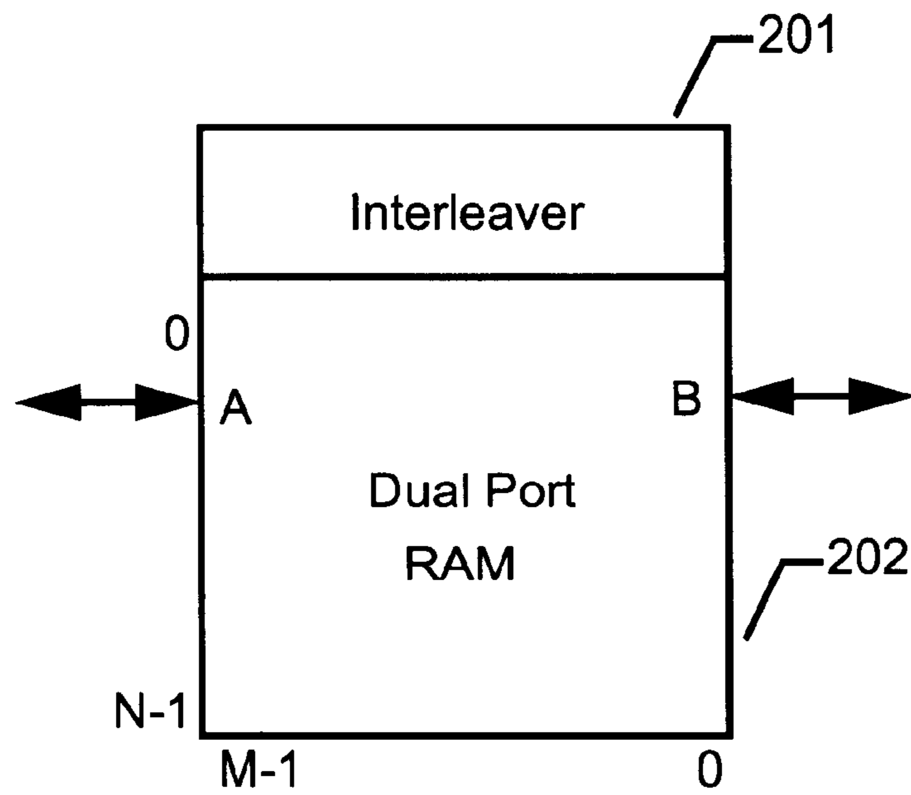
FIGURE 20. Interleaver RAM Memory Module
