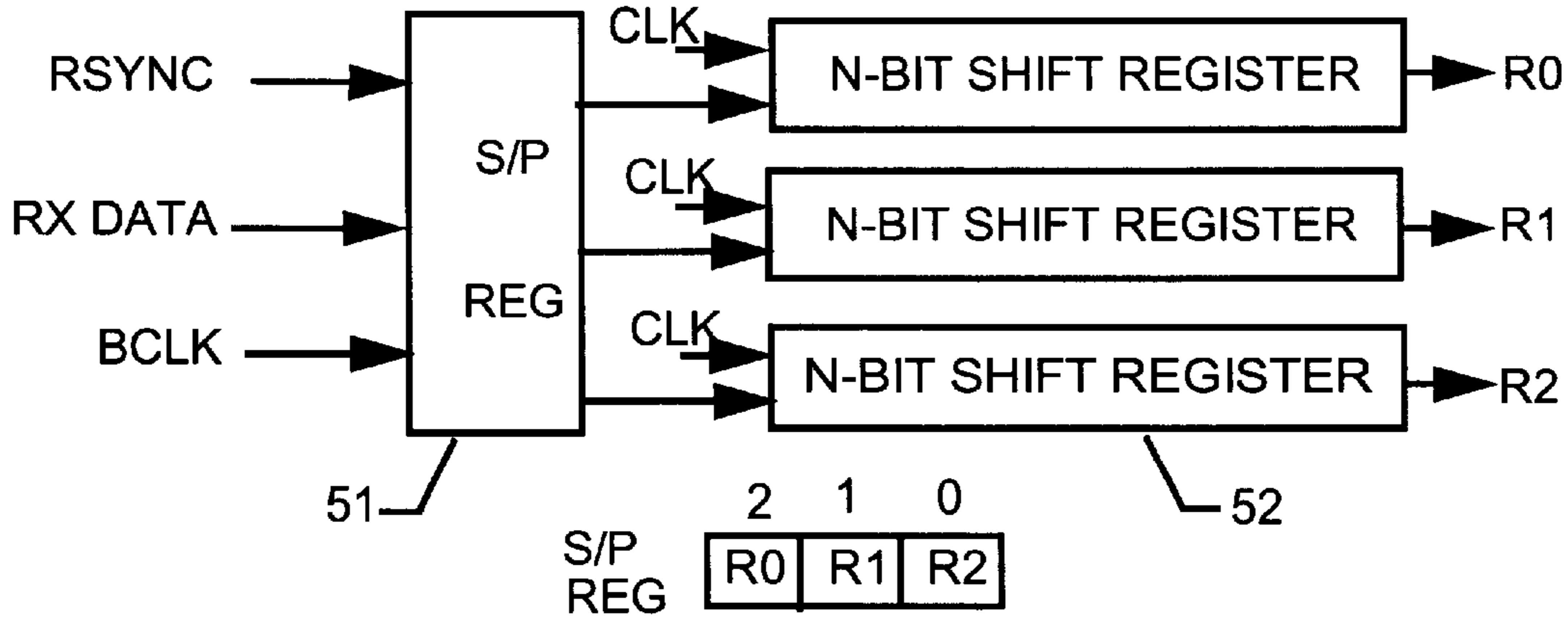
FIGURE 5. Input Buffer Shift Registers
