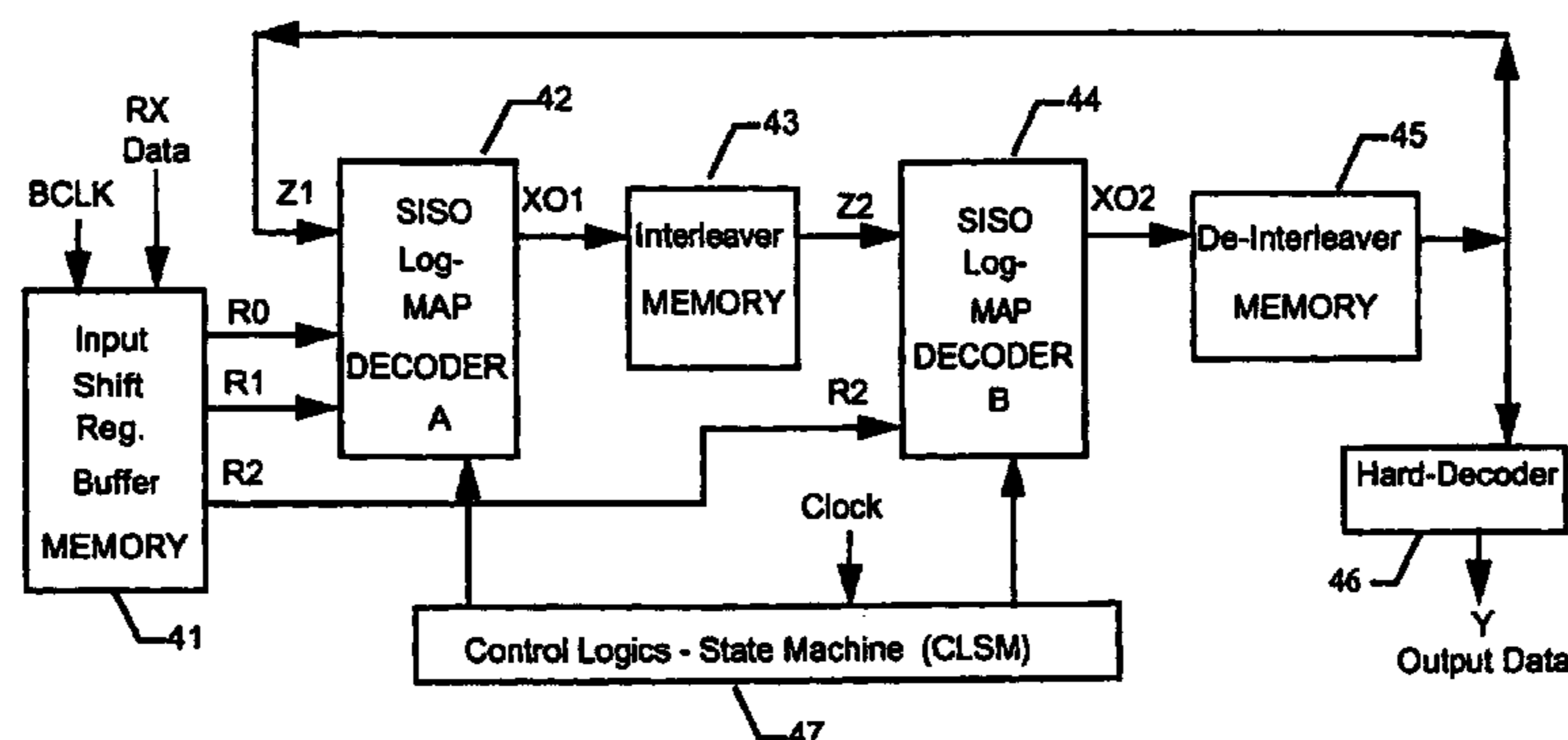
Turbo Codes Decoder System Block Diagram
