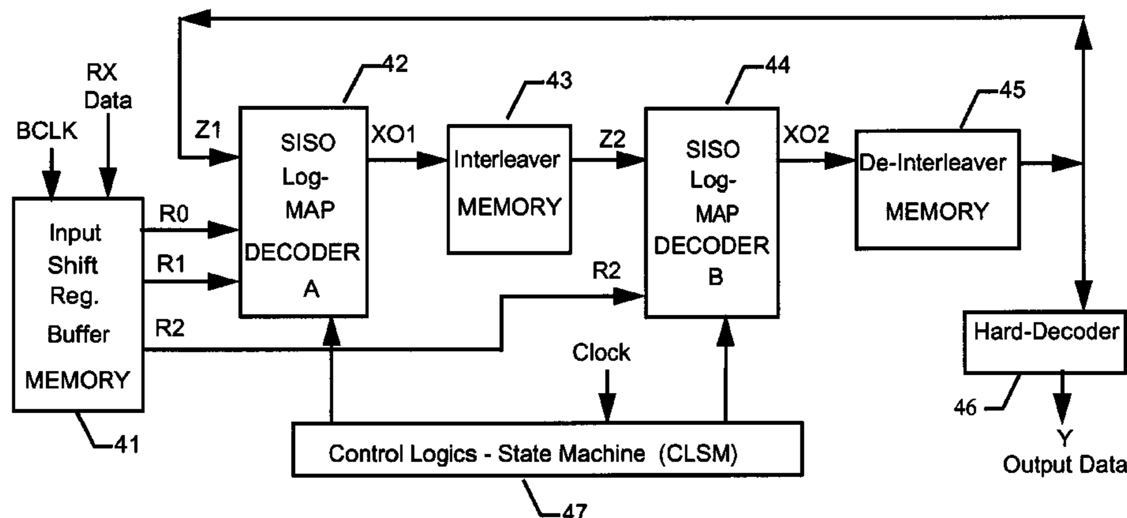
Turbo Codes Decoder System Block Diagram
