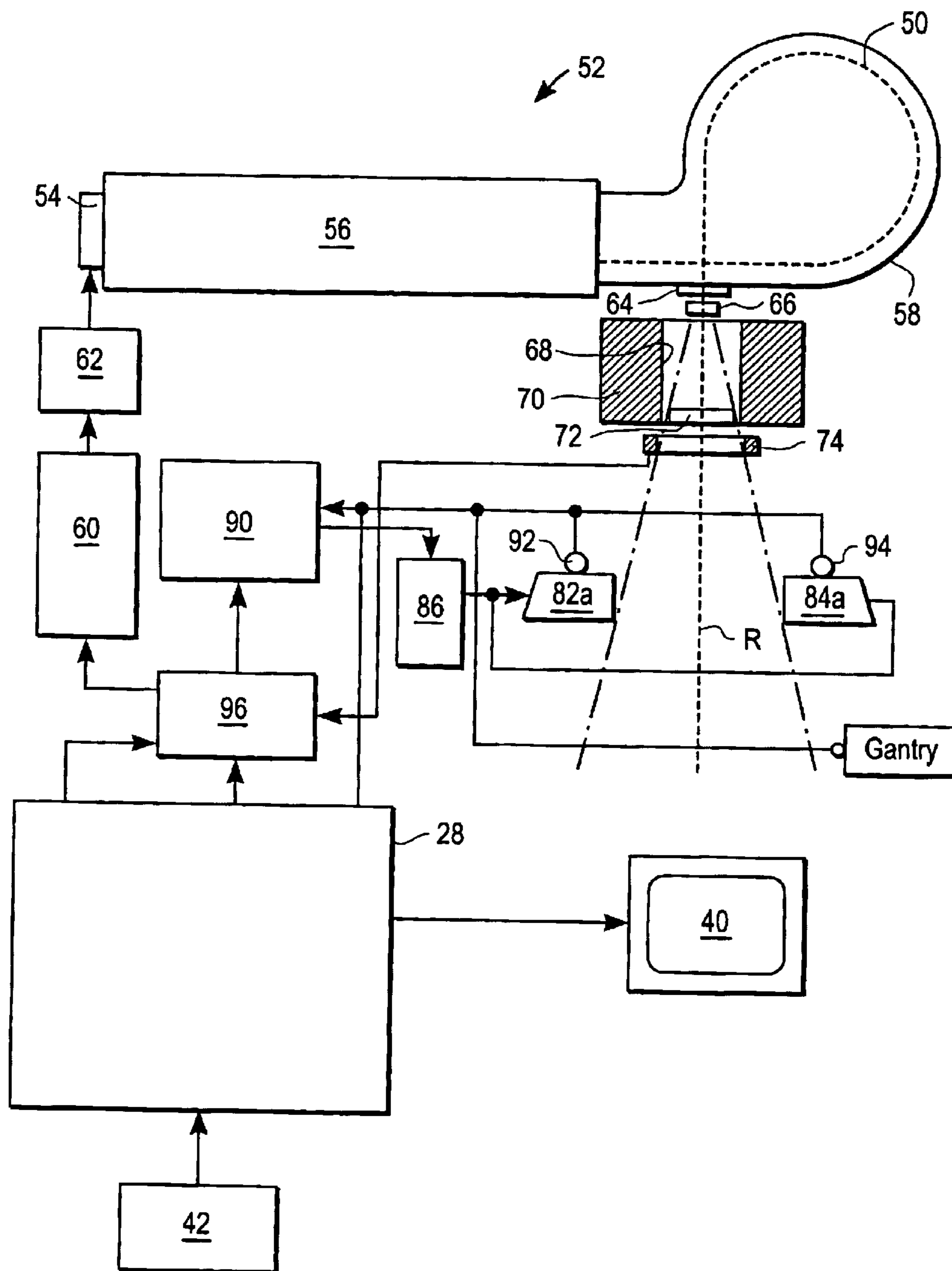
FIG. 2 (PRIOR ART)
