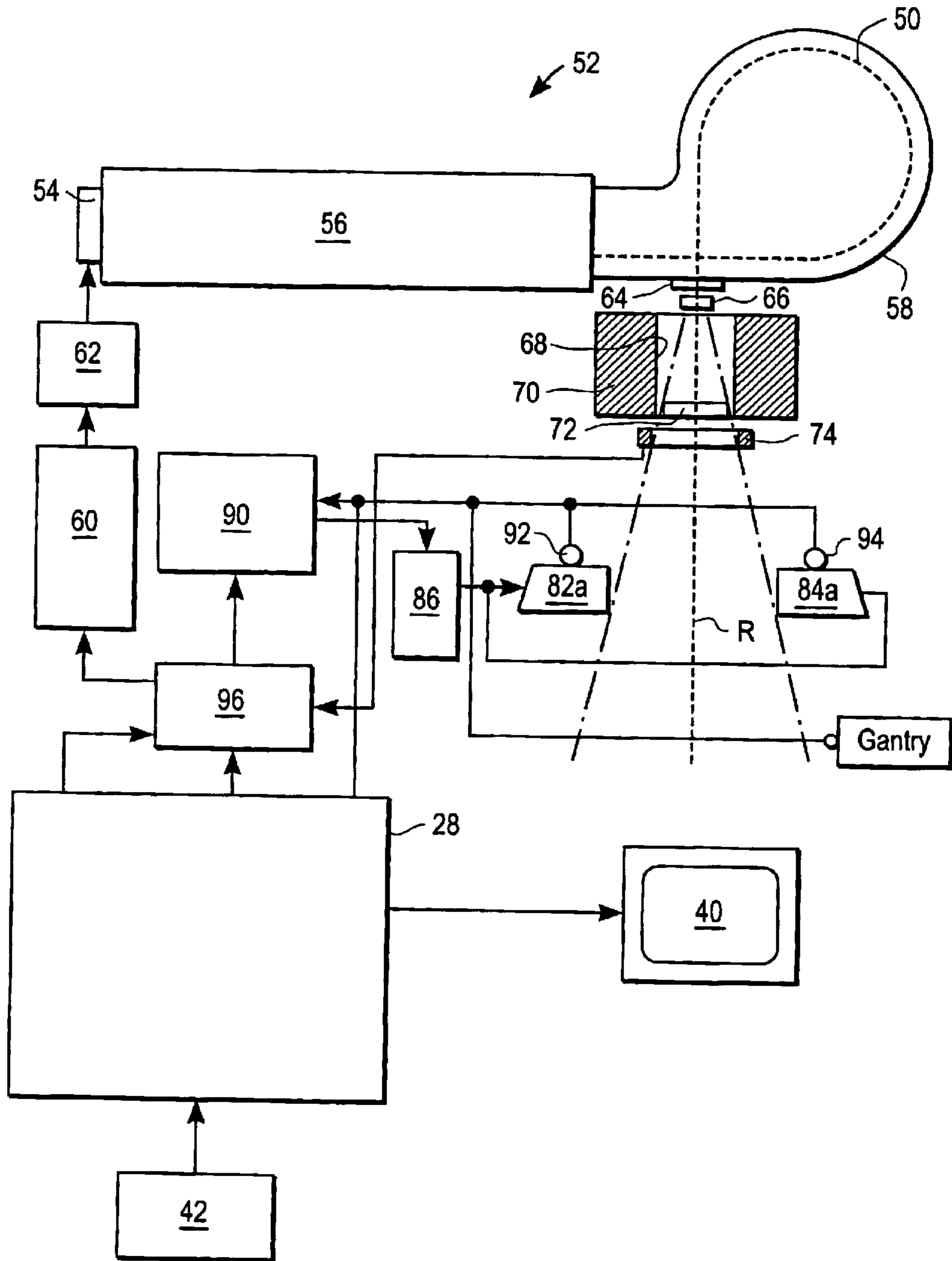
FIG. 2 (PRIOR ART)
