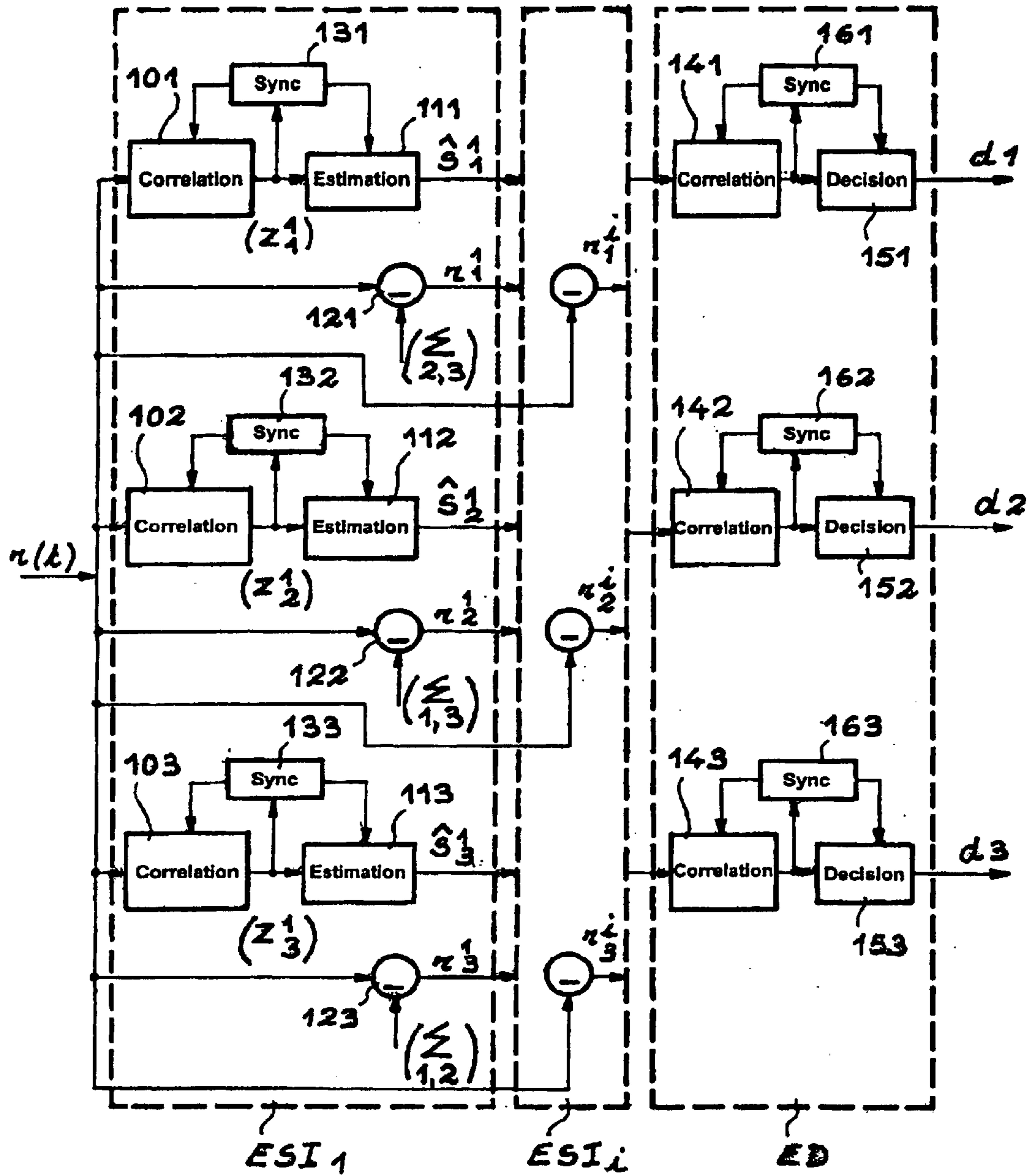
FIG. 7 - PRIOR ART -
