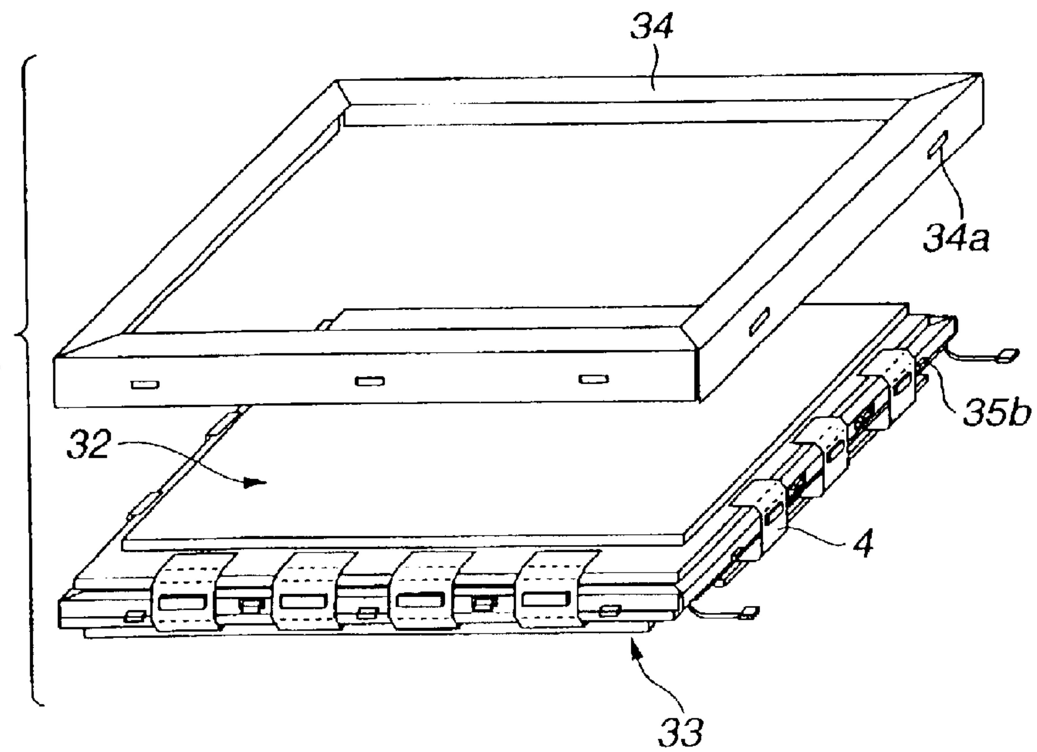
FIG.29 PRIOR ART
