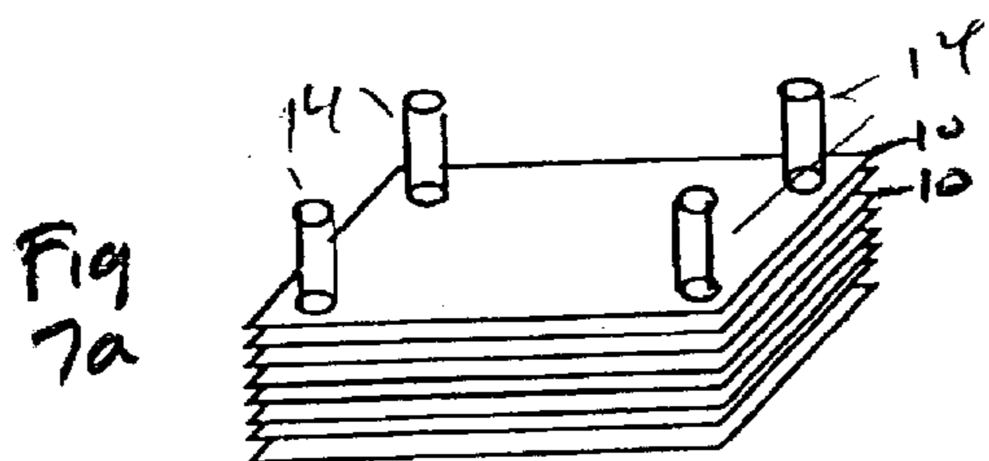
Figure 7 One possible way of reconfiguring the material is through a set of alignment pins, which could tilt the entire stack in various directions, and steer the transmitted beam.
