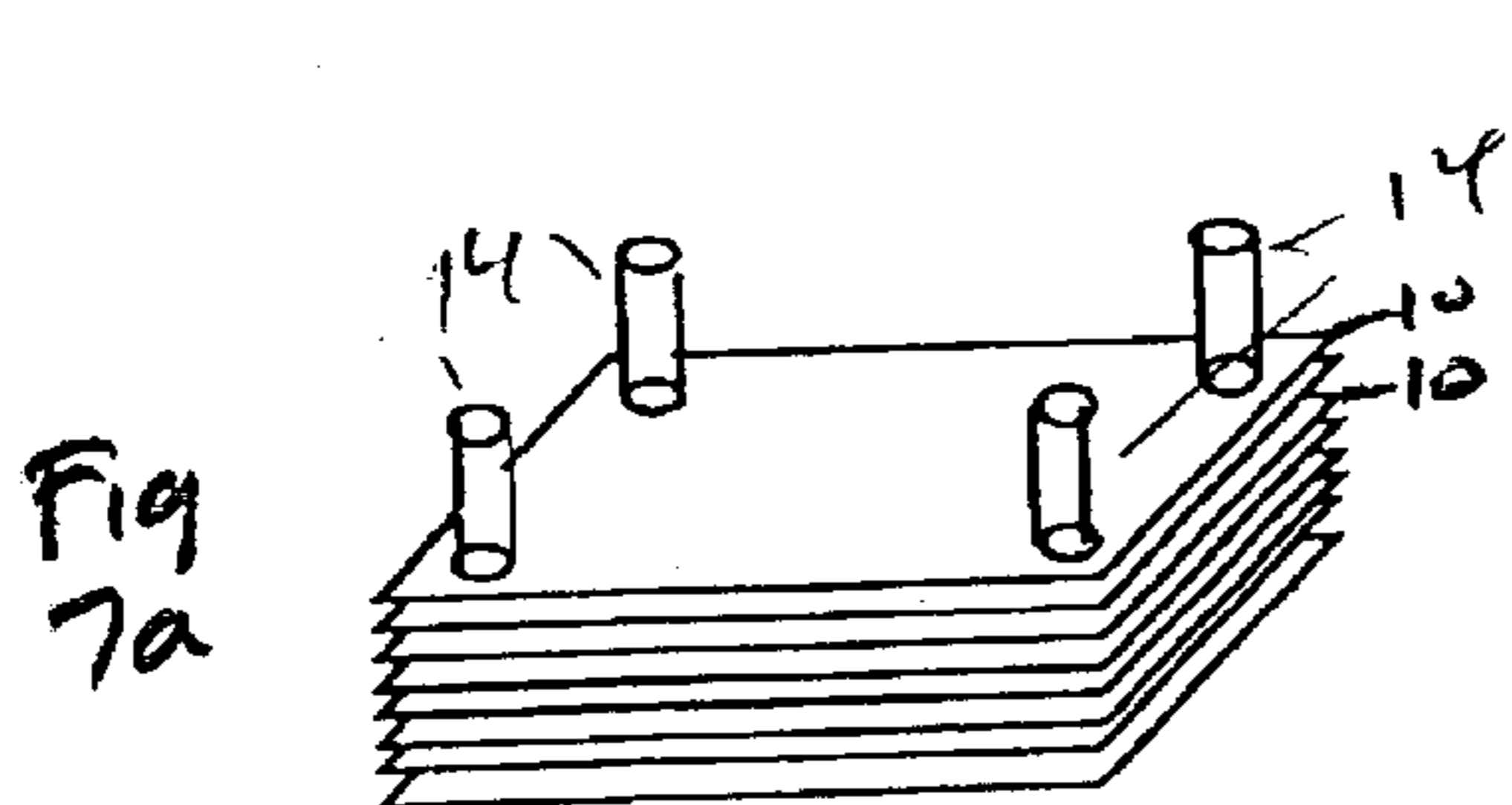
Figure 7 One possible way of reconfiguring the material is through a set of alignment pins, which could tilt the entire stack in various directions, and steer the transmitted beam.
