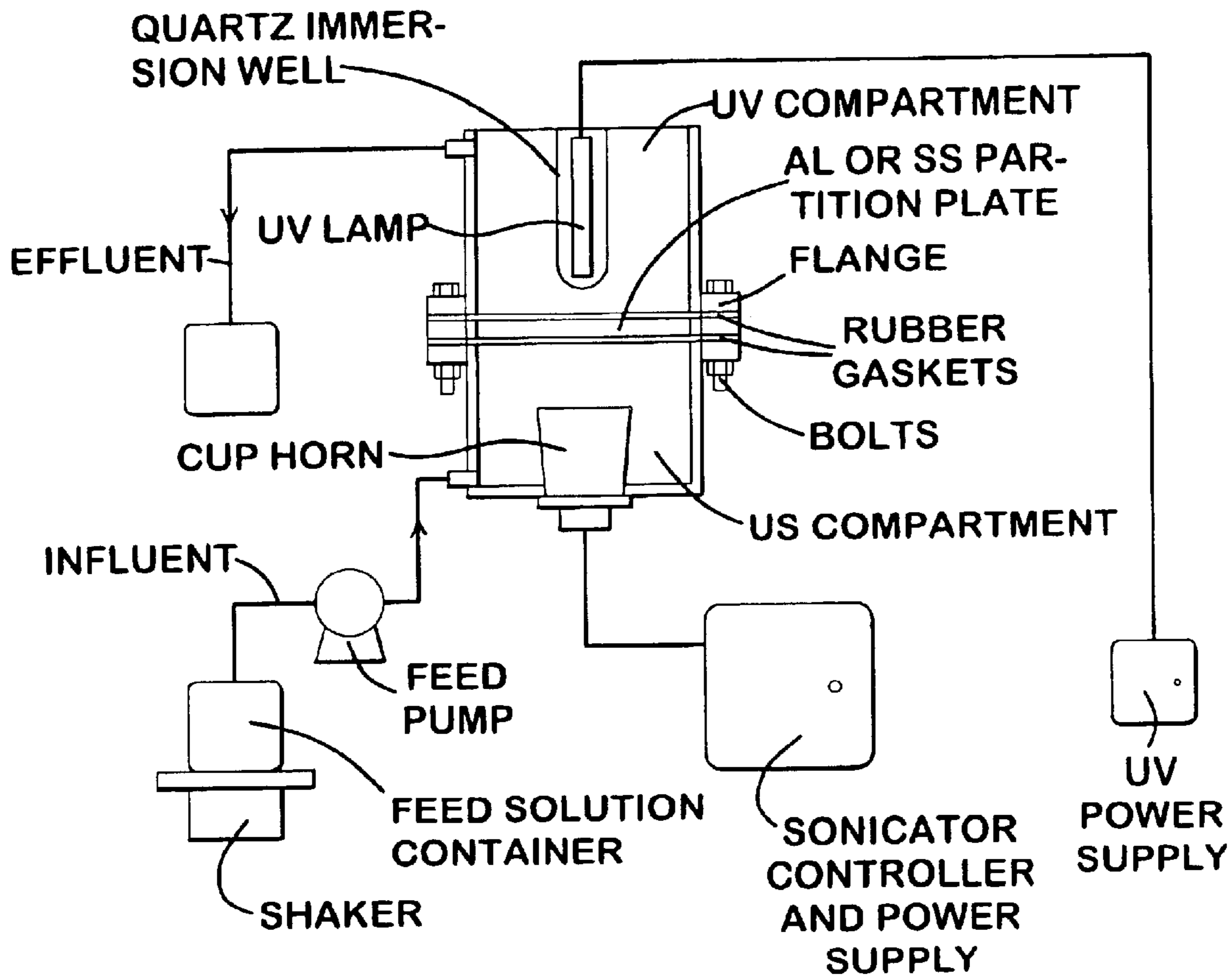
Fig. 10 THE UVUS REACTOR SYSTEM
