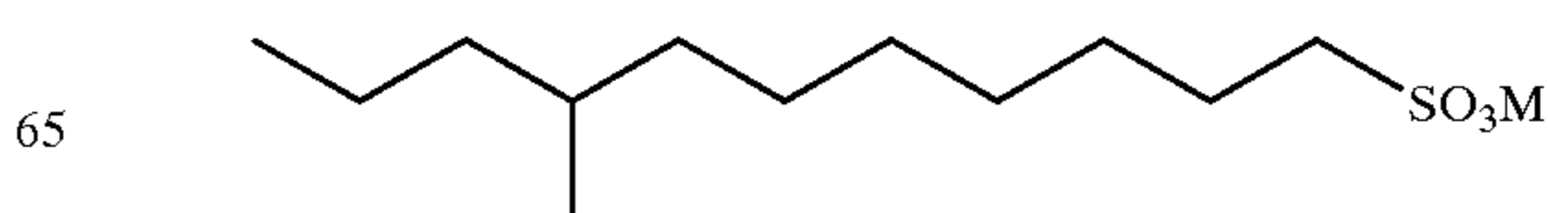
8-Methylundecyl sulfate:
