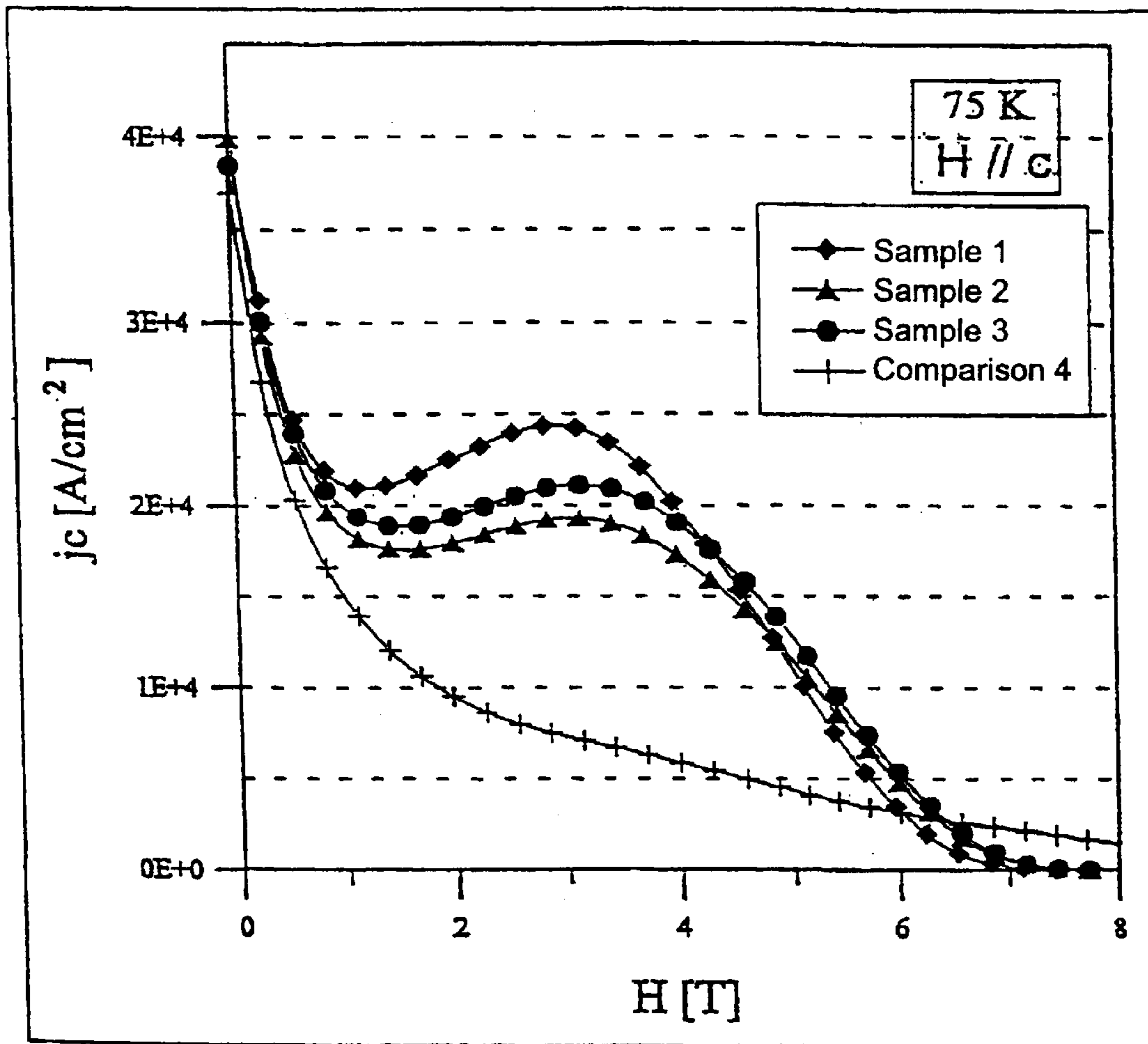
Critical Current Strength plotted vs. Field Strength
