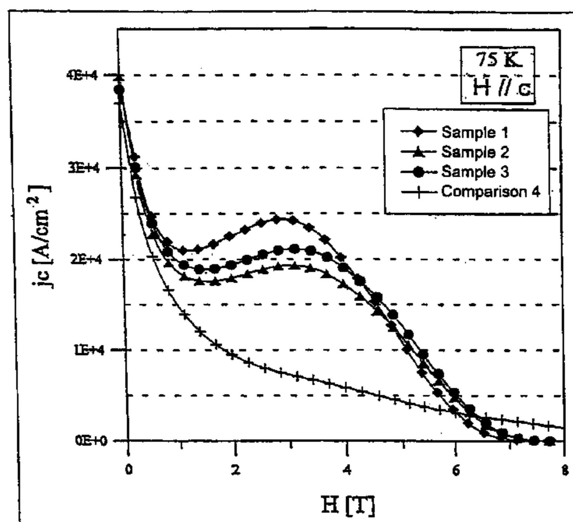
Critical Current Strength plotted vs. Field Strength
