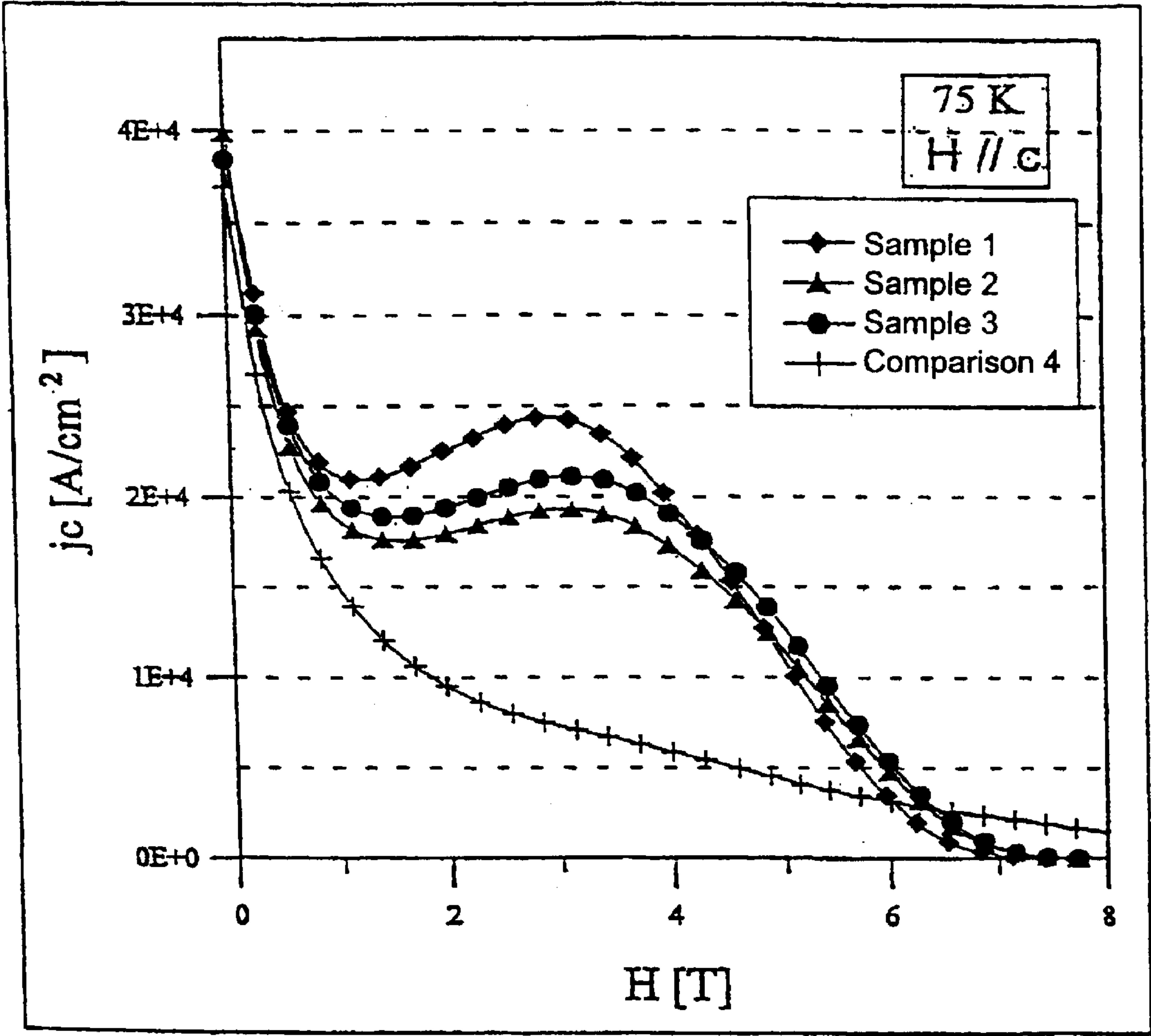
Critical Current Strength plotted vs. Field Strength
