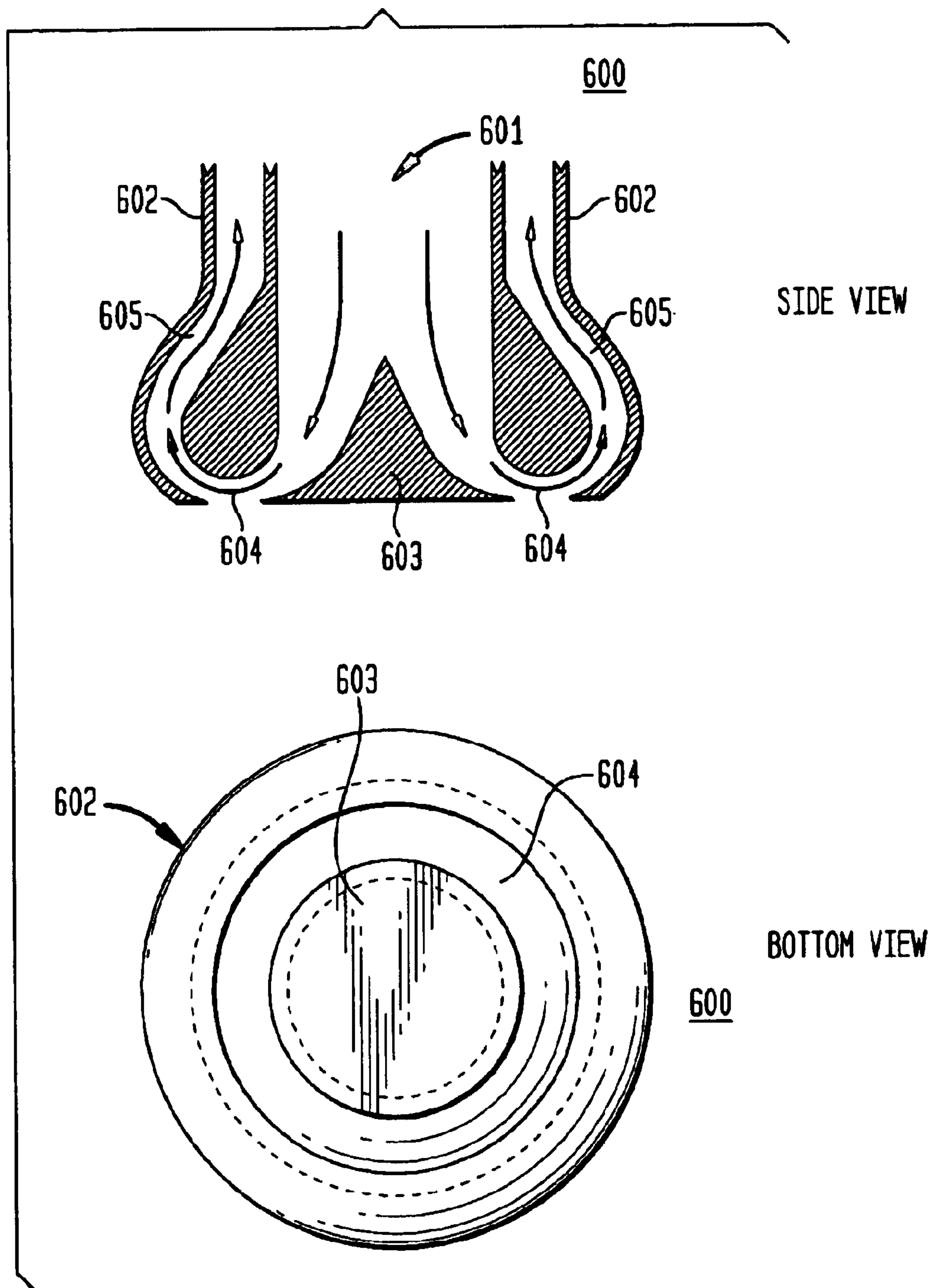
FIG. 6 (PRIOR ART)
