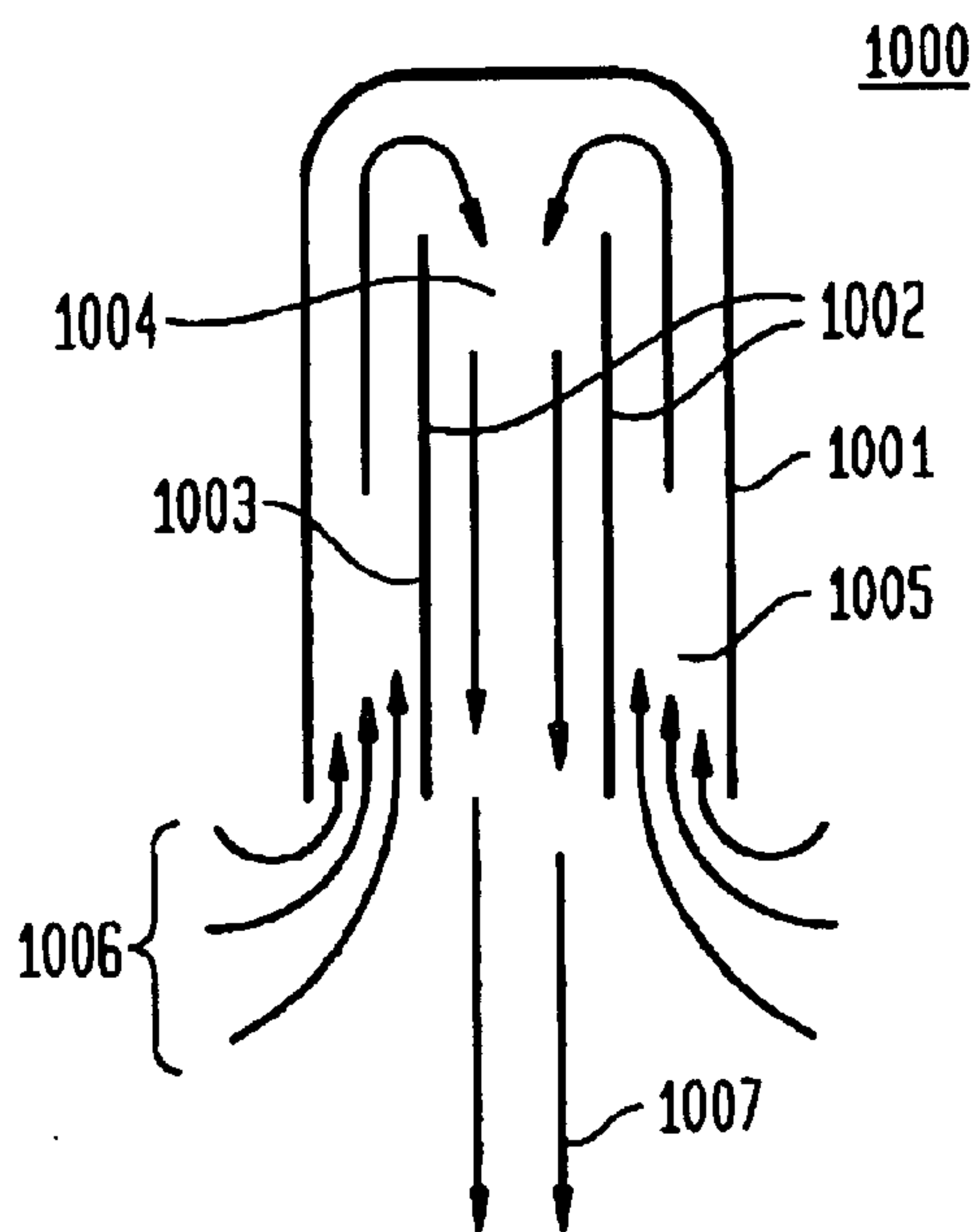
FIG. 10 (PRIOR ART)
