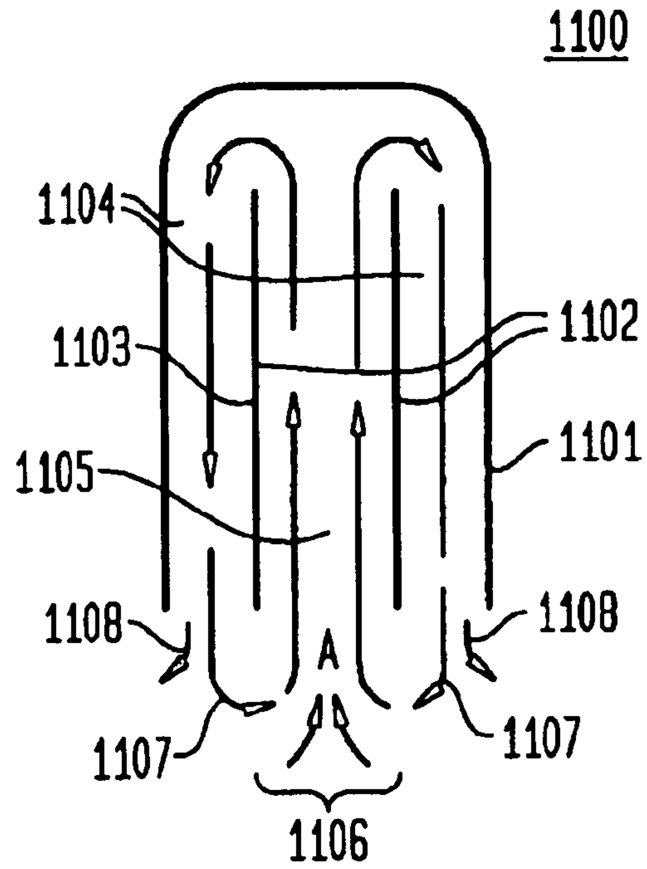
FIG. 11 (PRIOR ART)
