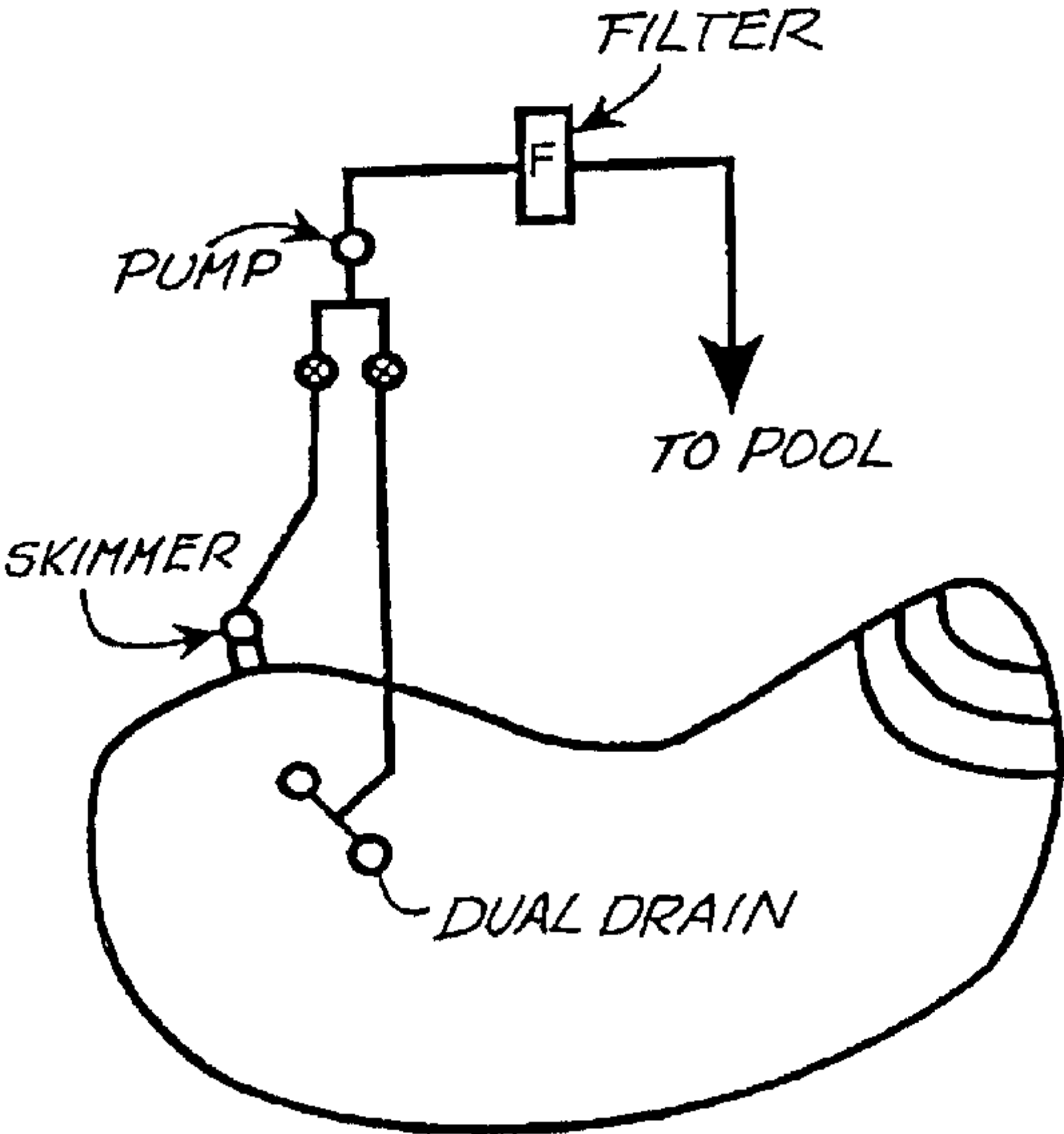
FIG. 12 (PRIOR ART)
