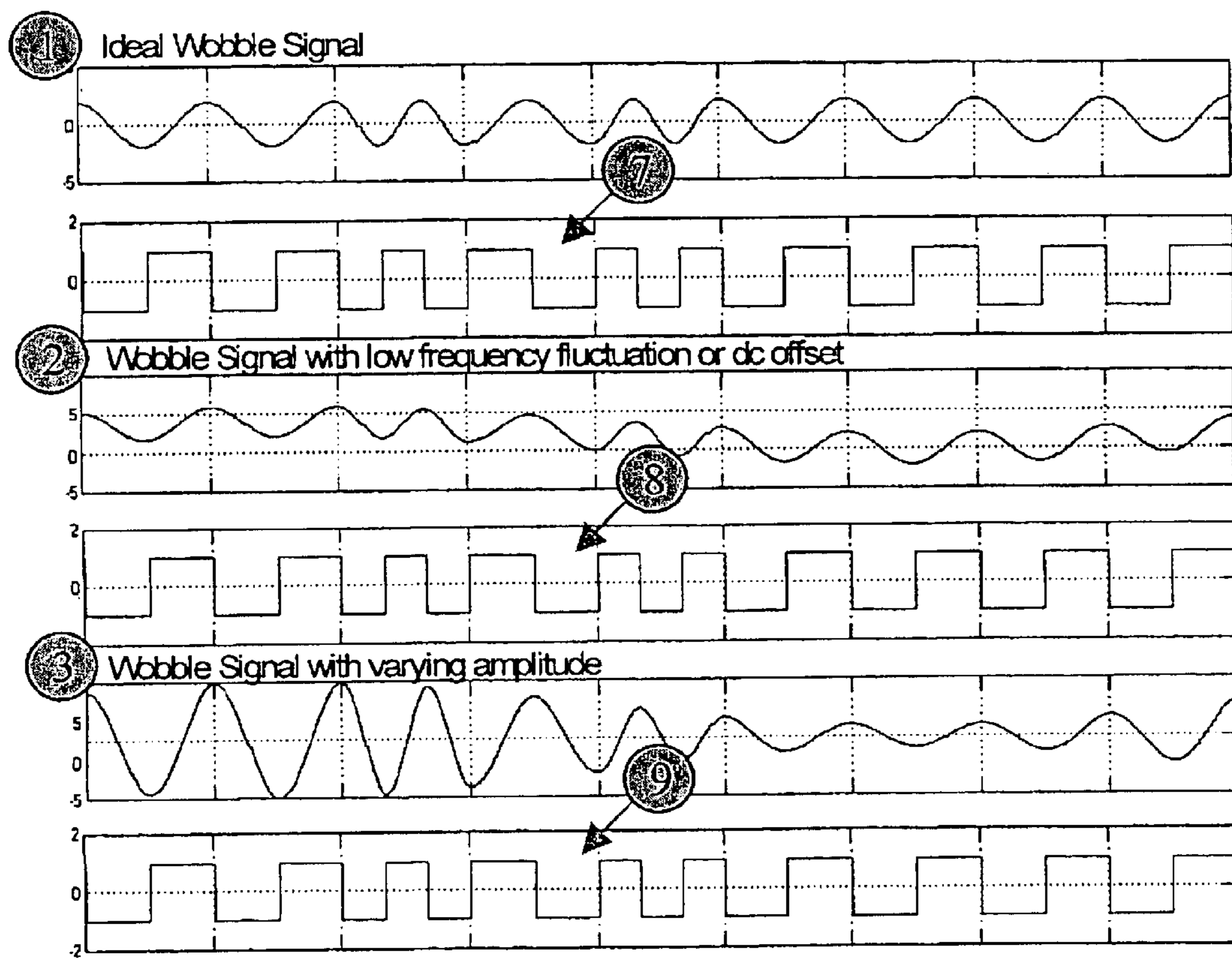
Peak Detected Wobble Signal
