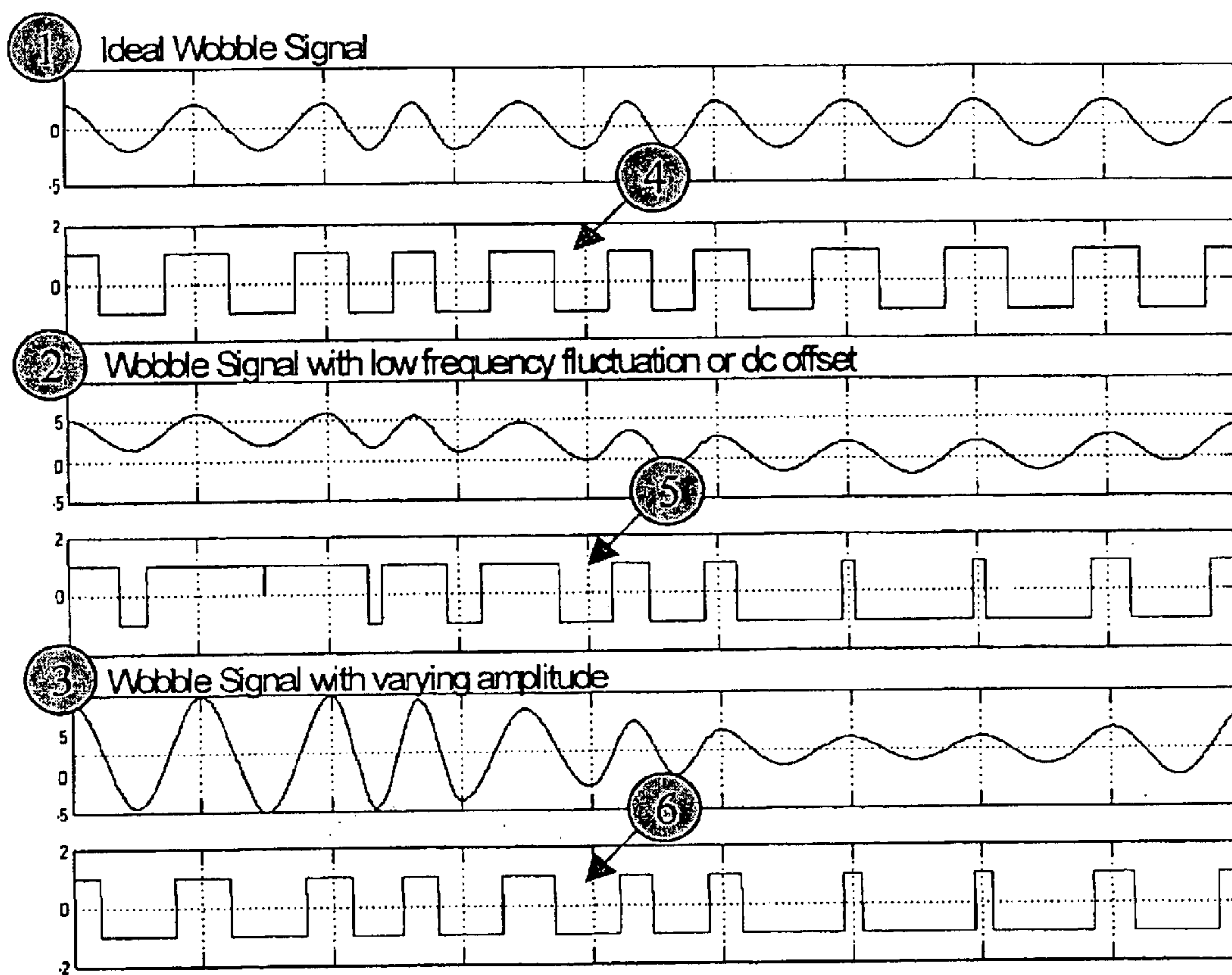
Wobble Signal Slicing Method
