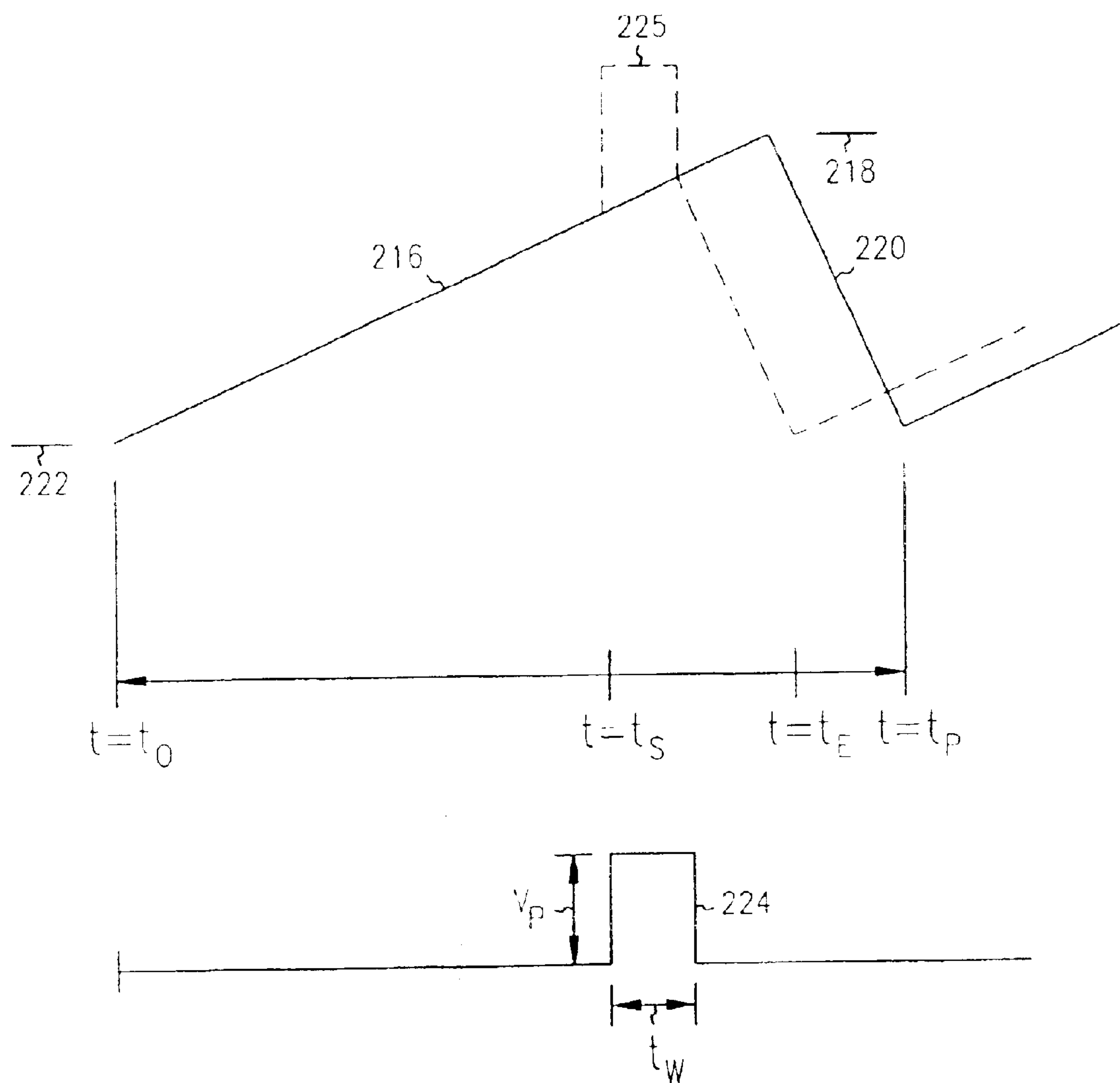
FIG. 2 (PRIOR ART)
