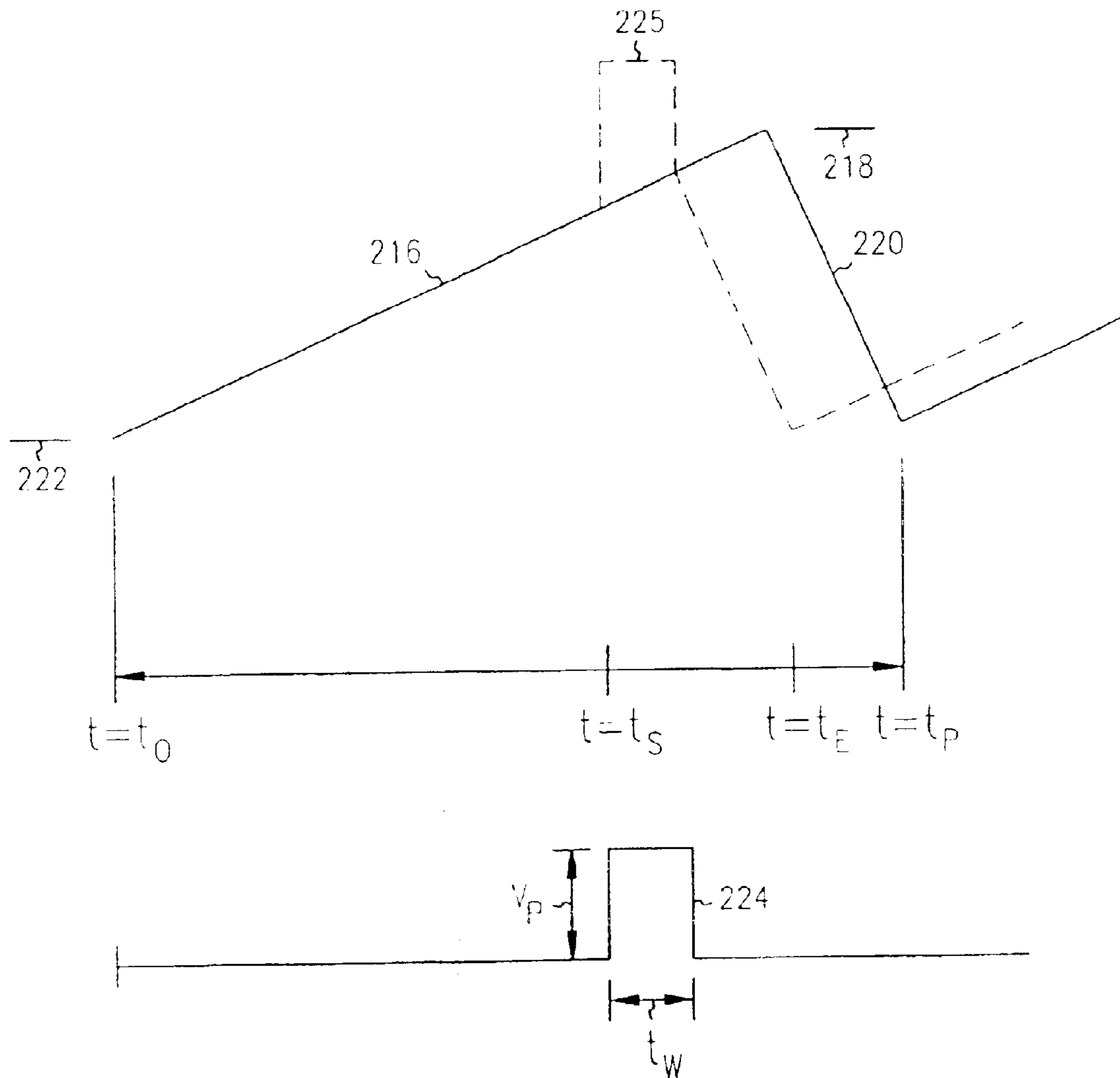
FIG. 2 (PRIOR ART)
