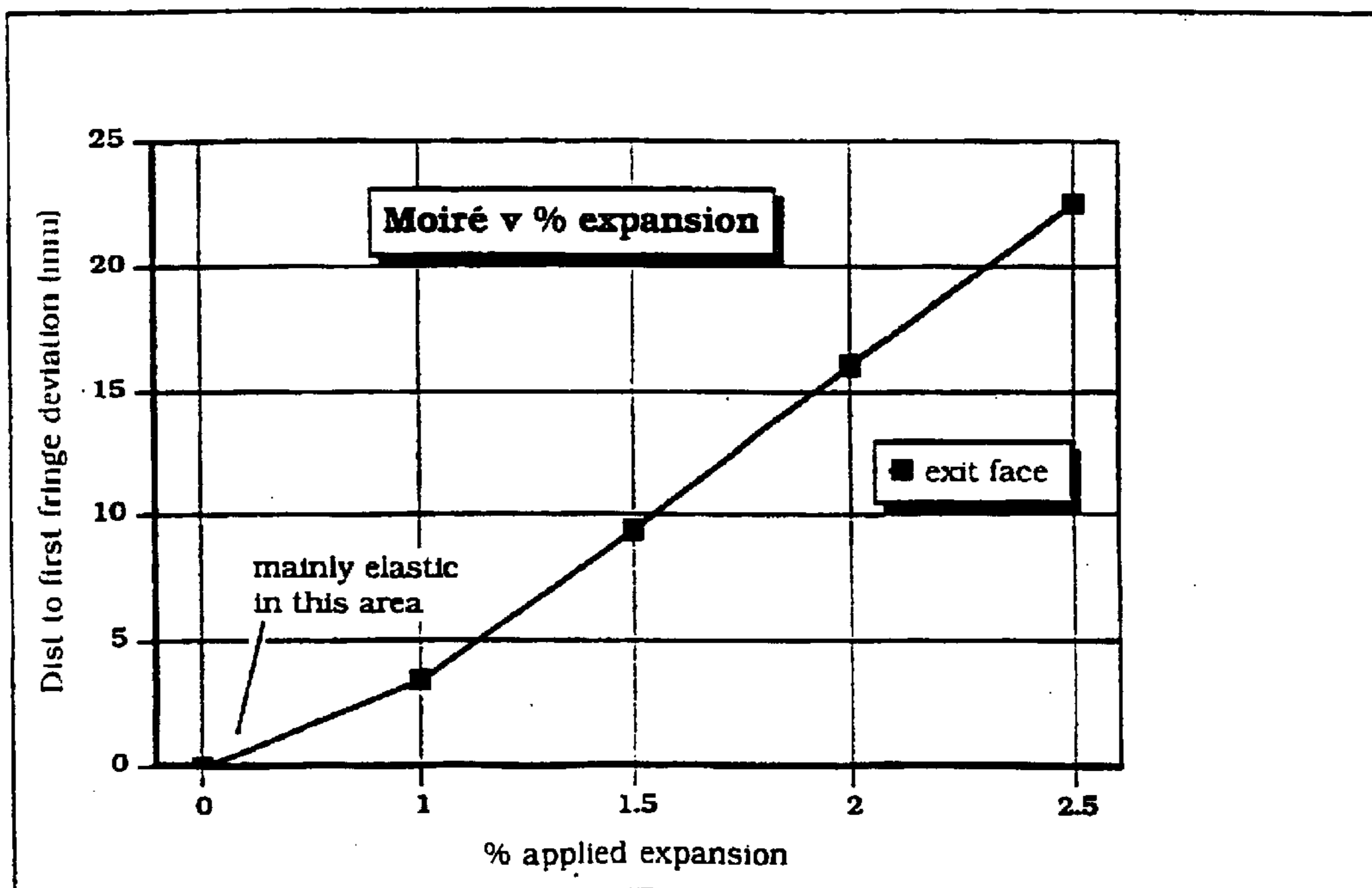
Fig. 5 b. Graph of extent of Poissons effect versus degree of applied expansion - exit face.
