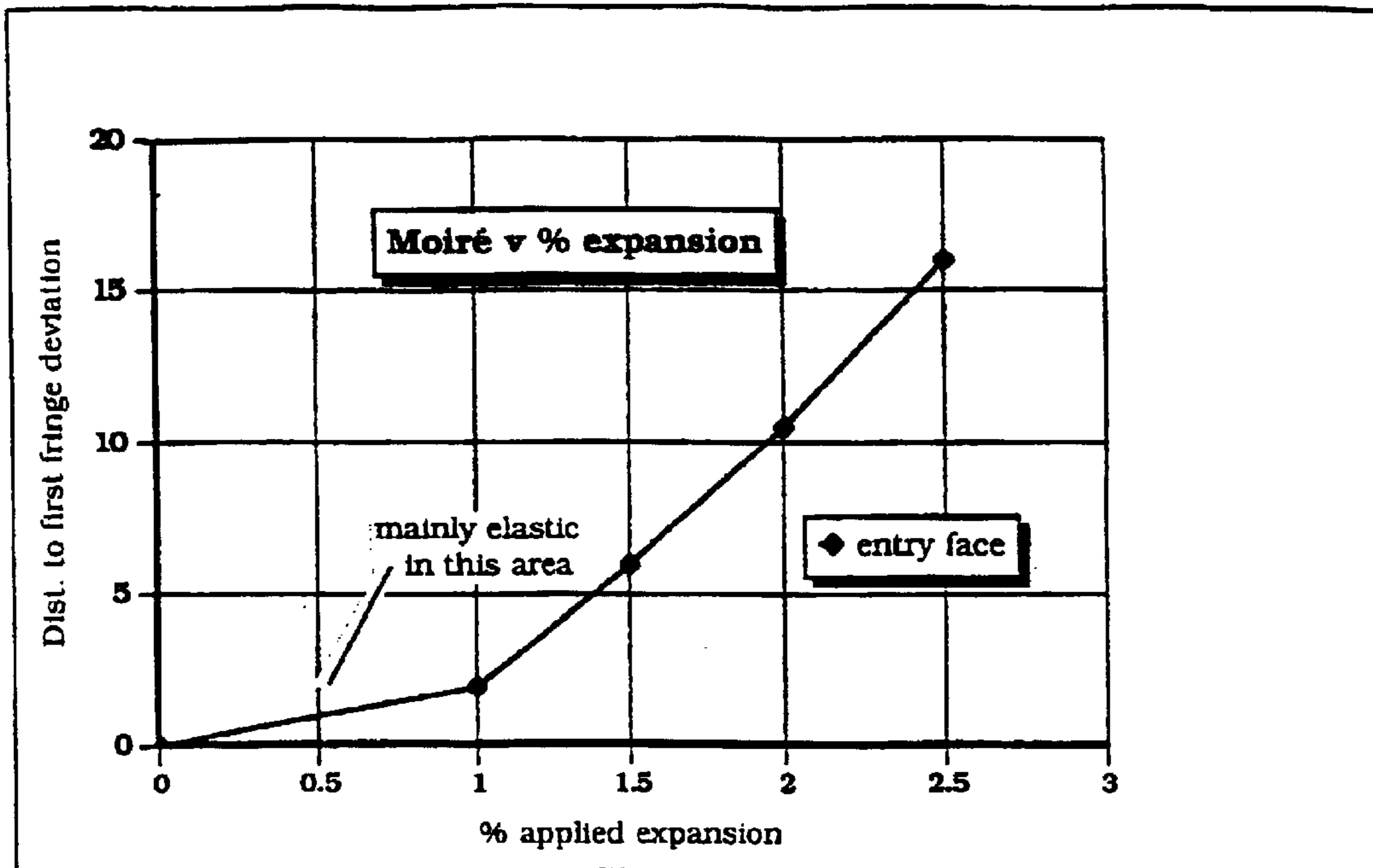
Fig. 5 a. Graph of extent of Poissons effect versus degree of applied expansion - entry face.
