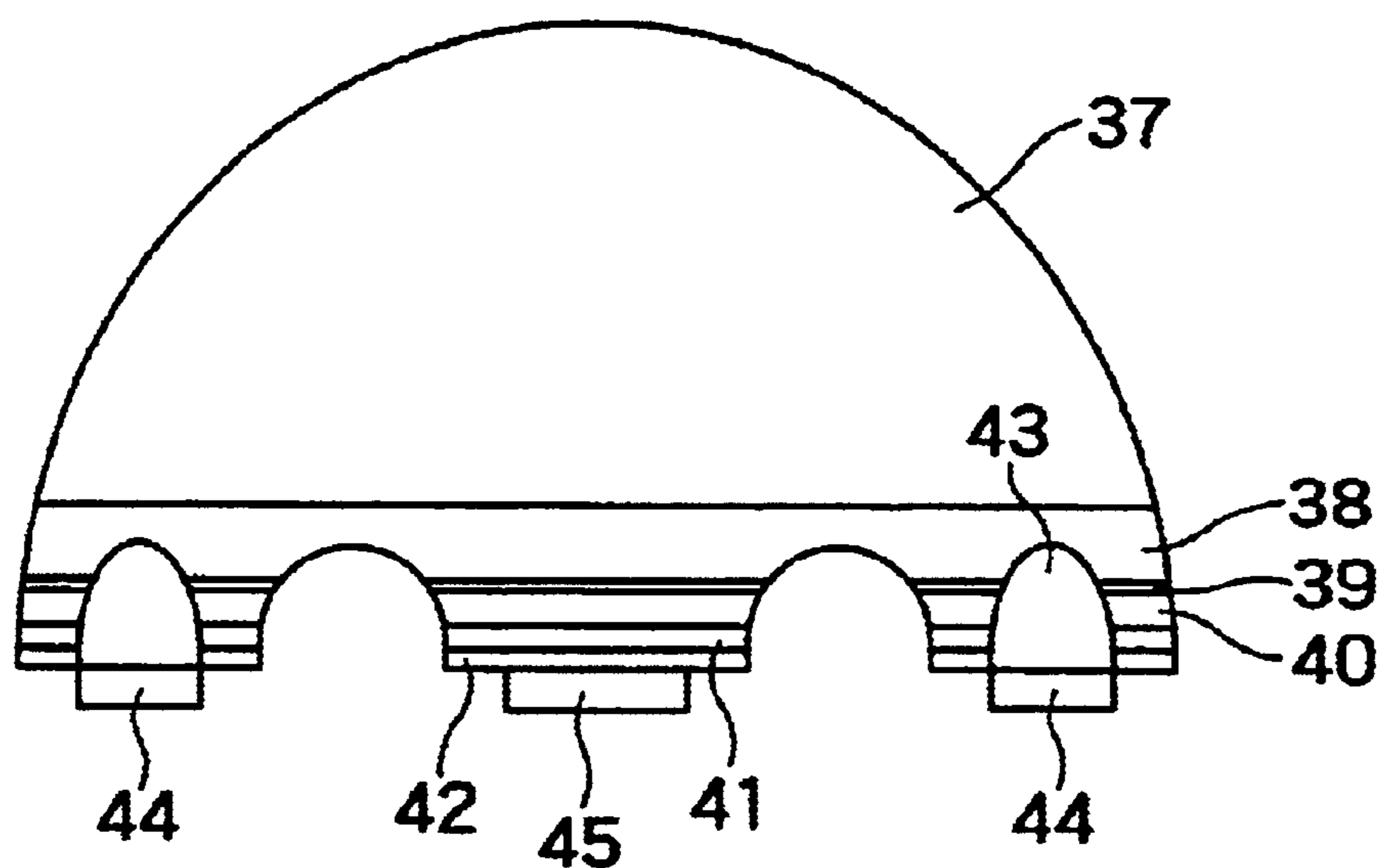
FIG. 21 PRIOR ART
