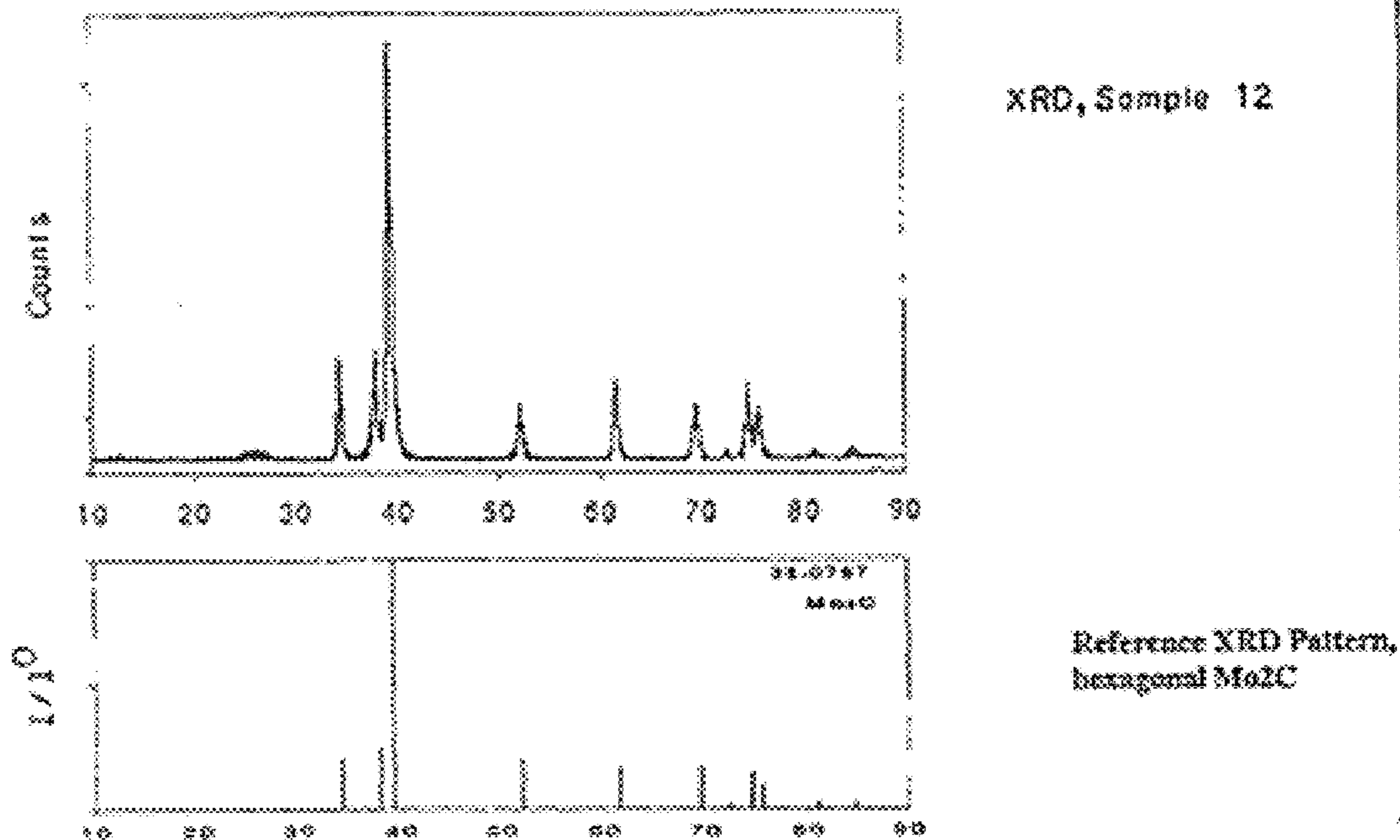
FIG. 1A XRD and SEM of CARBIDE NANORODS
