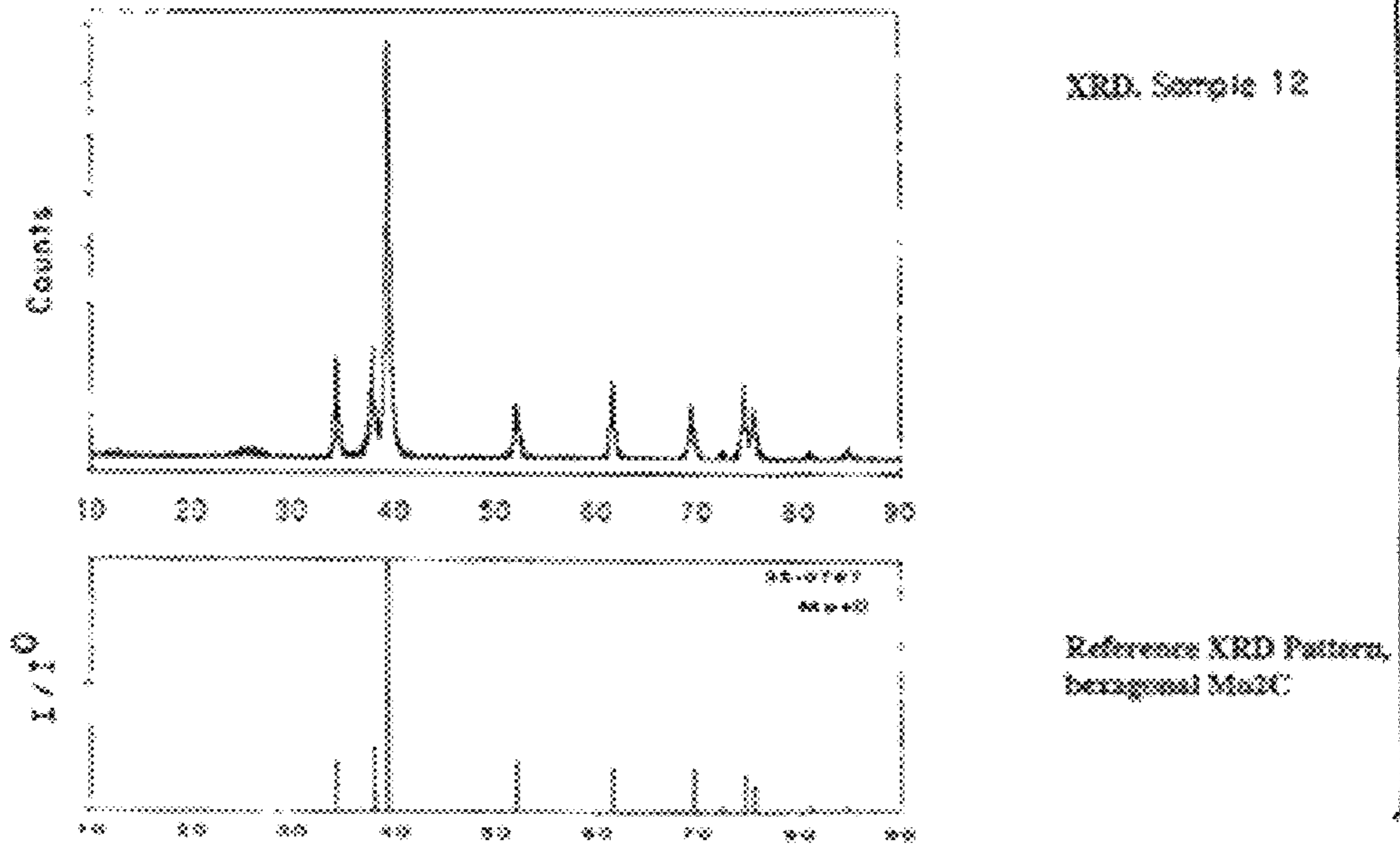
FIG.2A XRD and HRTEM of CARBIDE NANORODS
