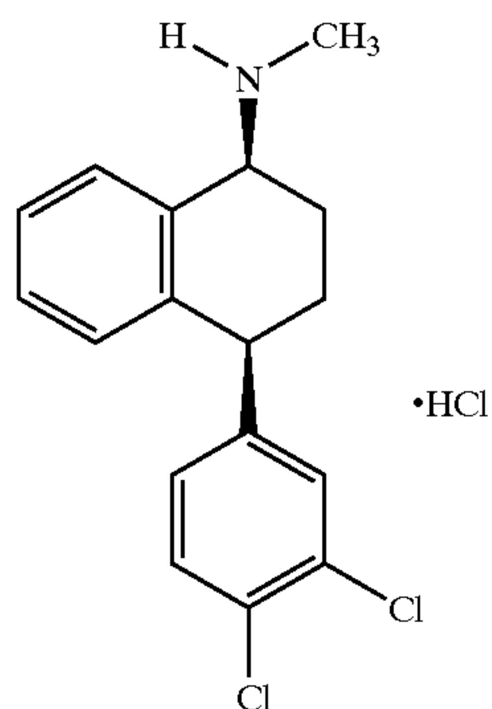
Sertraline hydrochloride
