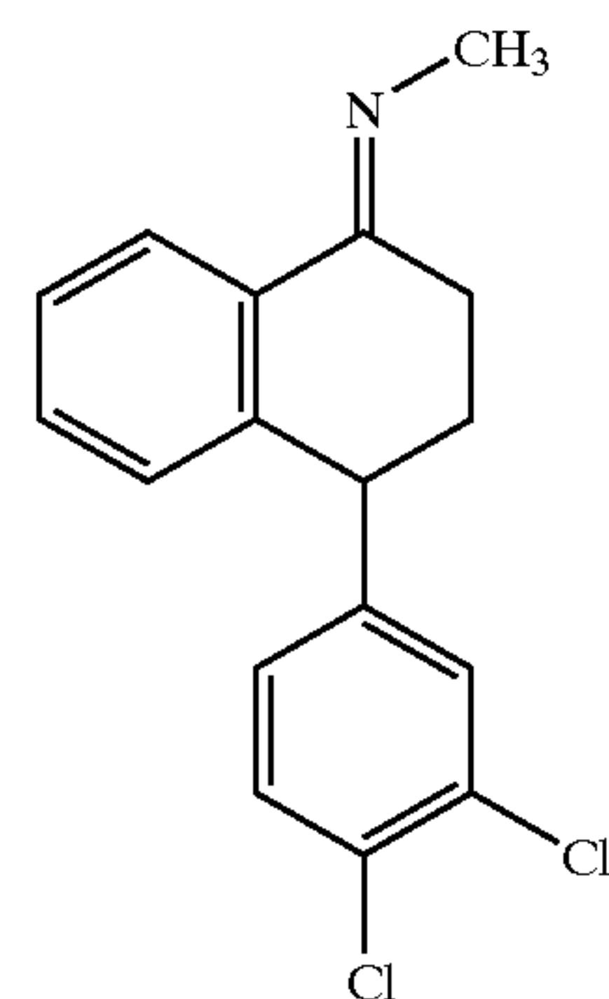
Sertraline 1-imine
