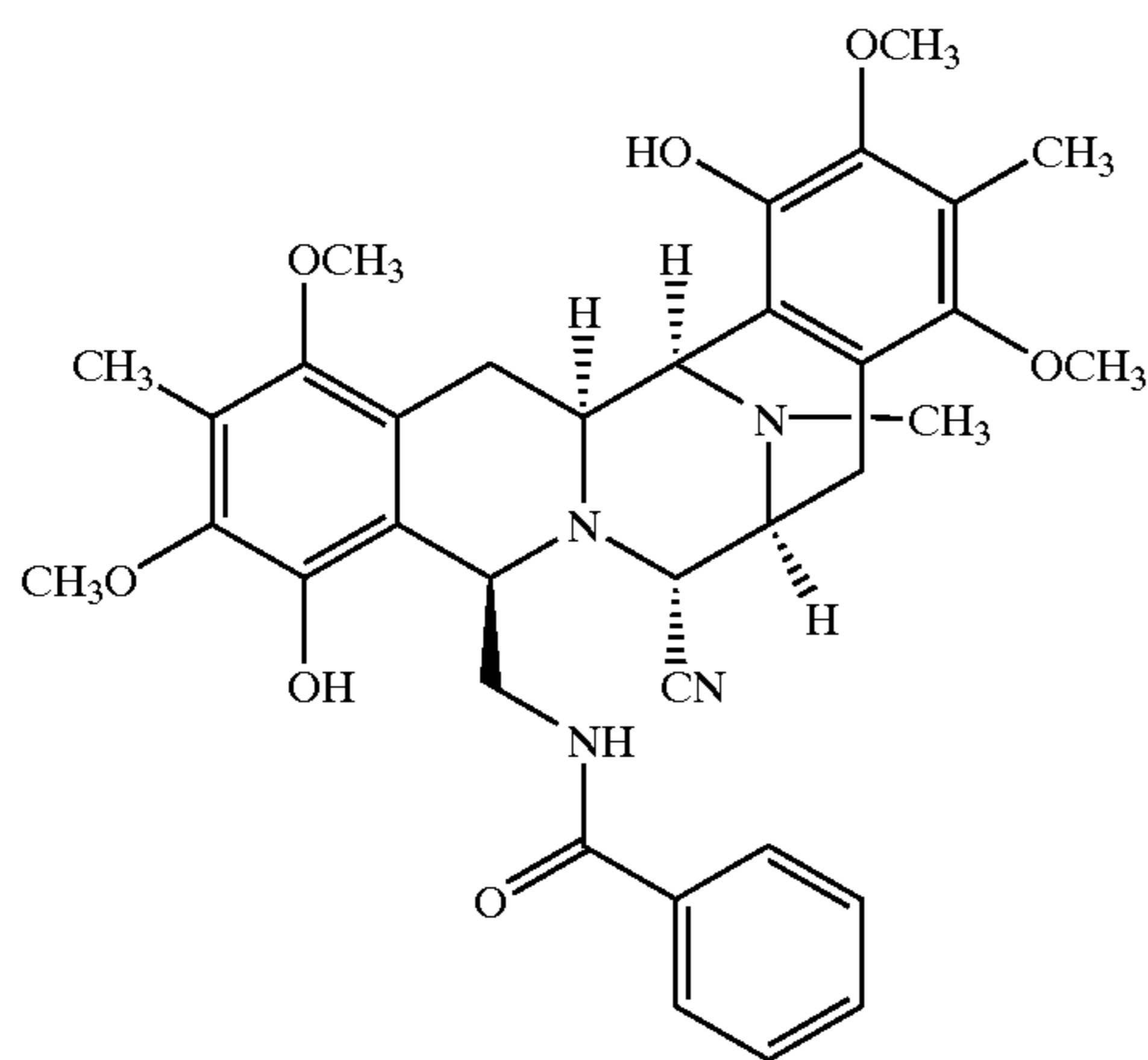
Benzamide Derivative
