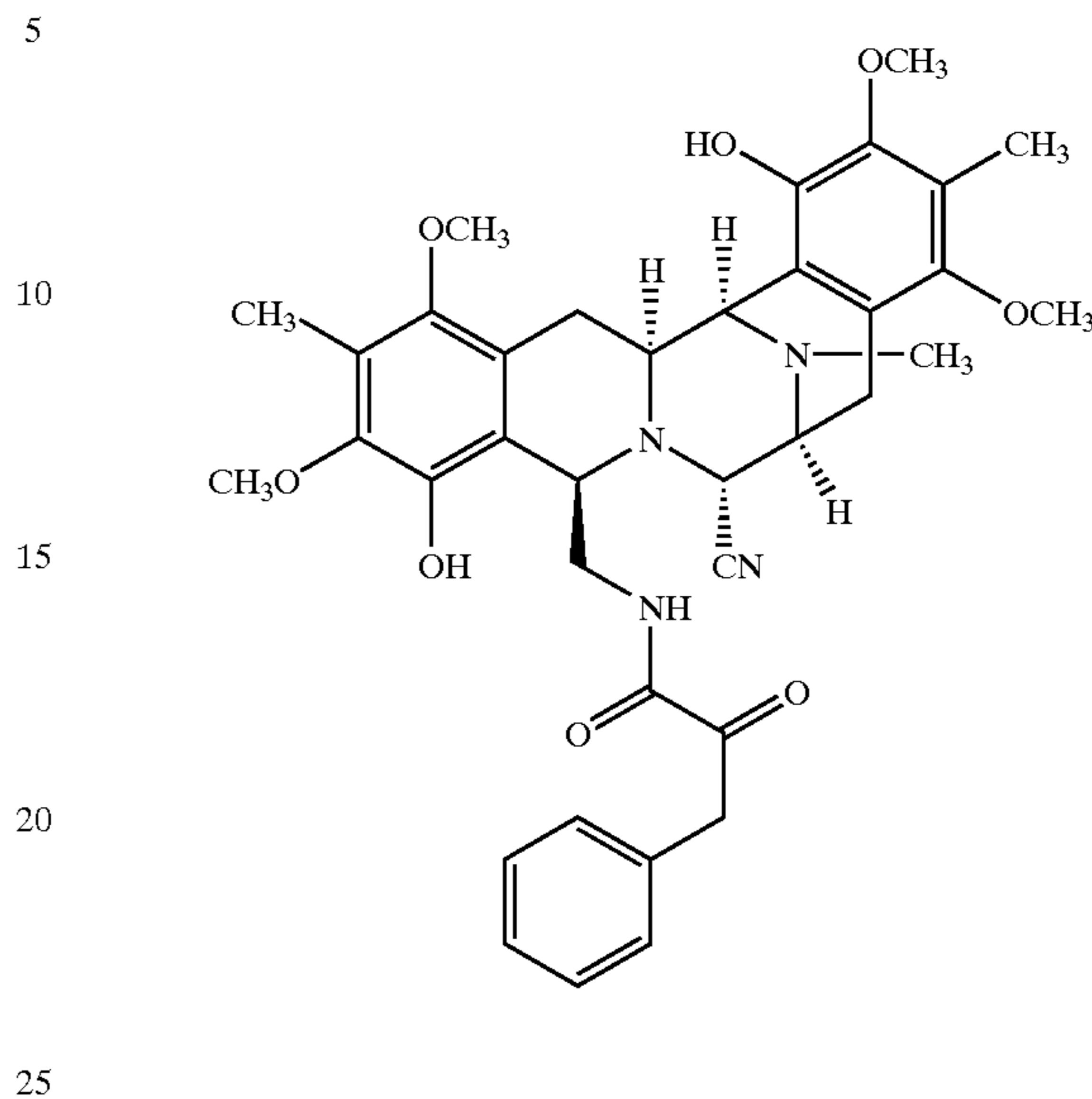
Phenylpyruvamide Derivative
