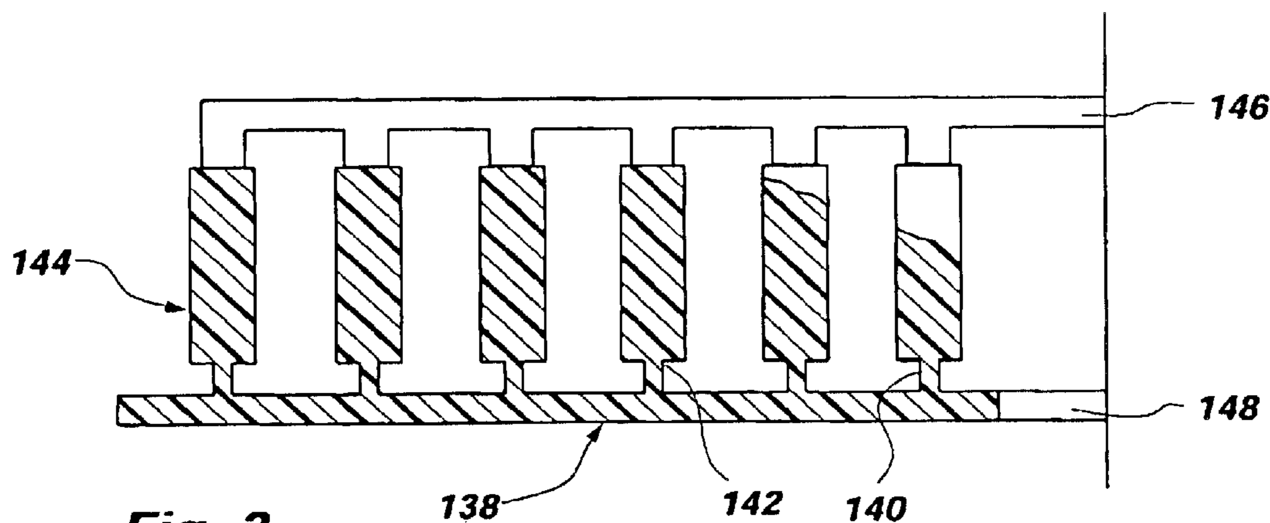
Fig. 3 (PRIOR ART)
