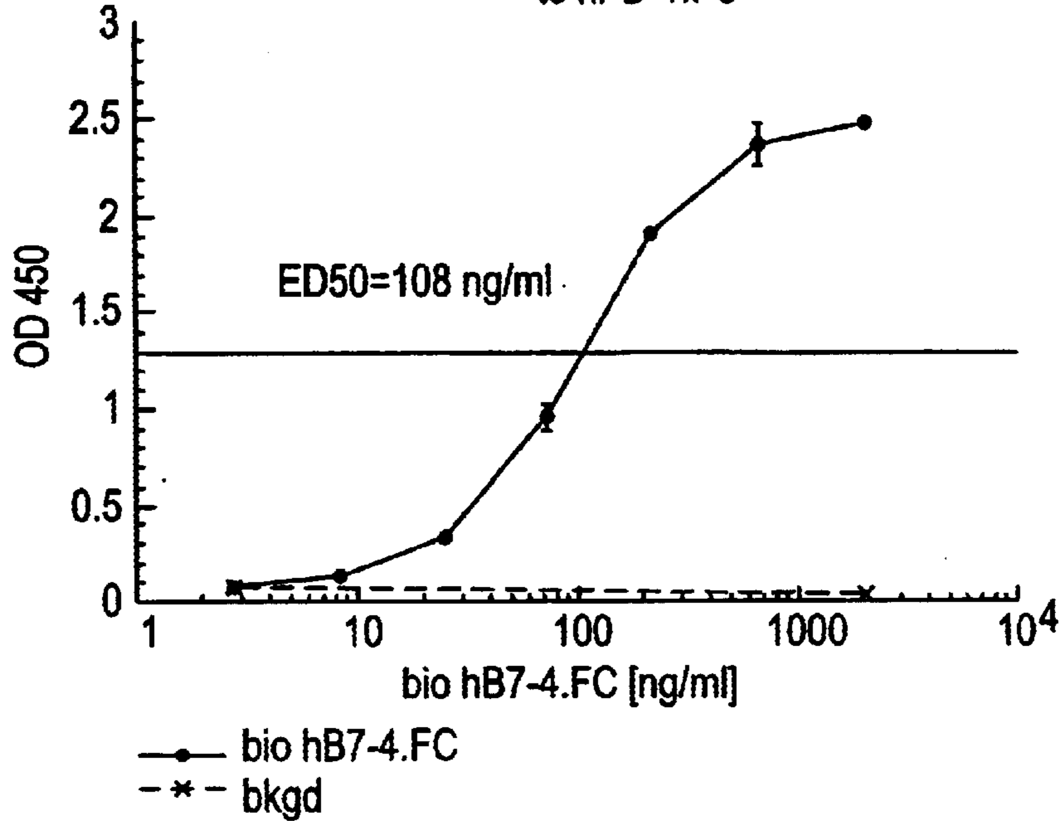
KM89 Binding curve of bio hB7-4.FC (TV2001) to hPD-1.FC
