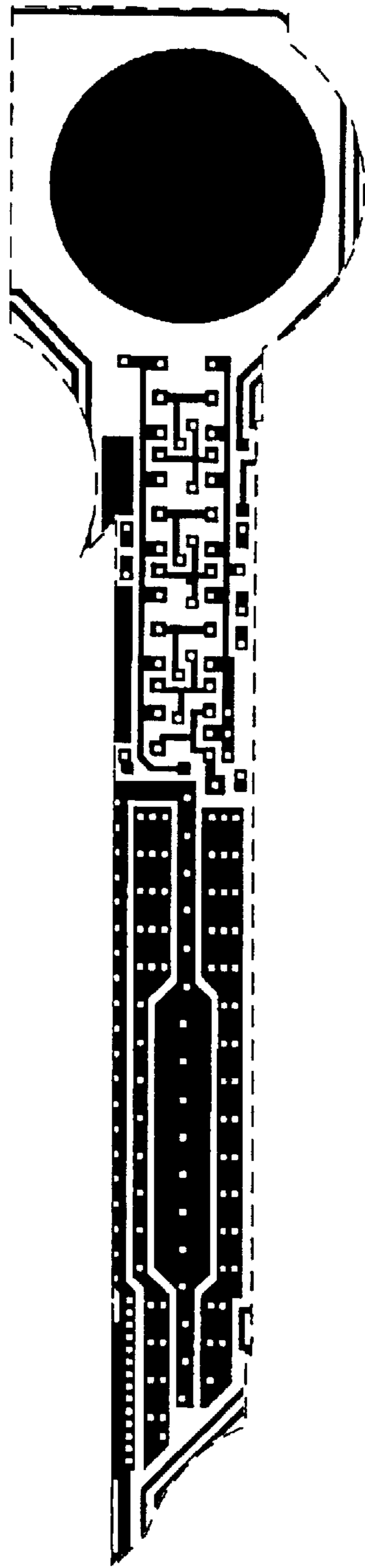
Metal 1 mask
