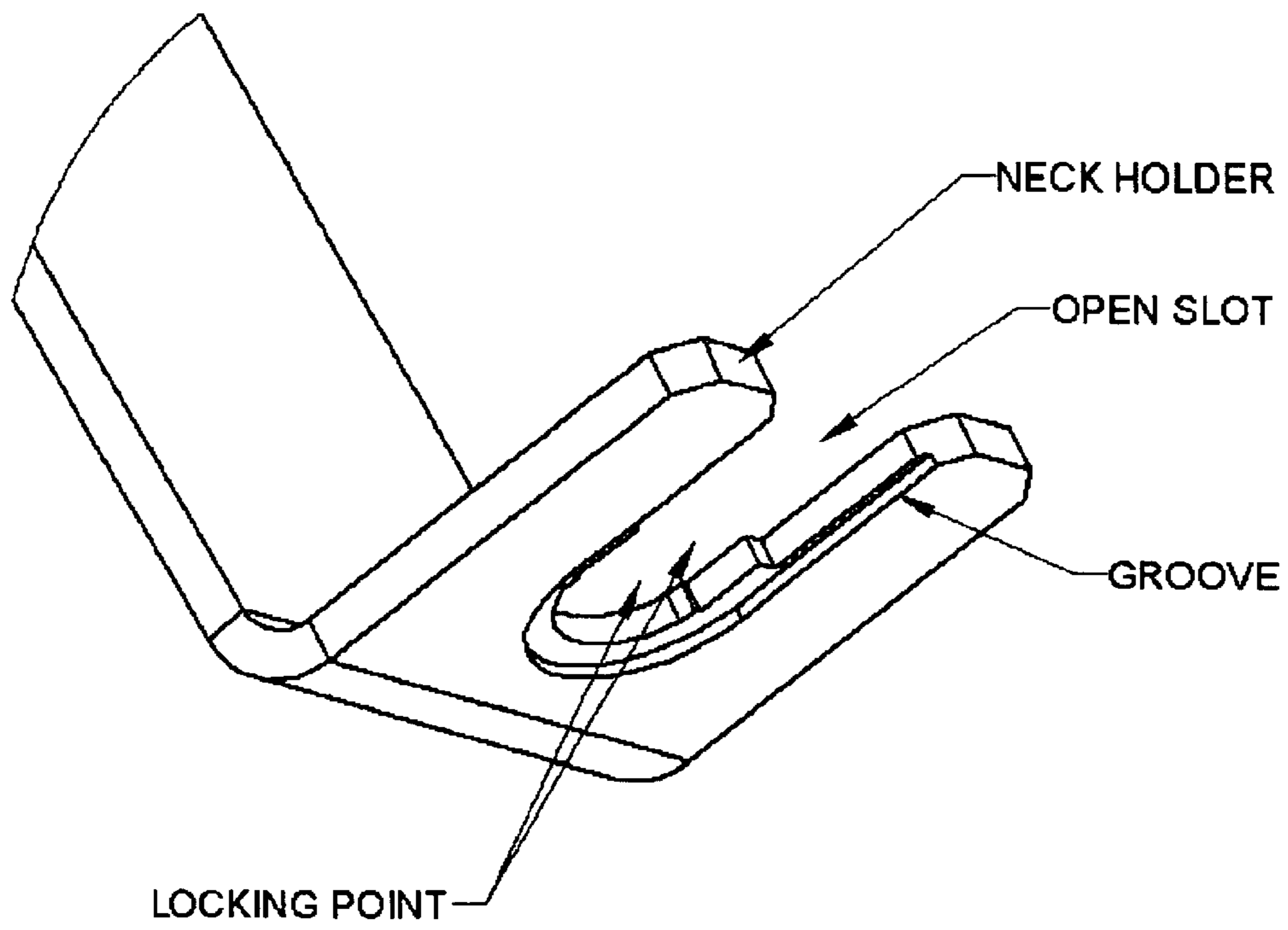
Fig. 10 Neck holder with a groove to hold different size bottles
