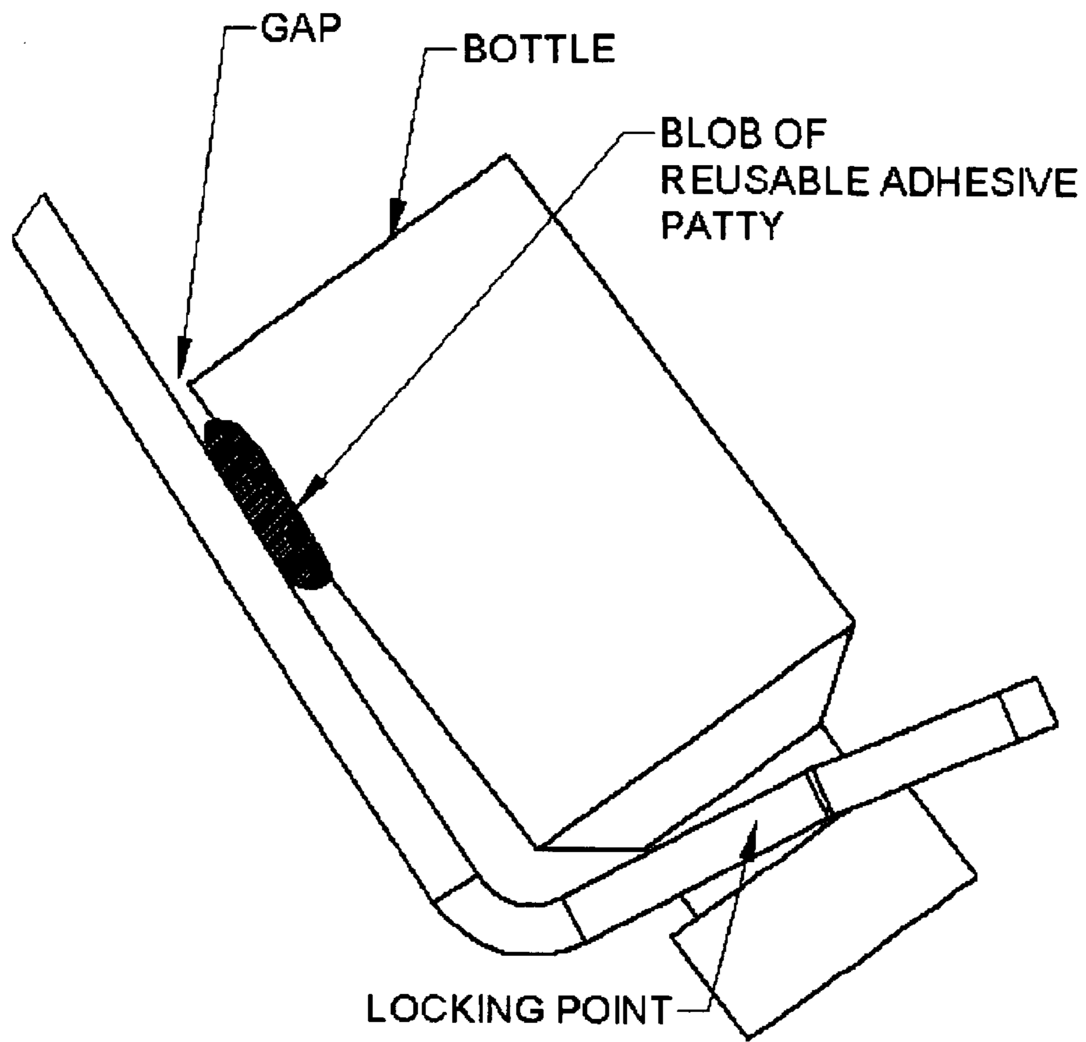
FIG. 8 Fastening device using a blob of reusable adhesive patty.
