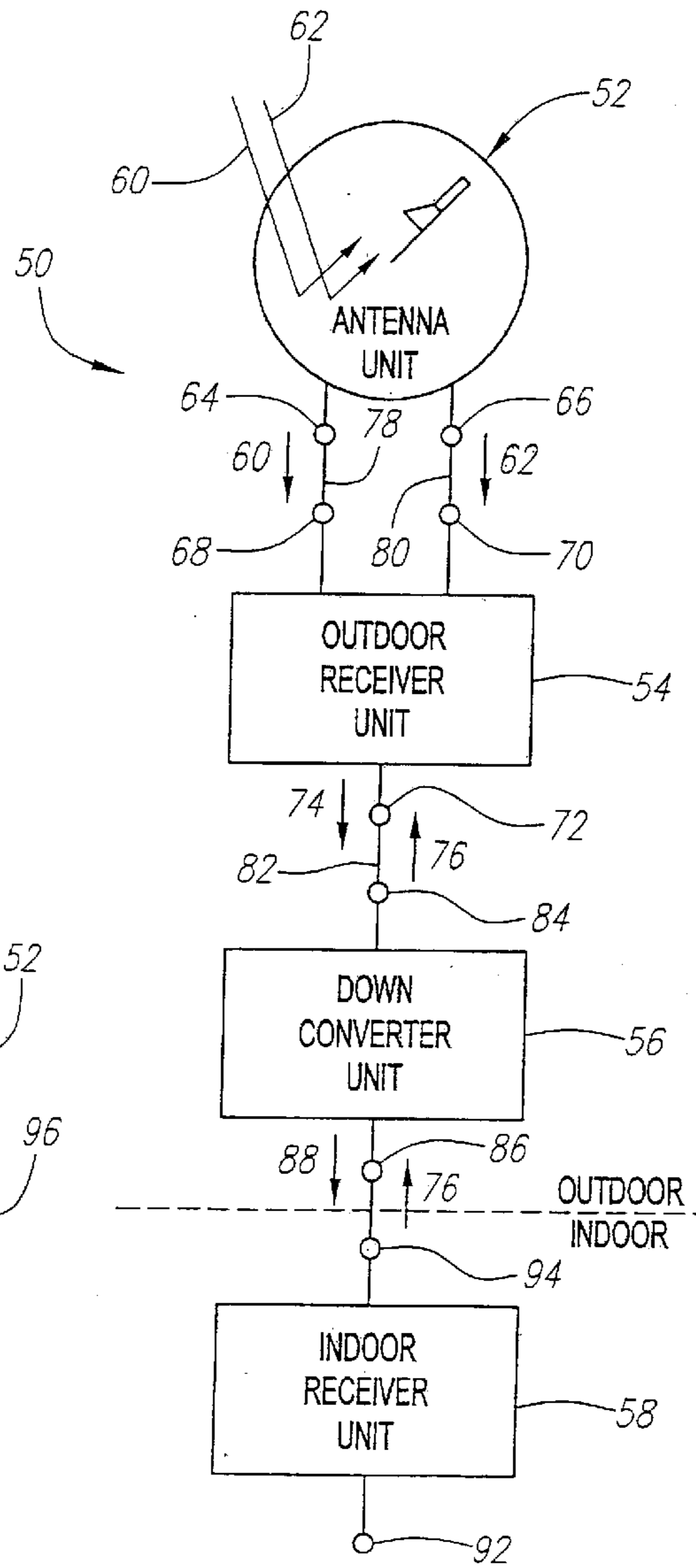
FIG. 1 (PRIOR ART)
