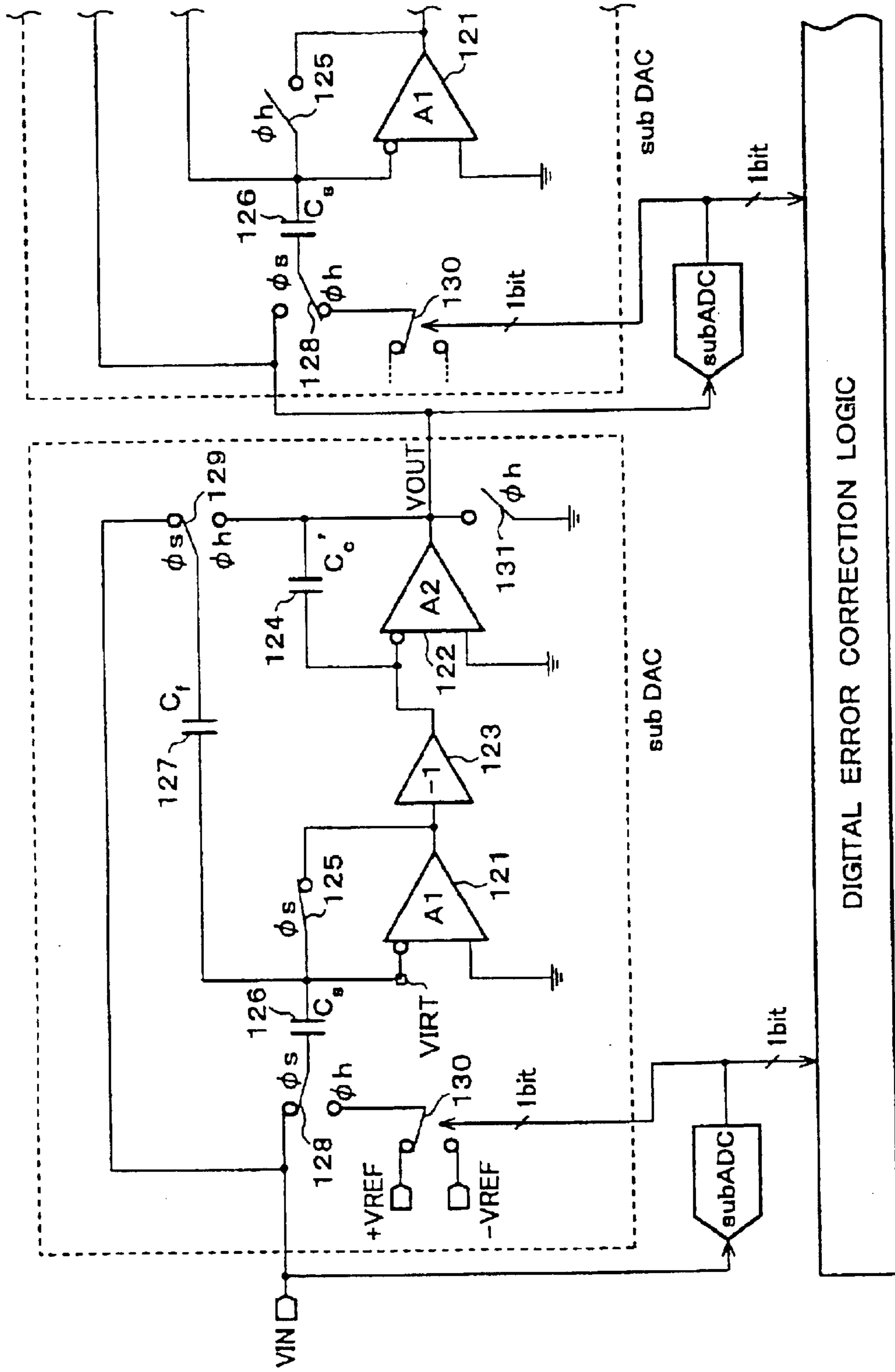
FIG. 15 PRIOR ART
