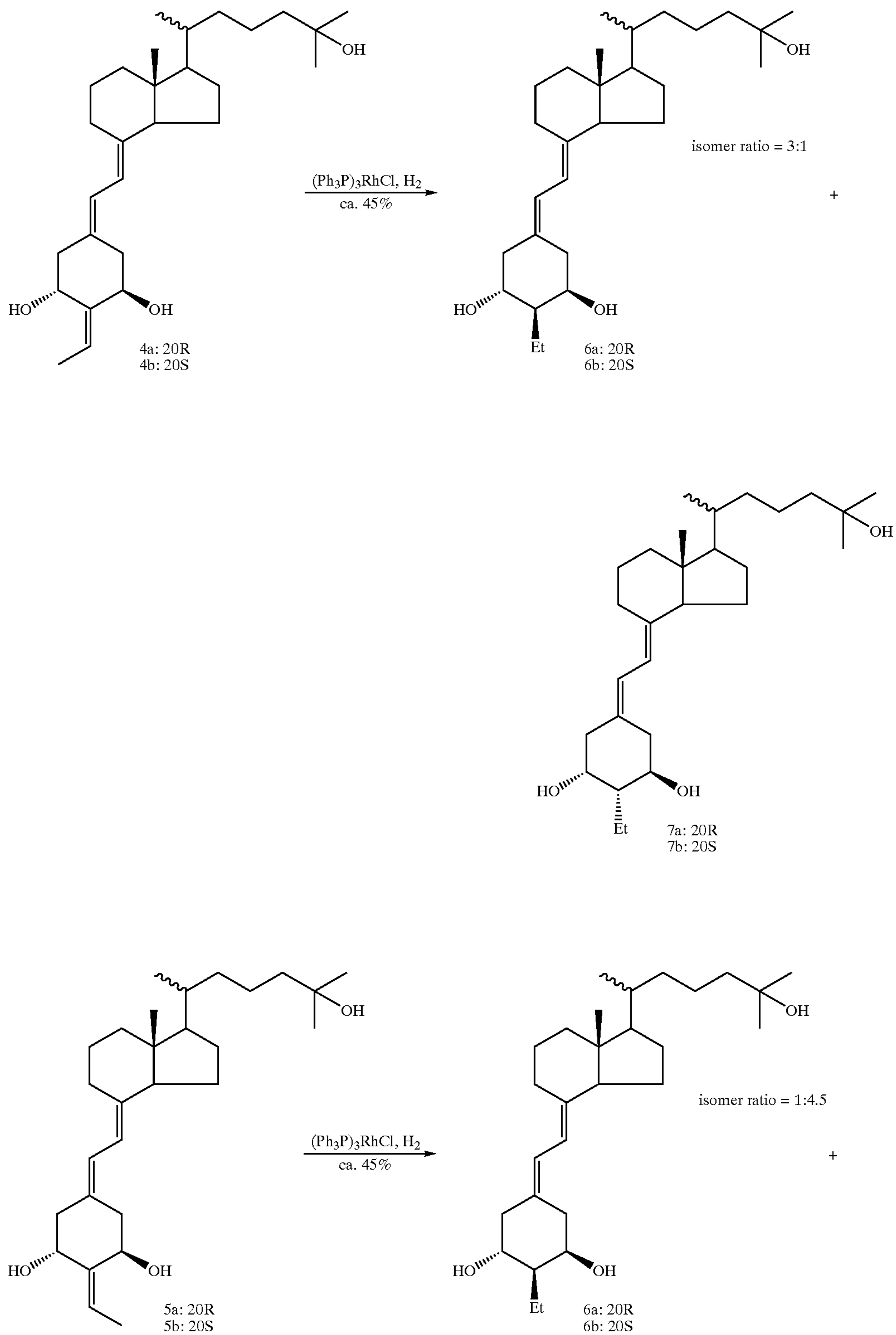
Scheme 6
