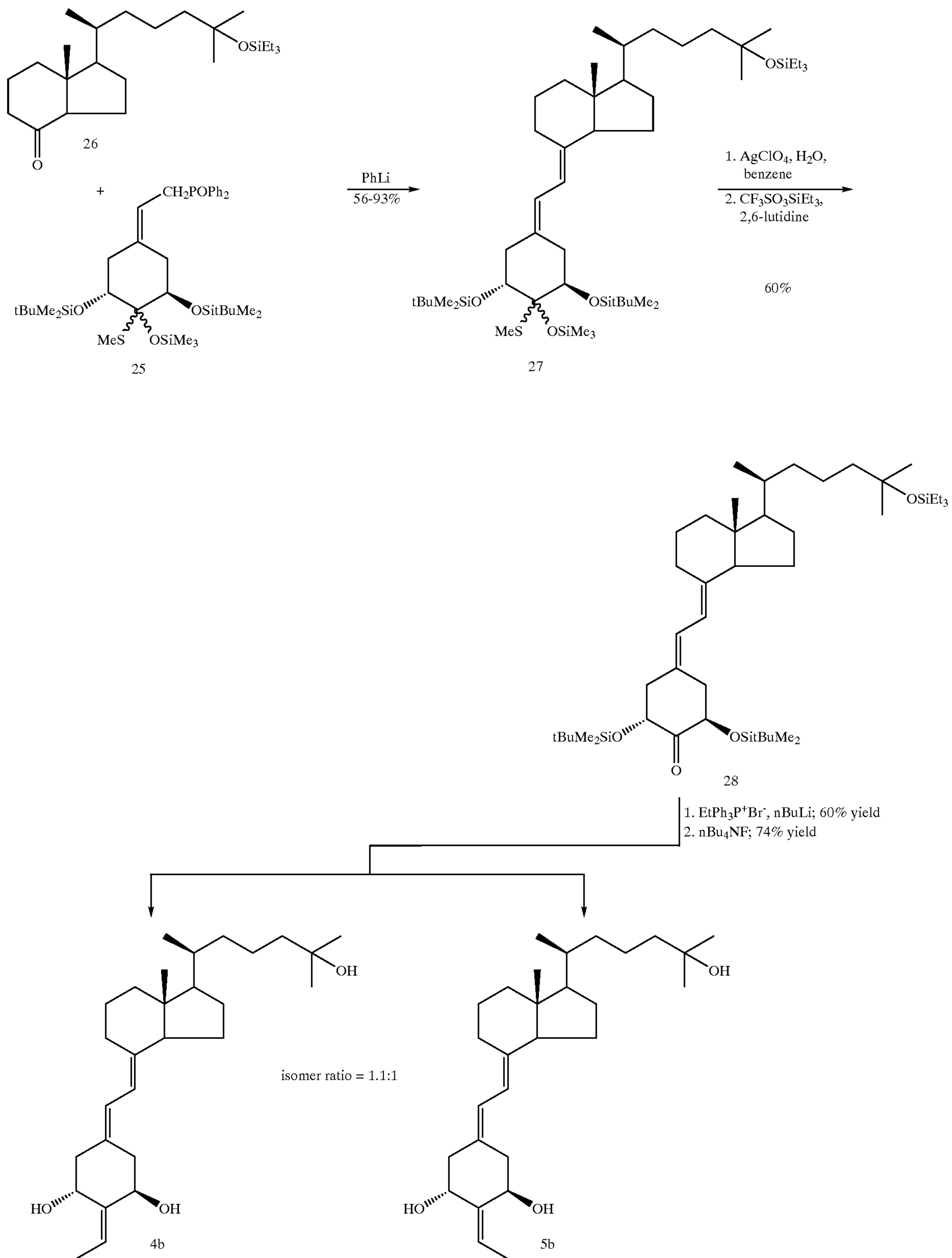
Scheme 5
