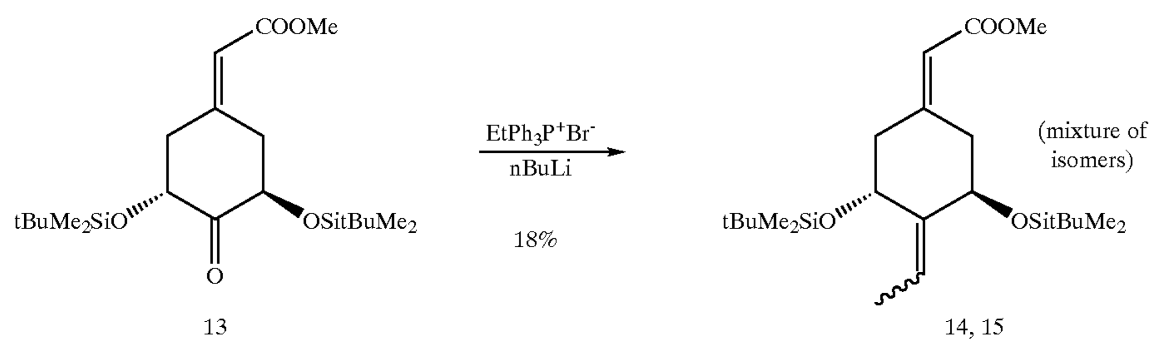
Scheme 2
