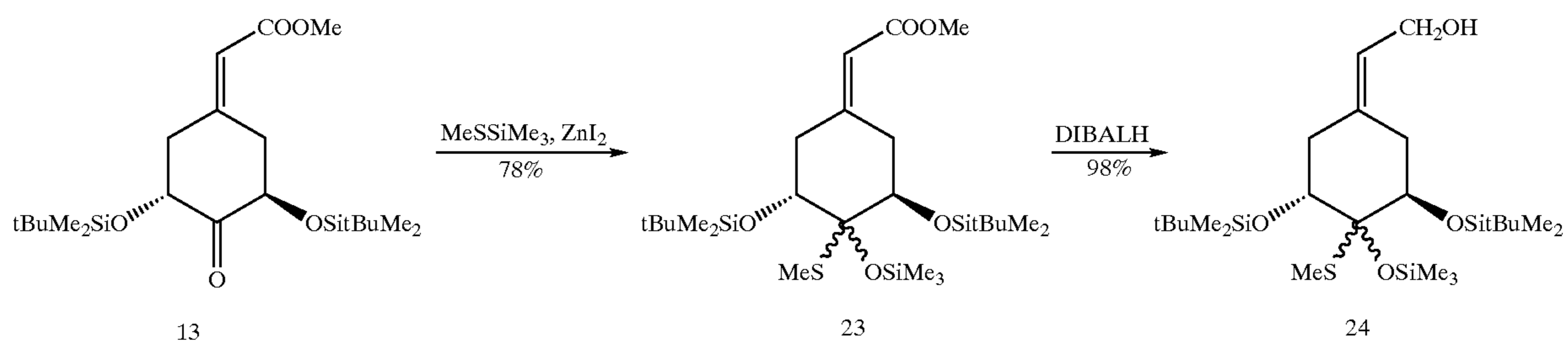
Scheme 4
