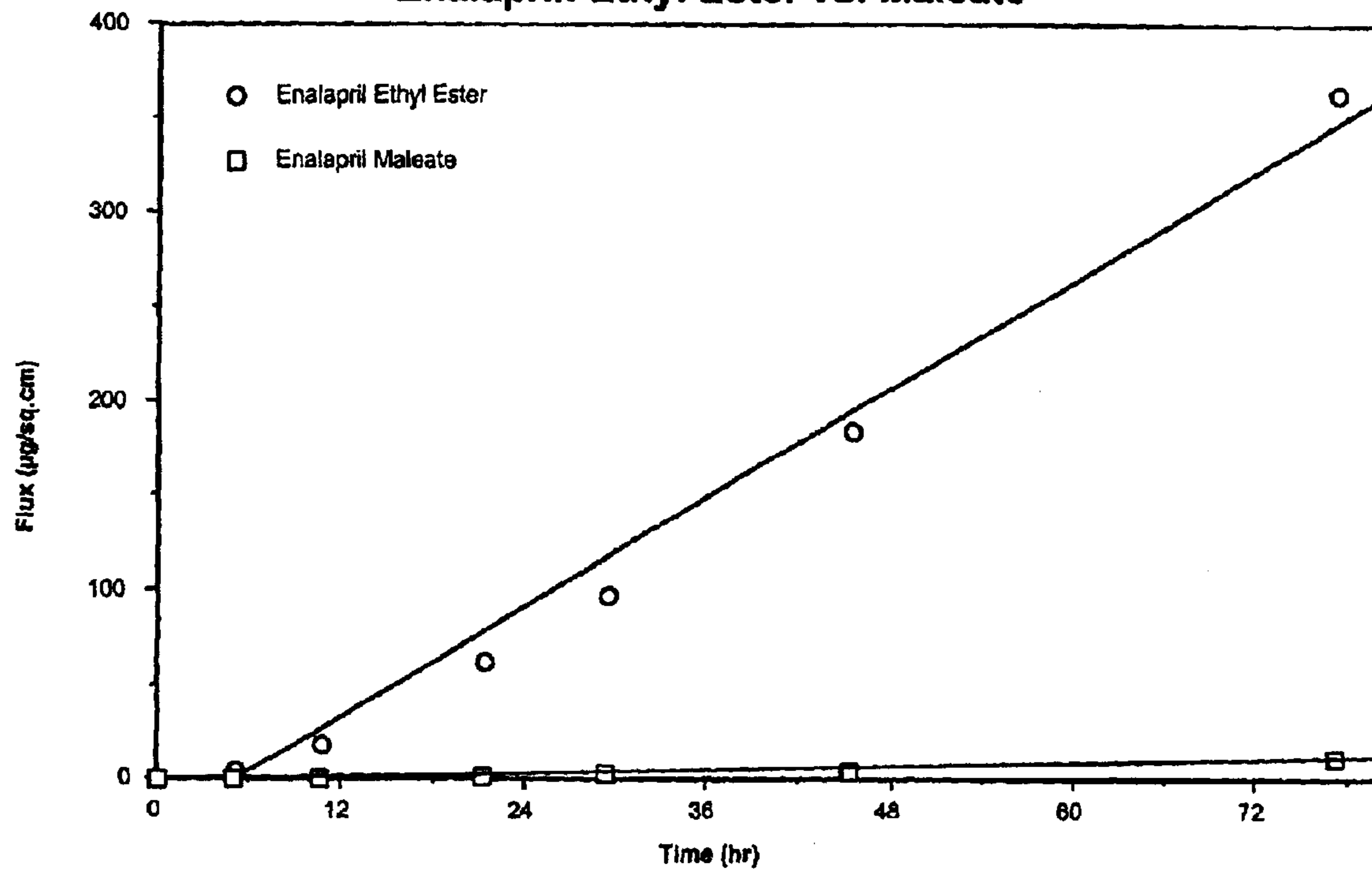
Figure 1 Enalapril: Ethyl Ester vs. Maleate
