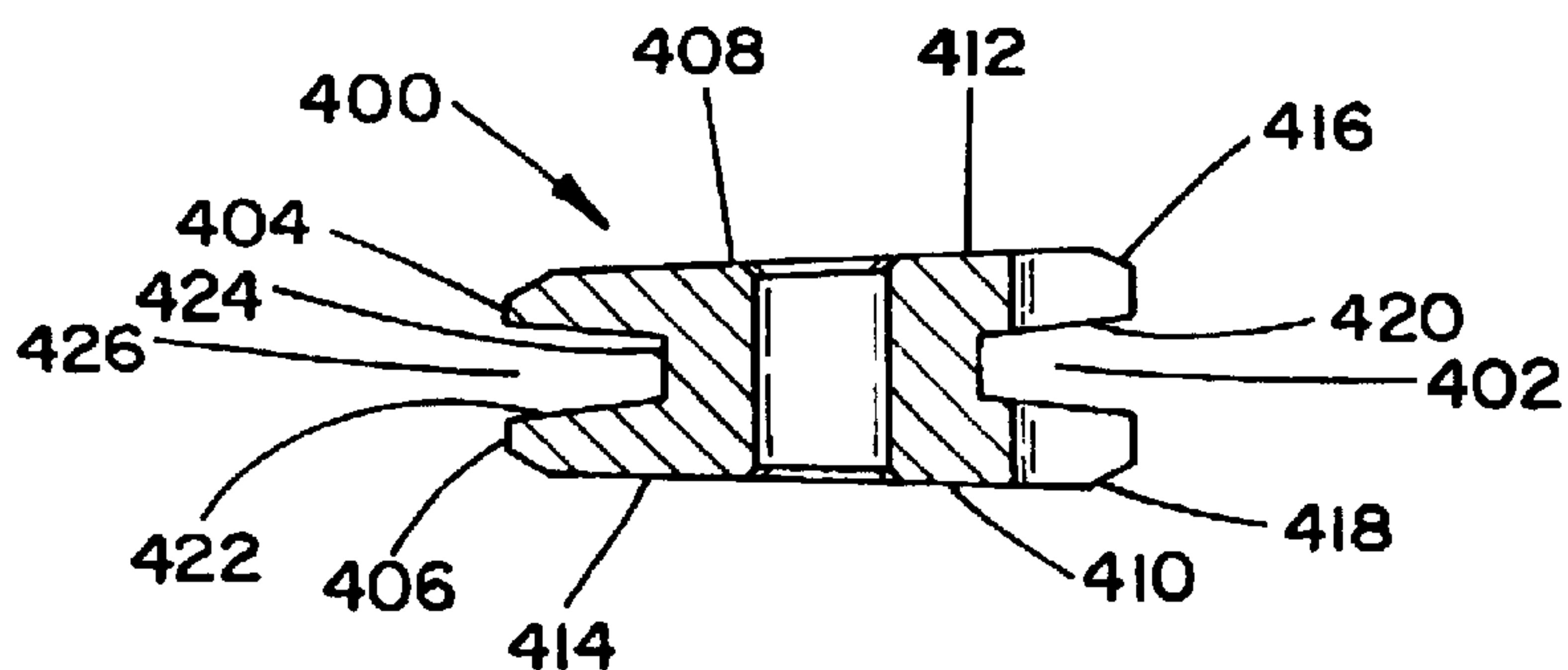
FIG. 4c Section 1-1 of FIG. 4a
