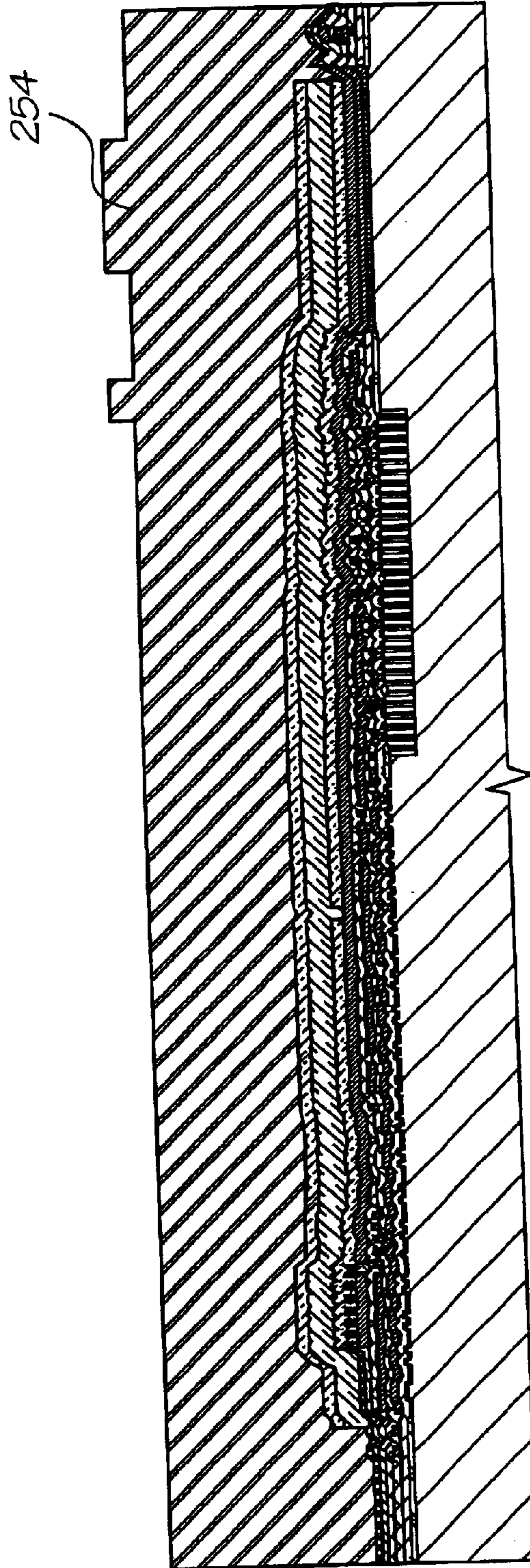
Deposit sacrificial layer, etch nozzles
