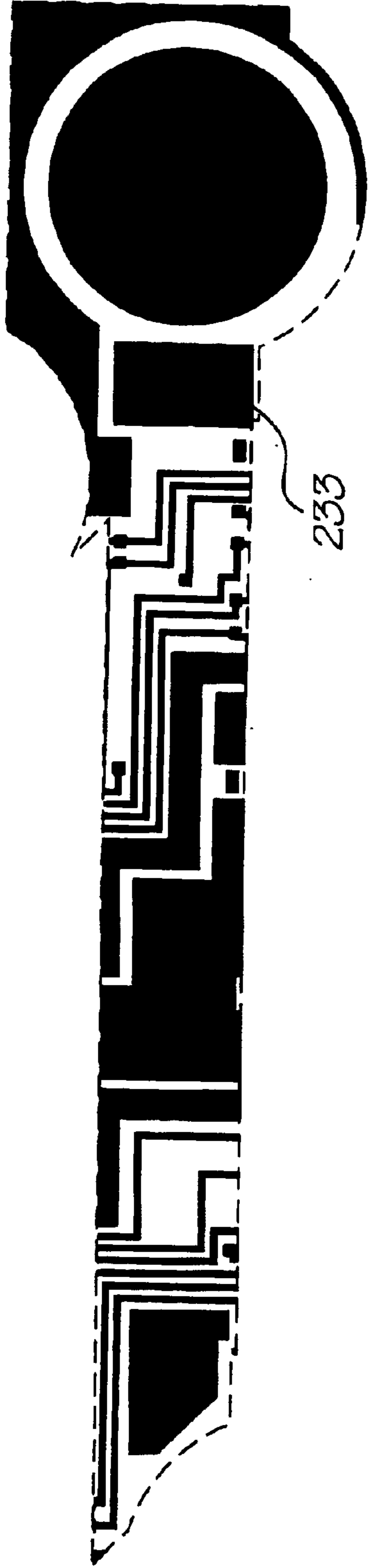
Metal 2 mask
