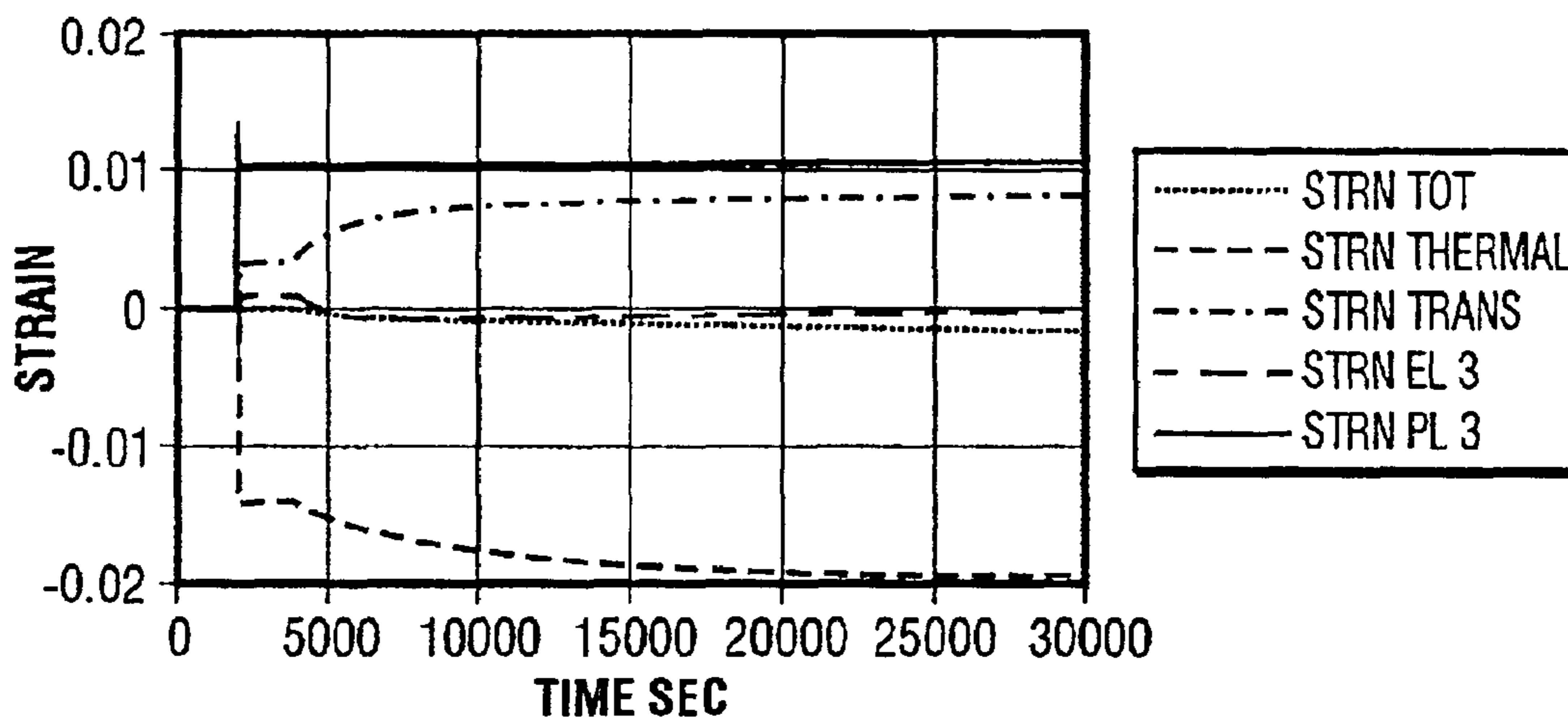
In-Plane Strains, Position #10 FIG. 5
