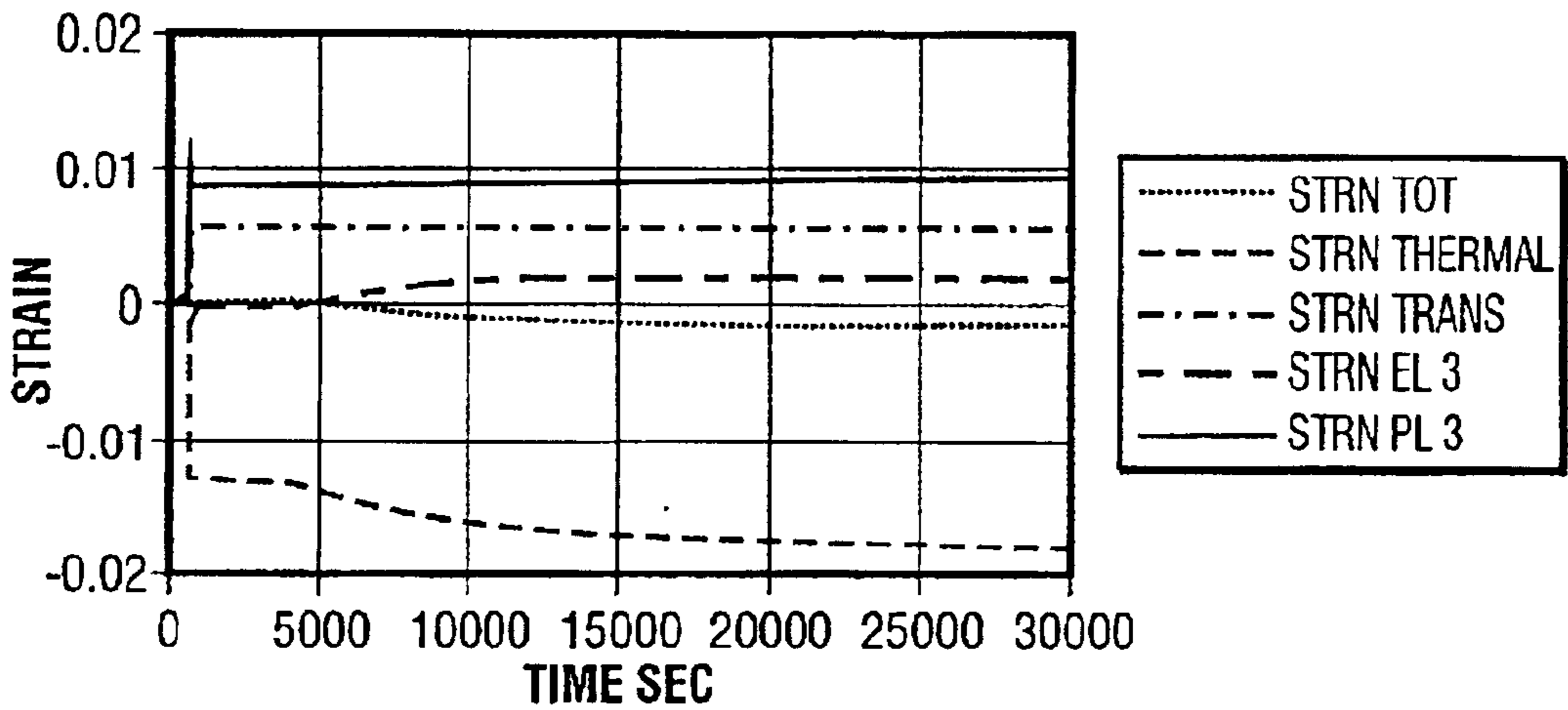
In-Plane Strains, Position #1 FIG. 9
