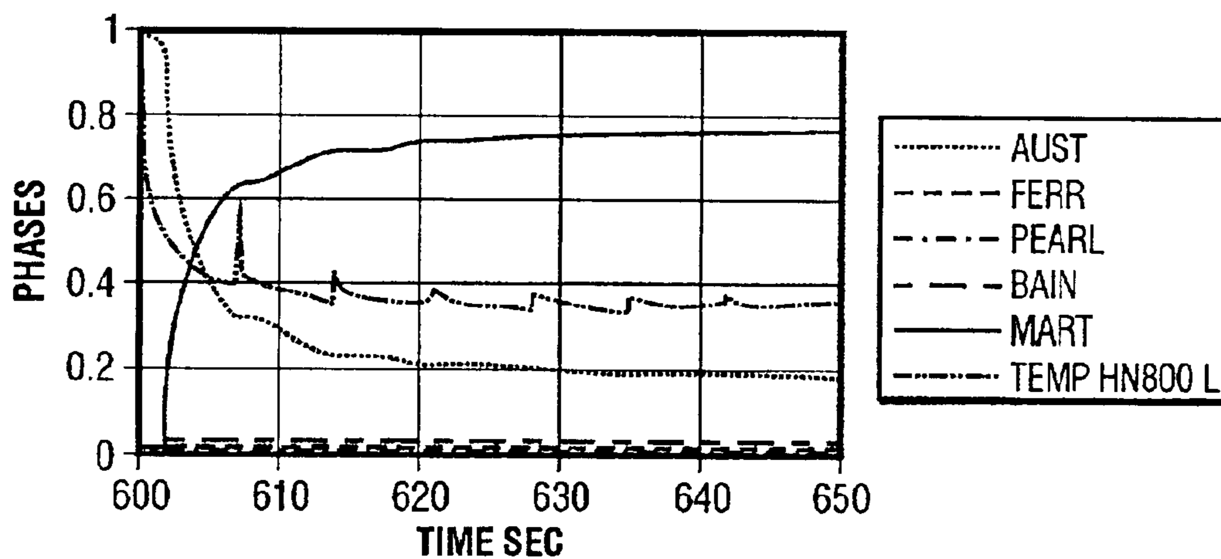
Phases, Position #1 FIG. 14
