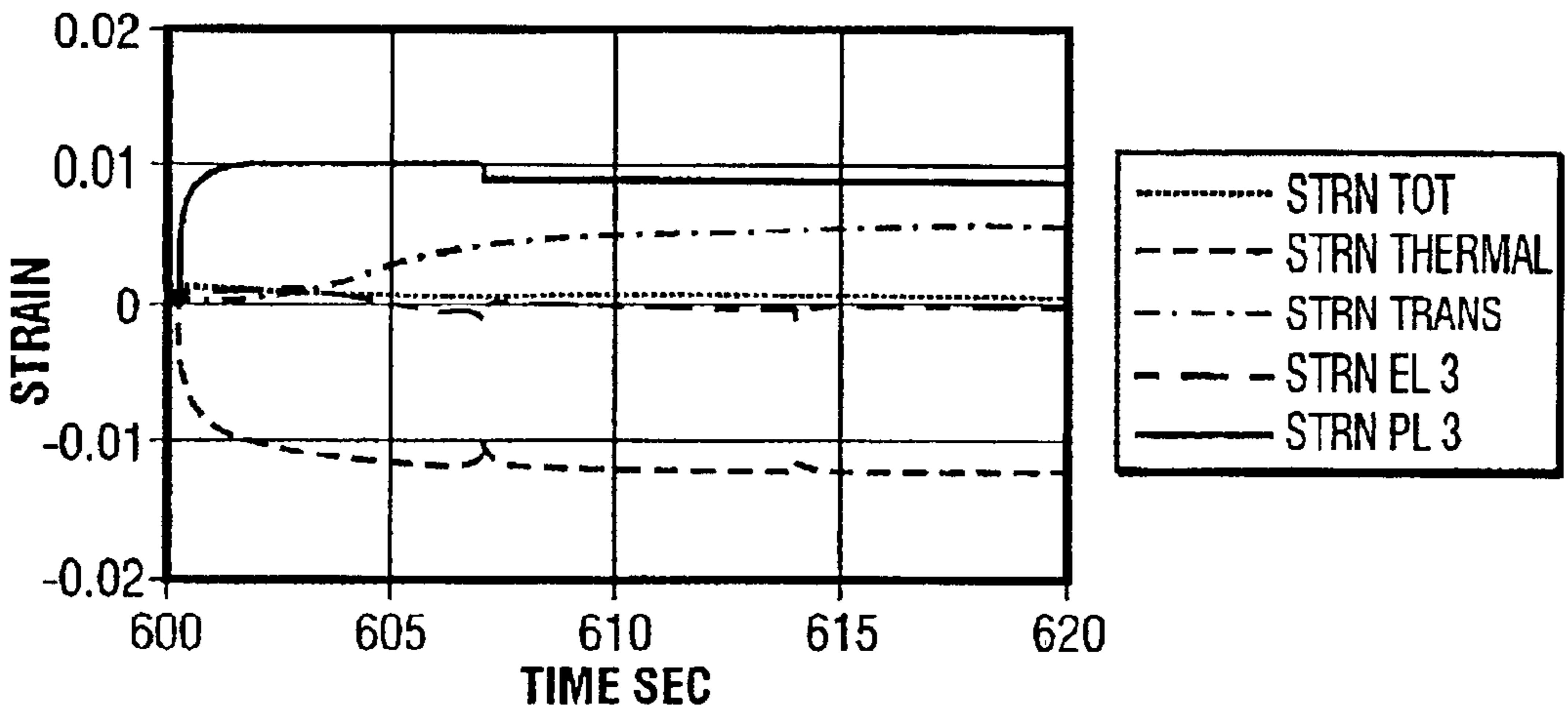
In-Plane Strains, Position #1 FIG. 10
