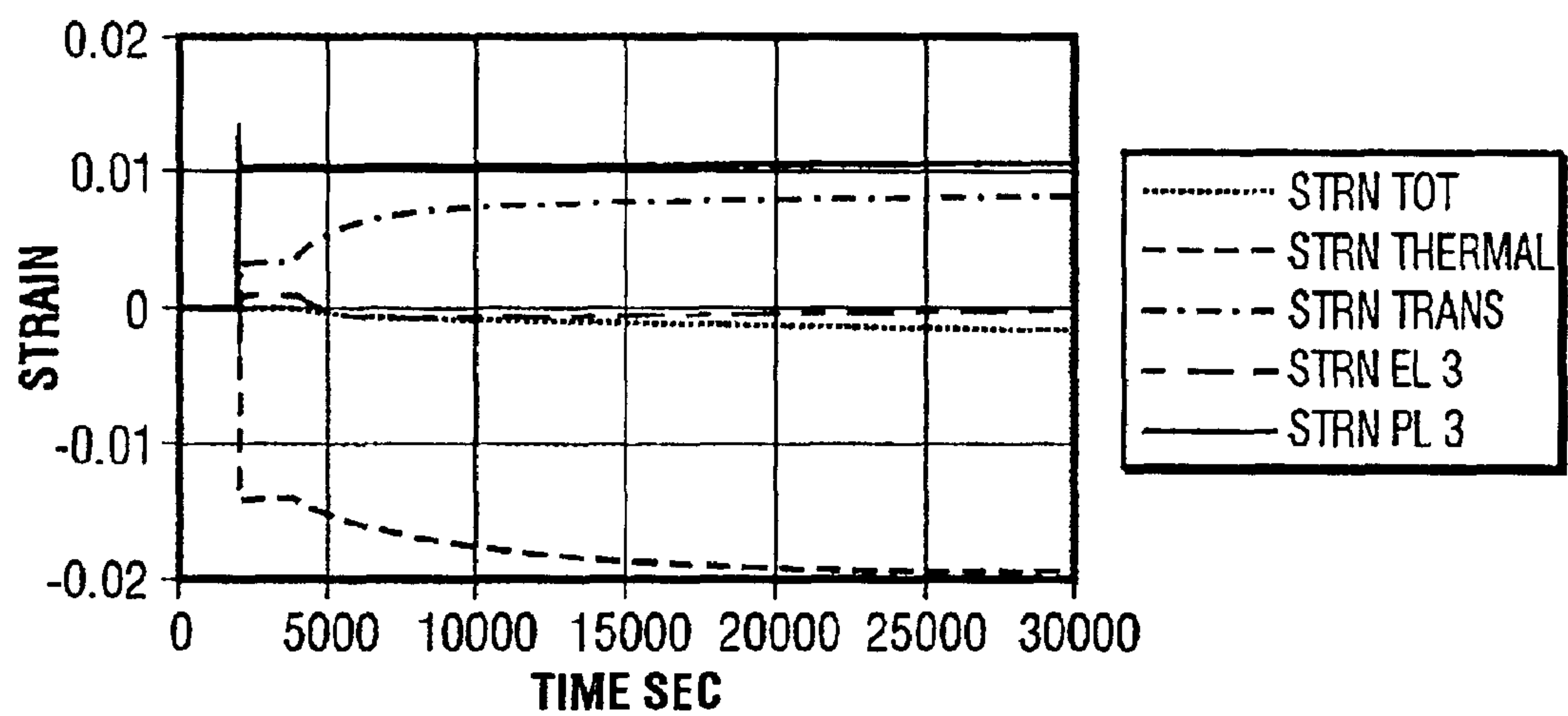
In-Plane Strains, Position #10 FIG. 5
