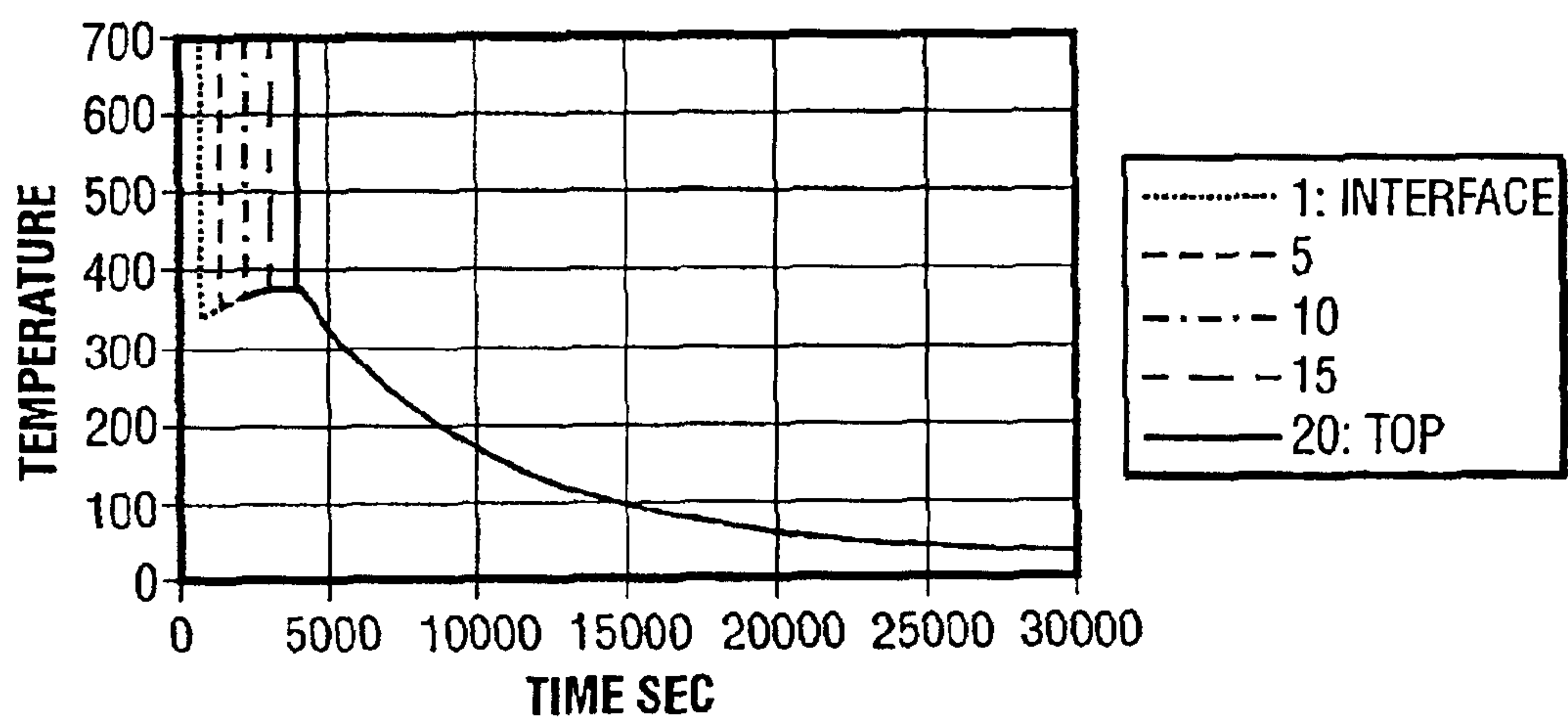
Temperature FIG. 3
