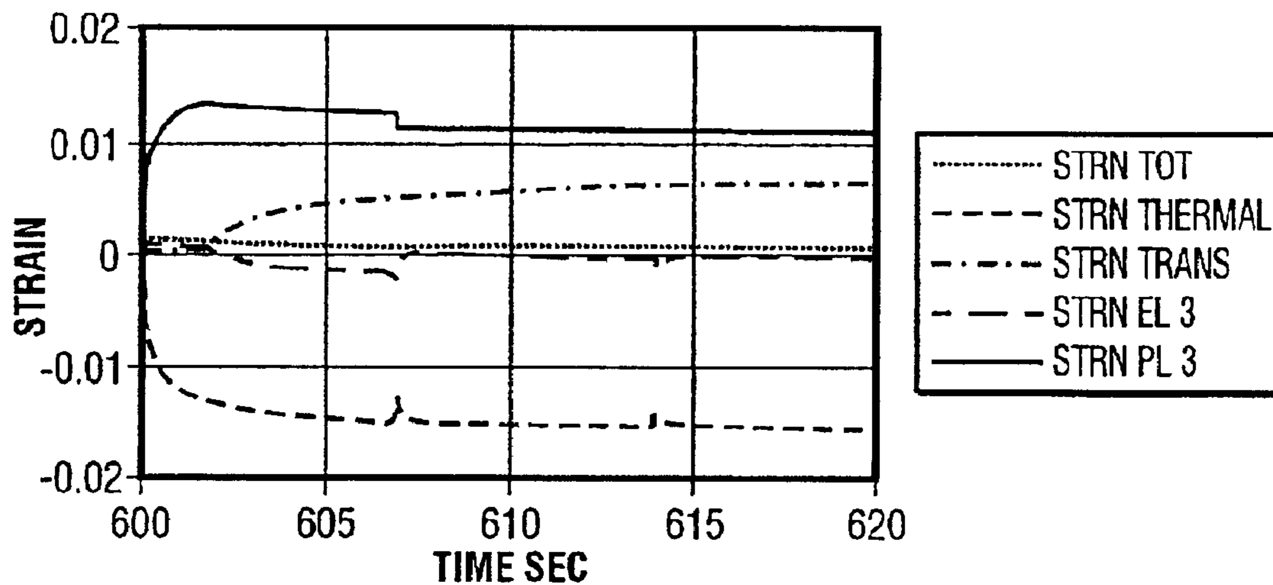
In-Plane Strains, Position #1
