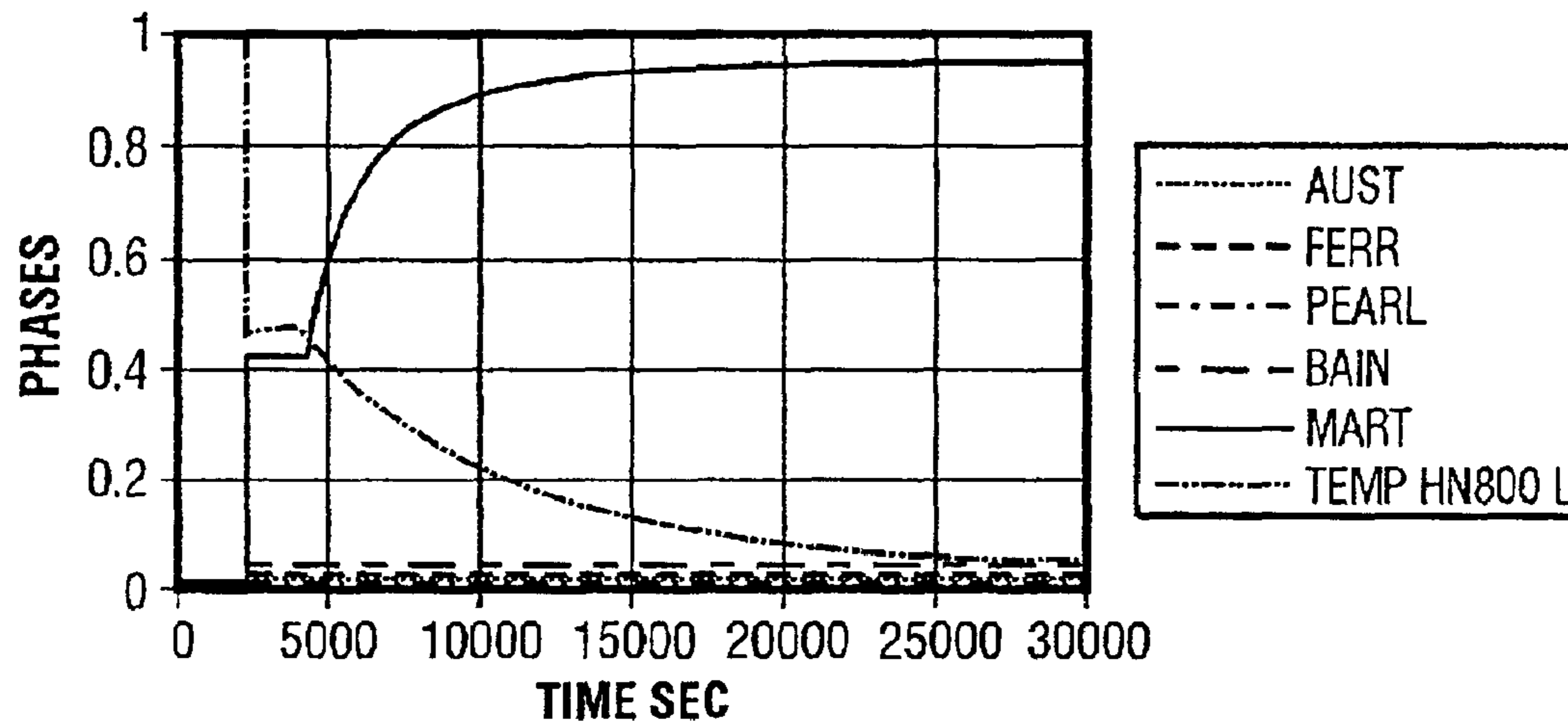
Phases, Position #10 FIG. 4
