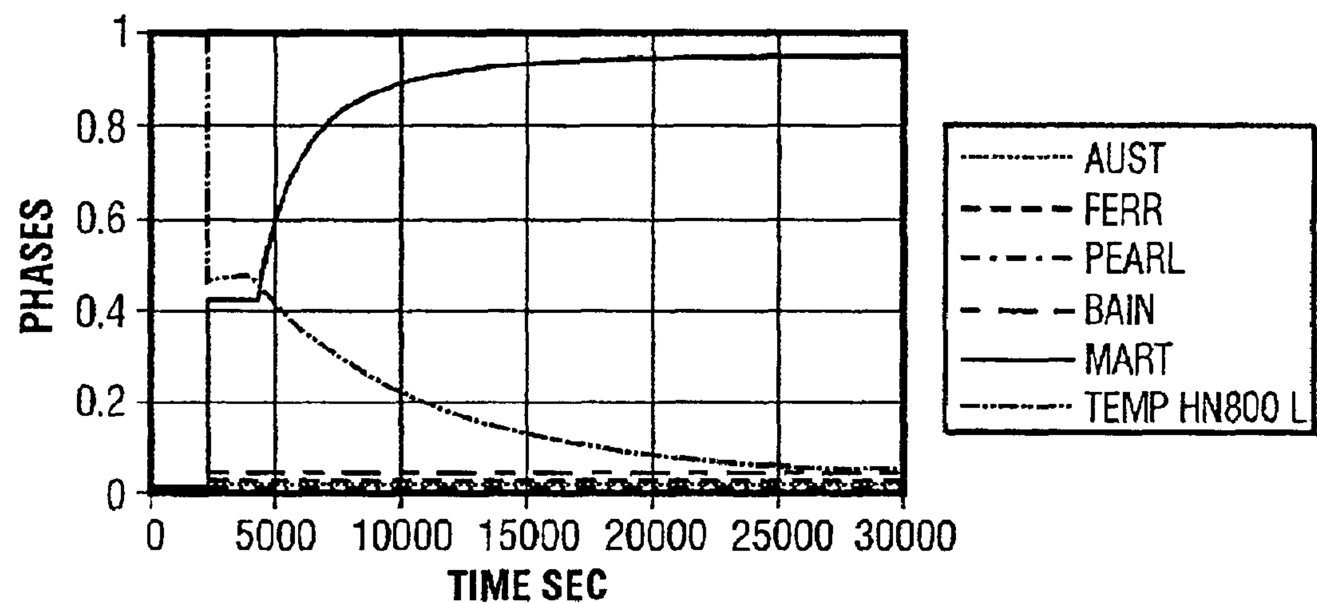
Phases, Position #10 FIG. 4
