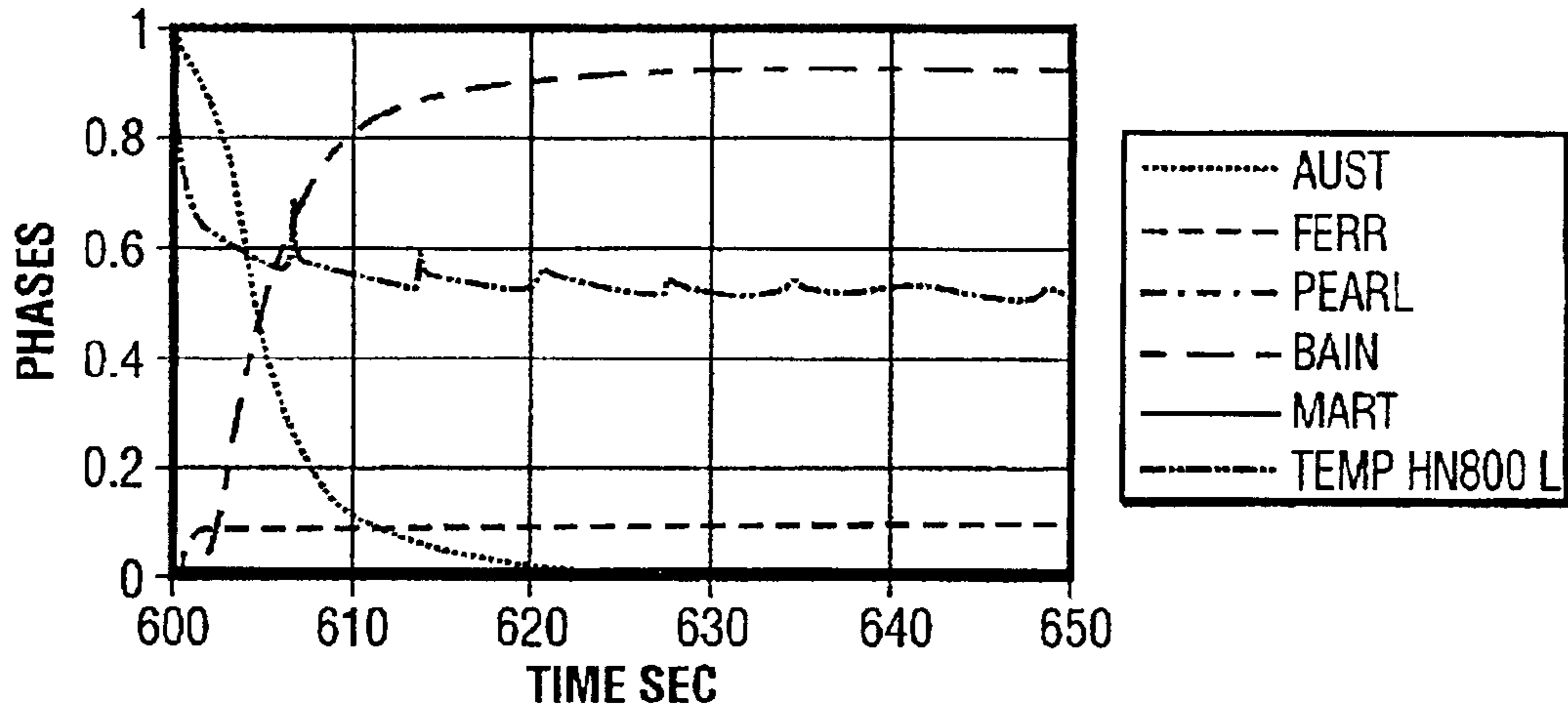
Phases, Position #1 FIG. 8
