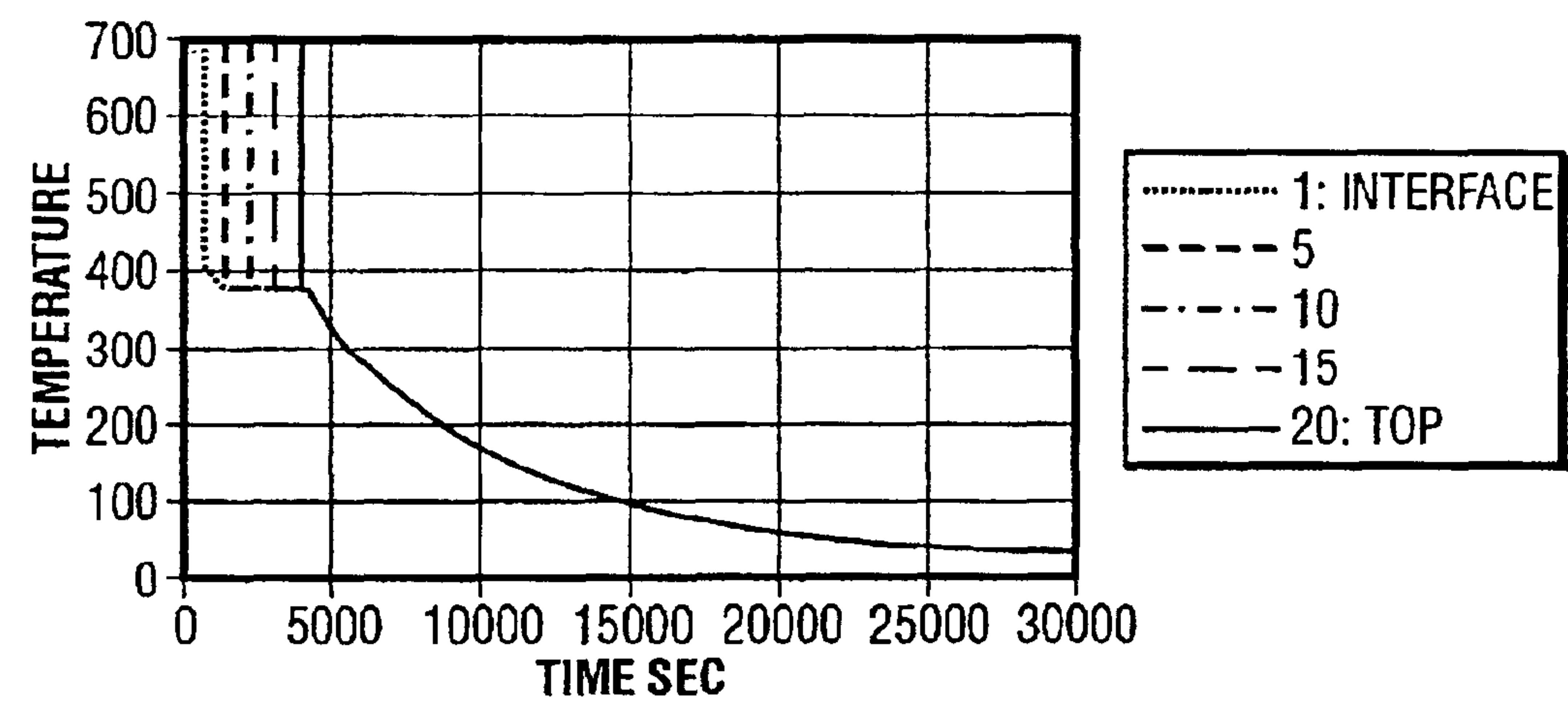
Temperature FIG. 7
