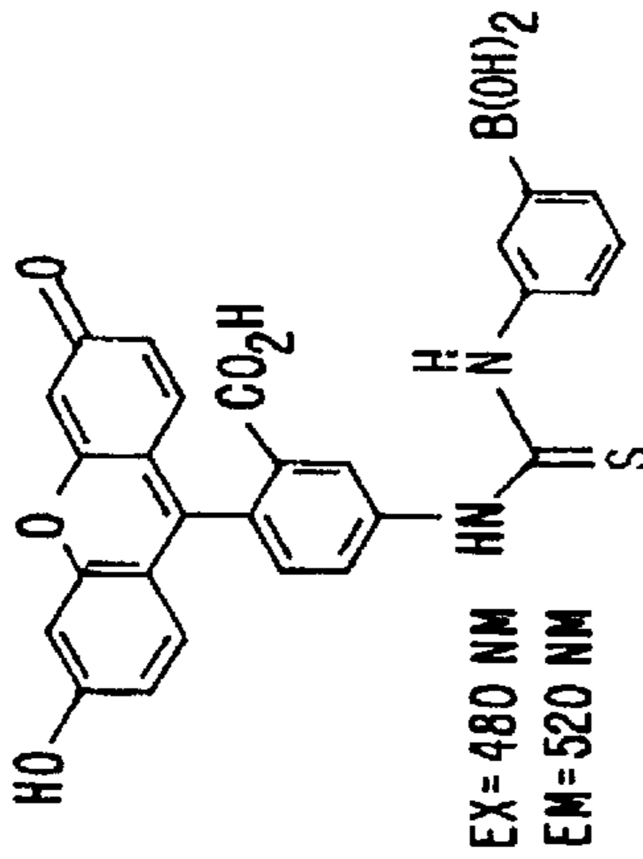
FLUORESCIN-2
