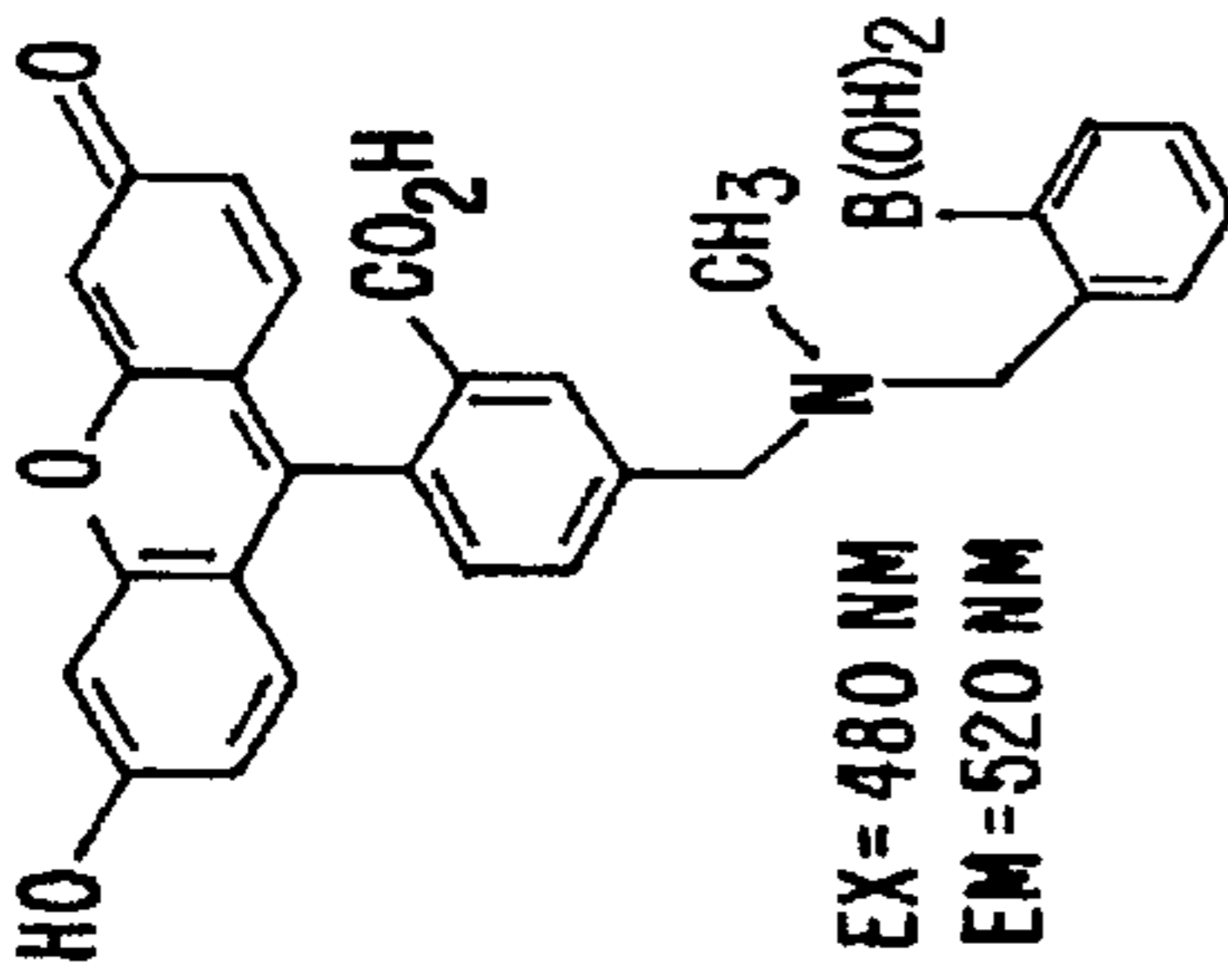
FLUORESCIN-1
