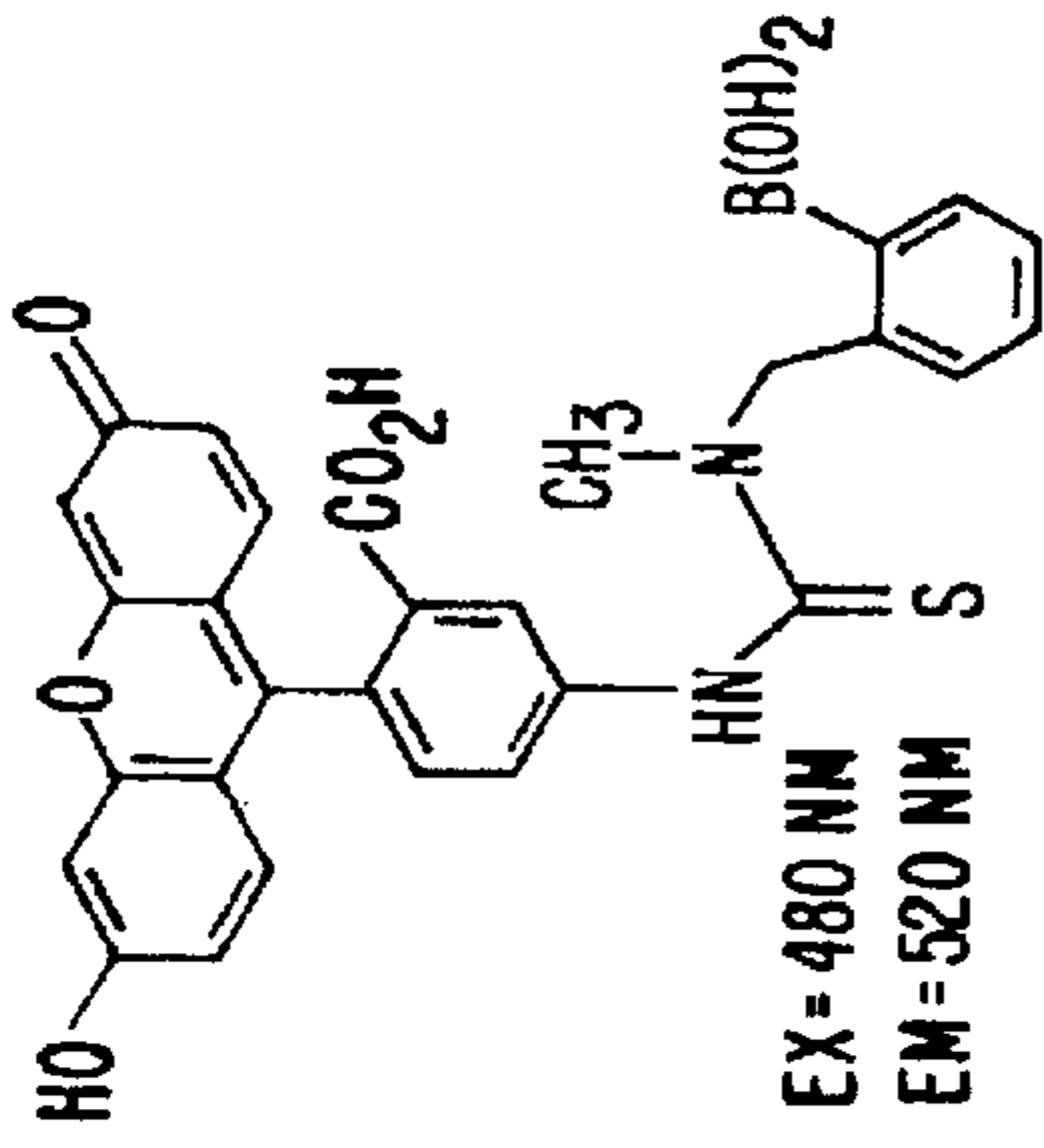
FLUORESCIN-3
