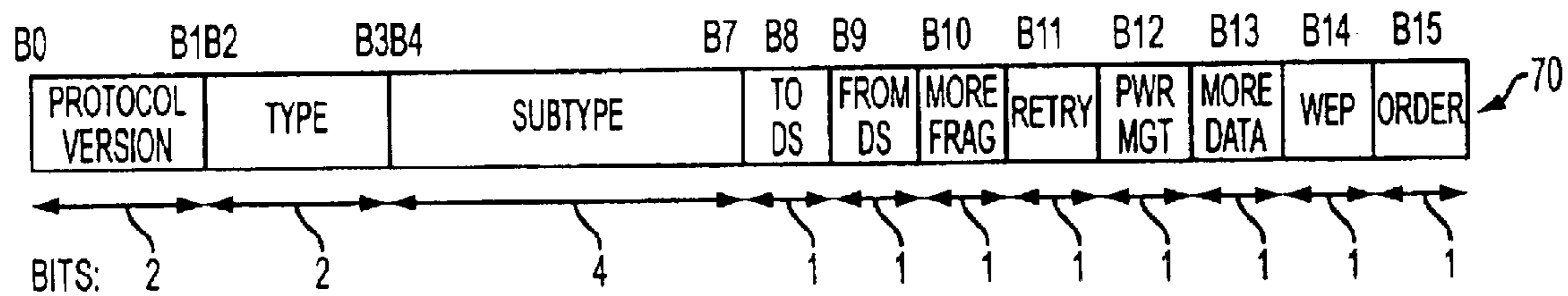
FIG. 9 (PRIOR ART)
