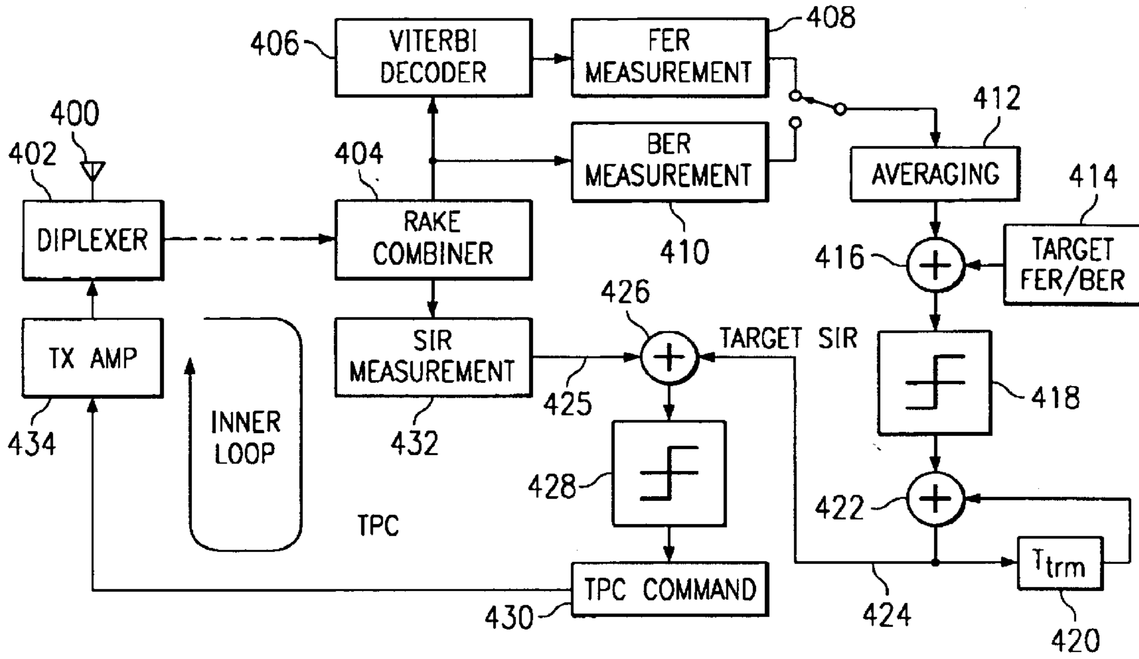
FIG. 4 (PRIOR ART)
