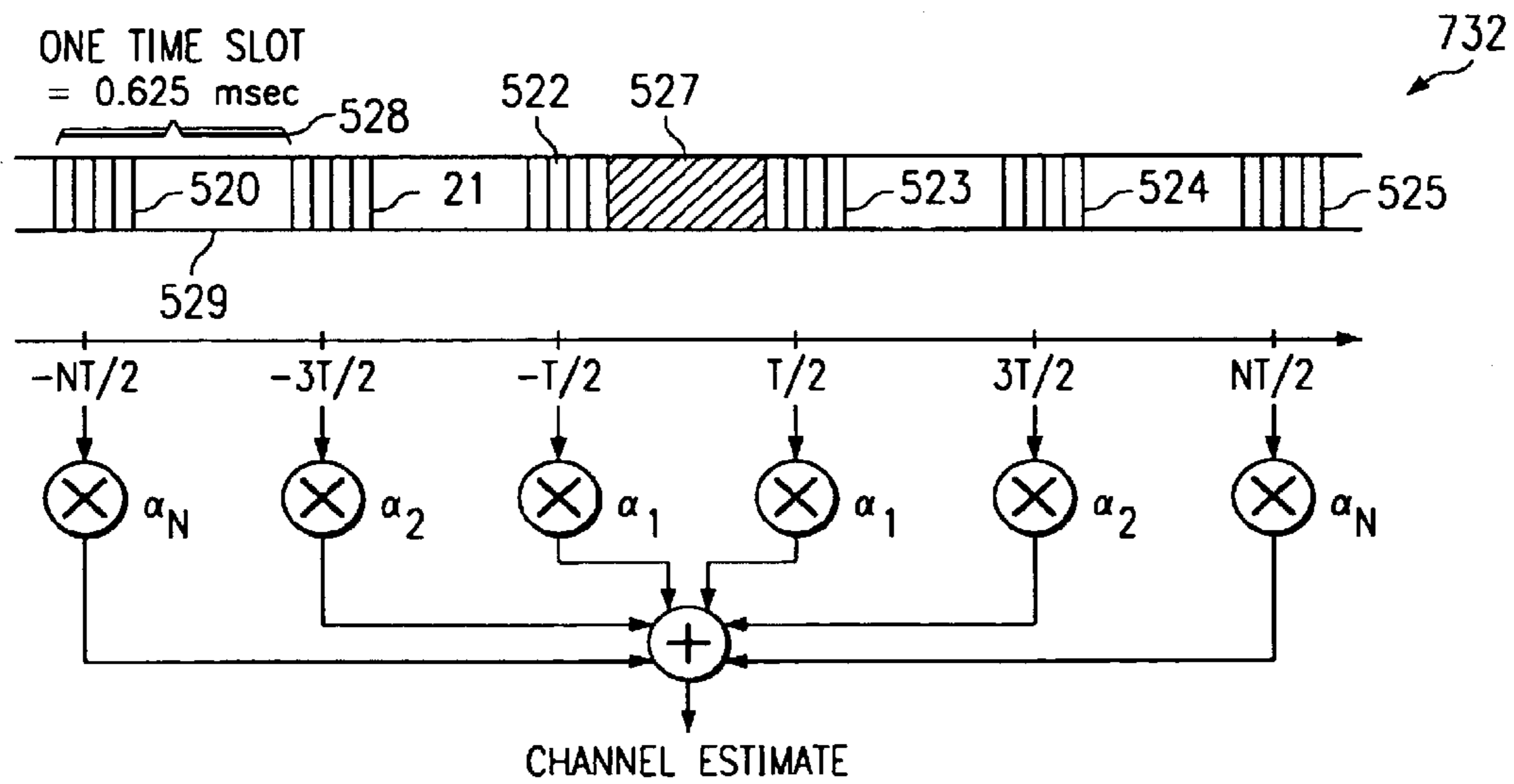
FIG. 5 (PRIOR ART)
