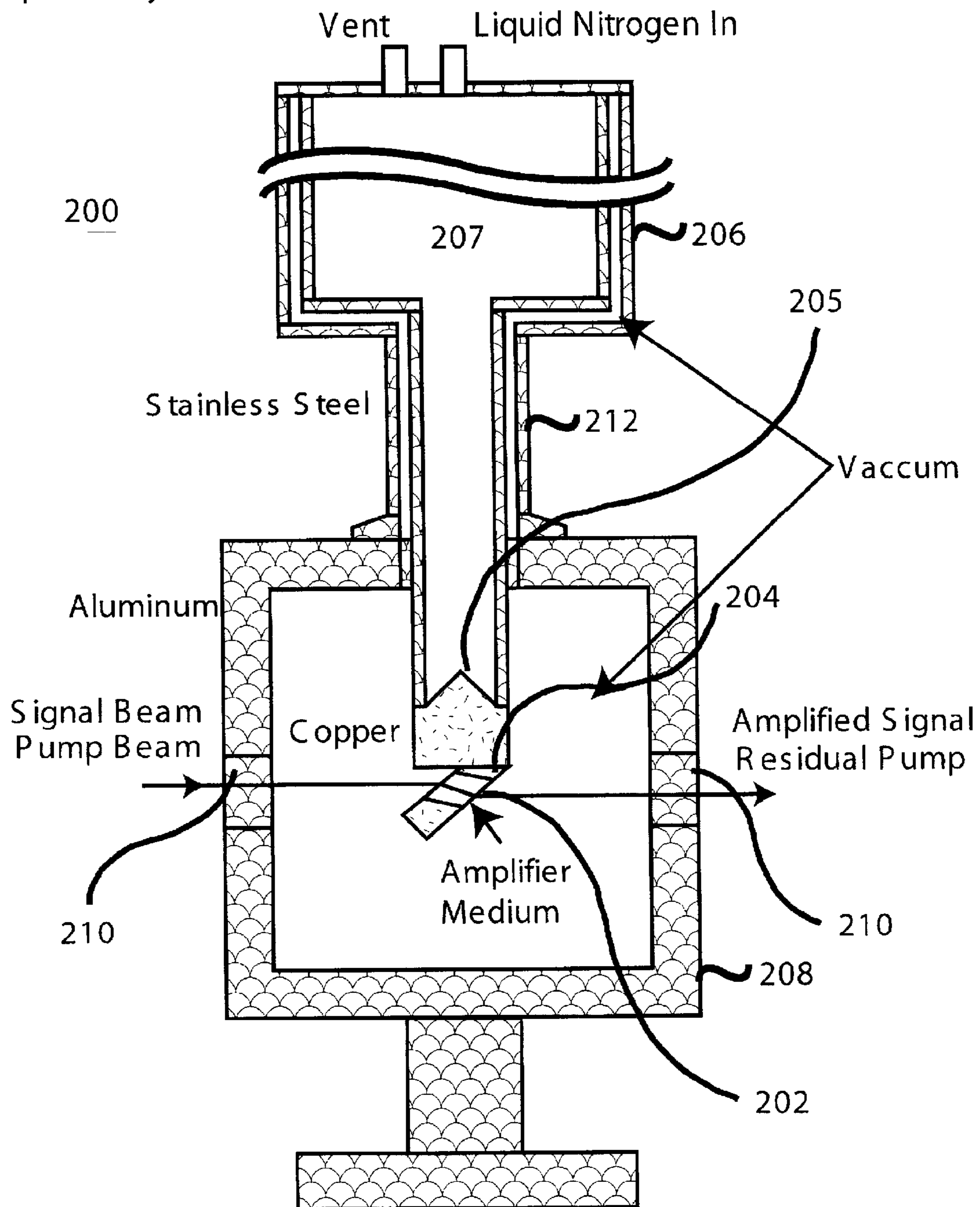
Figure 2 Amplifier Cryo-cell
