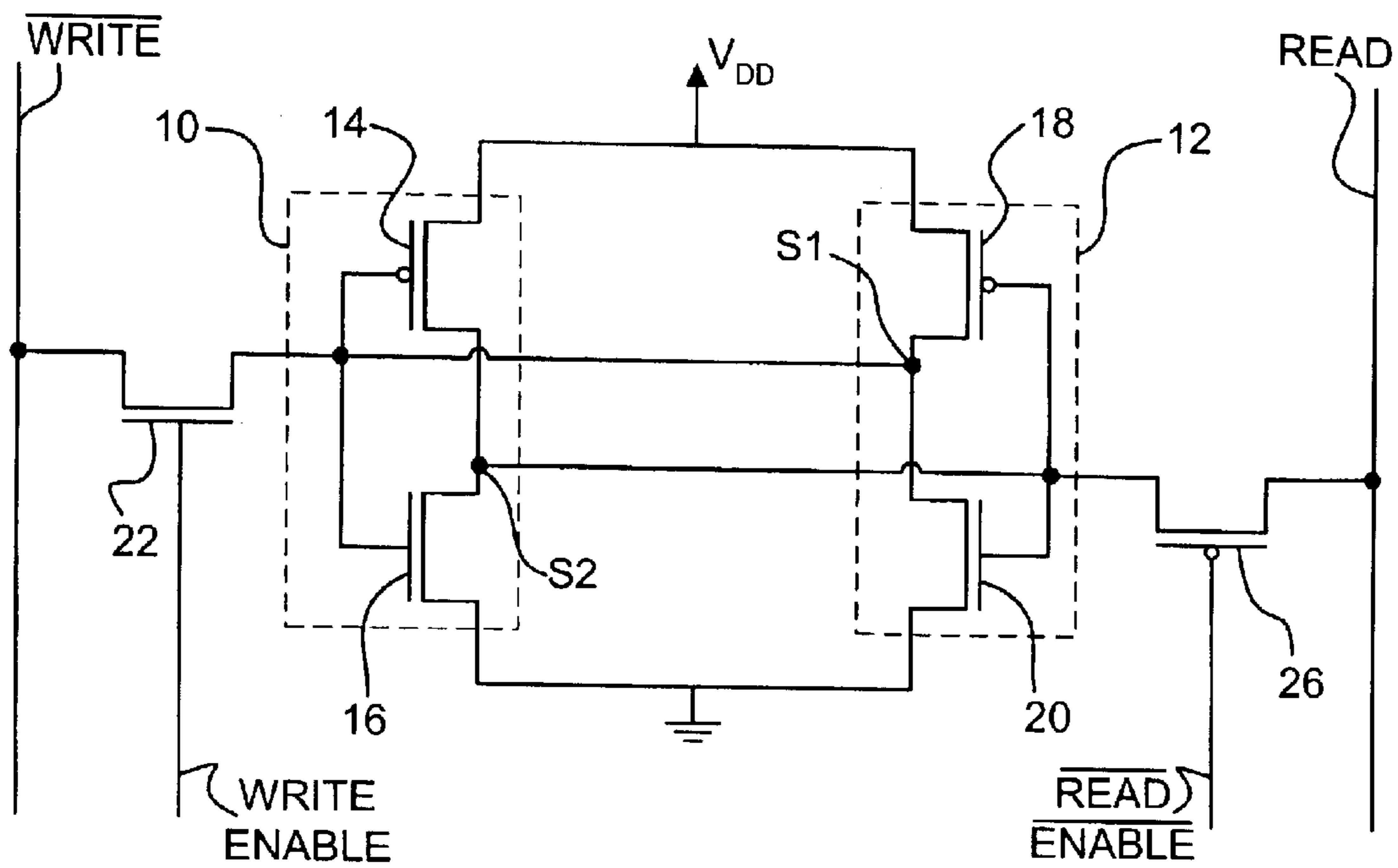
FIGURE 3 (PRIOR ART)
