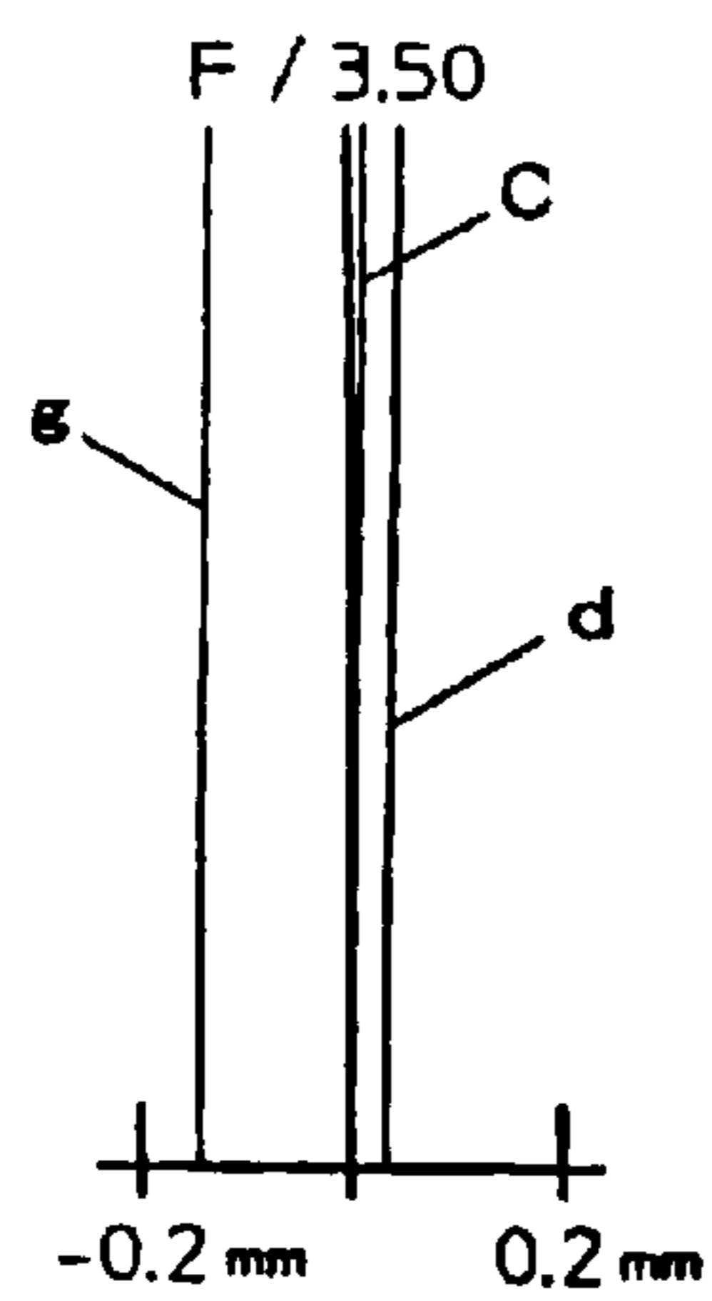
Spherical Aberration Fig. 5A
