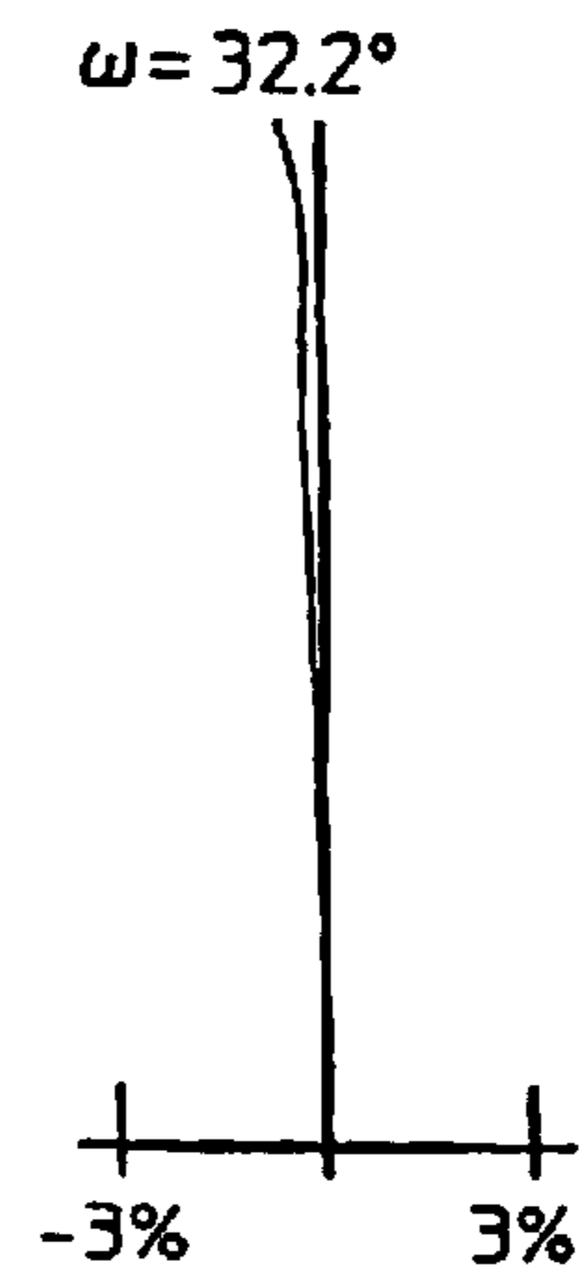
Distortion Fig. 4C
