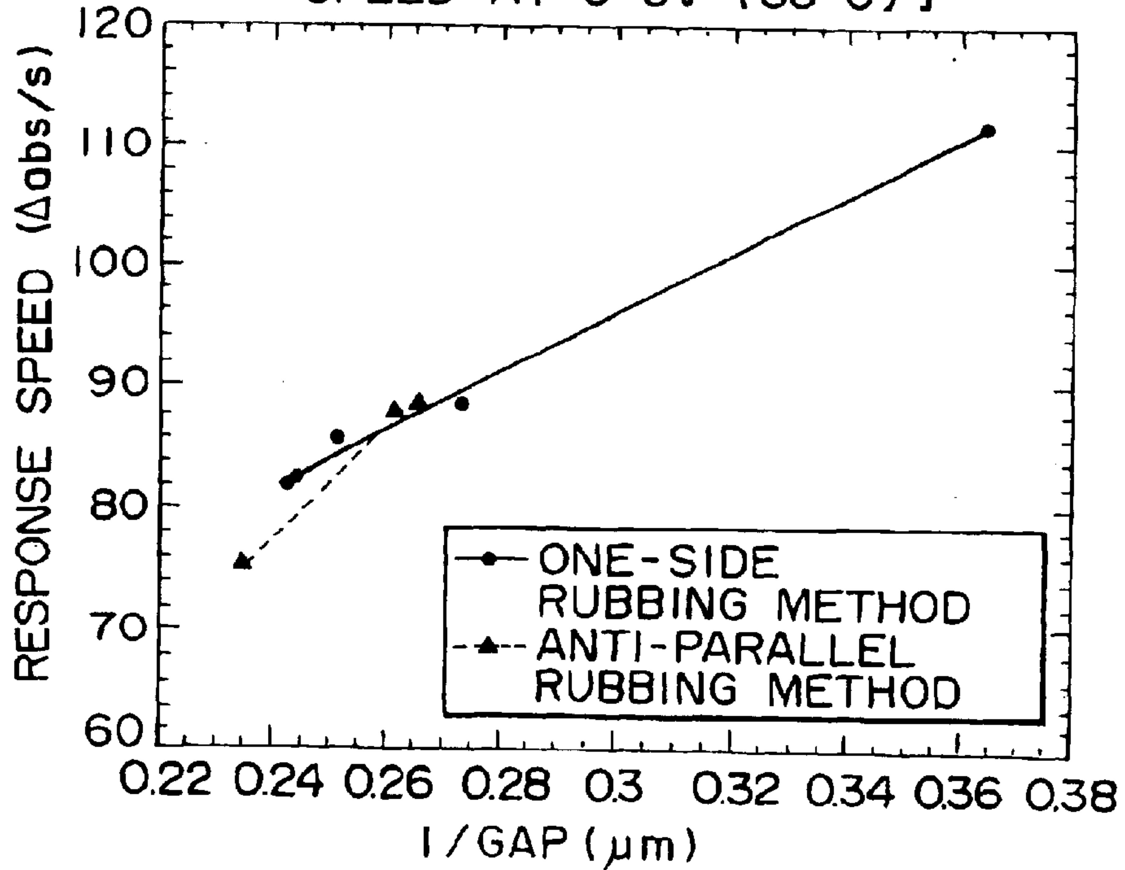
[ COMPARISON IN RESPONSE SPEED AT 0-5V (65°C) ]
