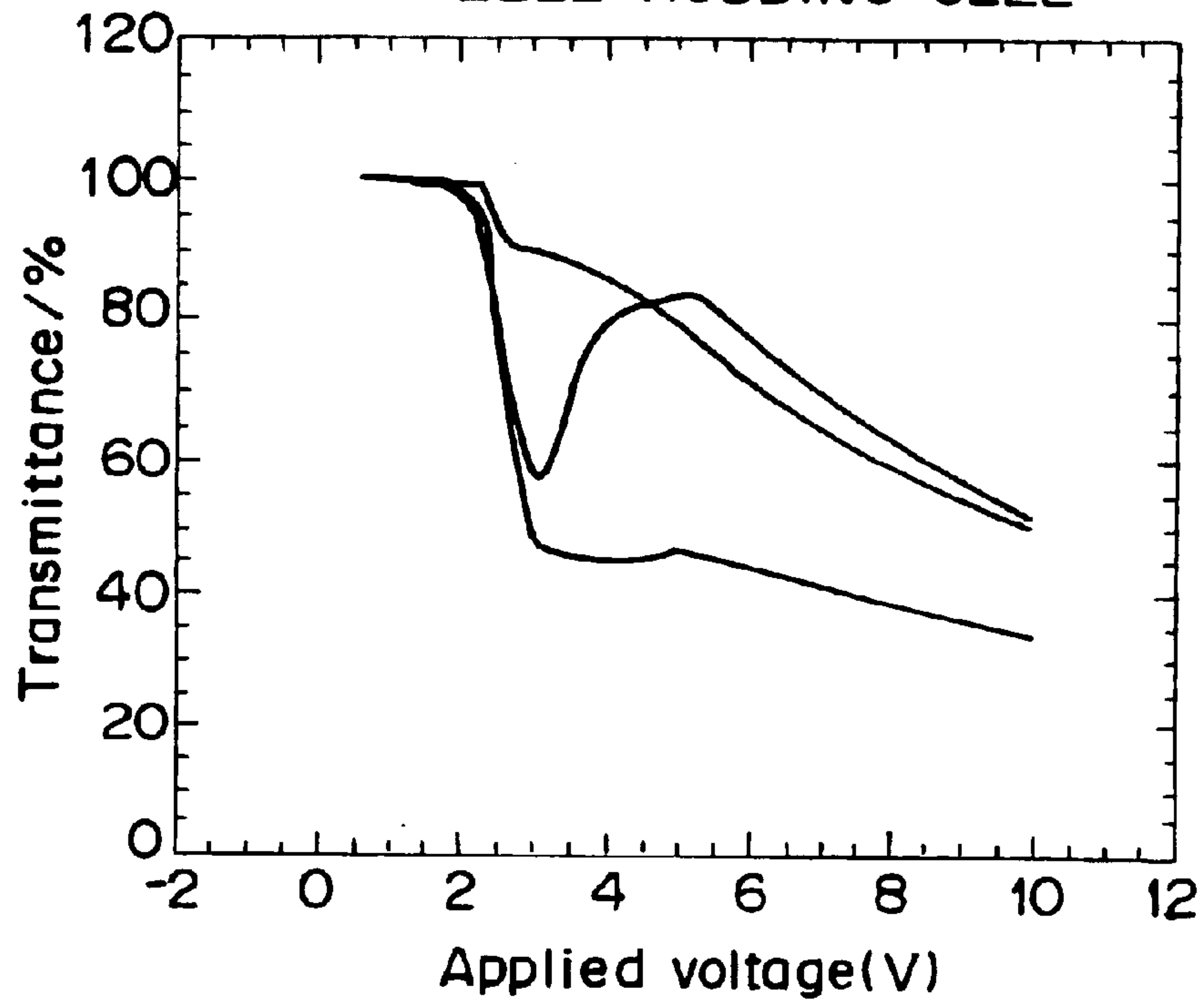
FIG. 6A PARALLEL RUBBING CELL
