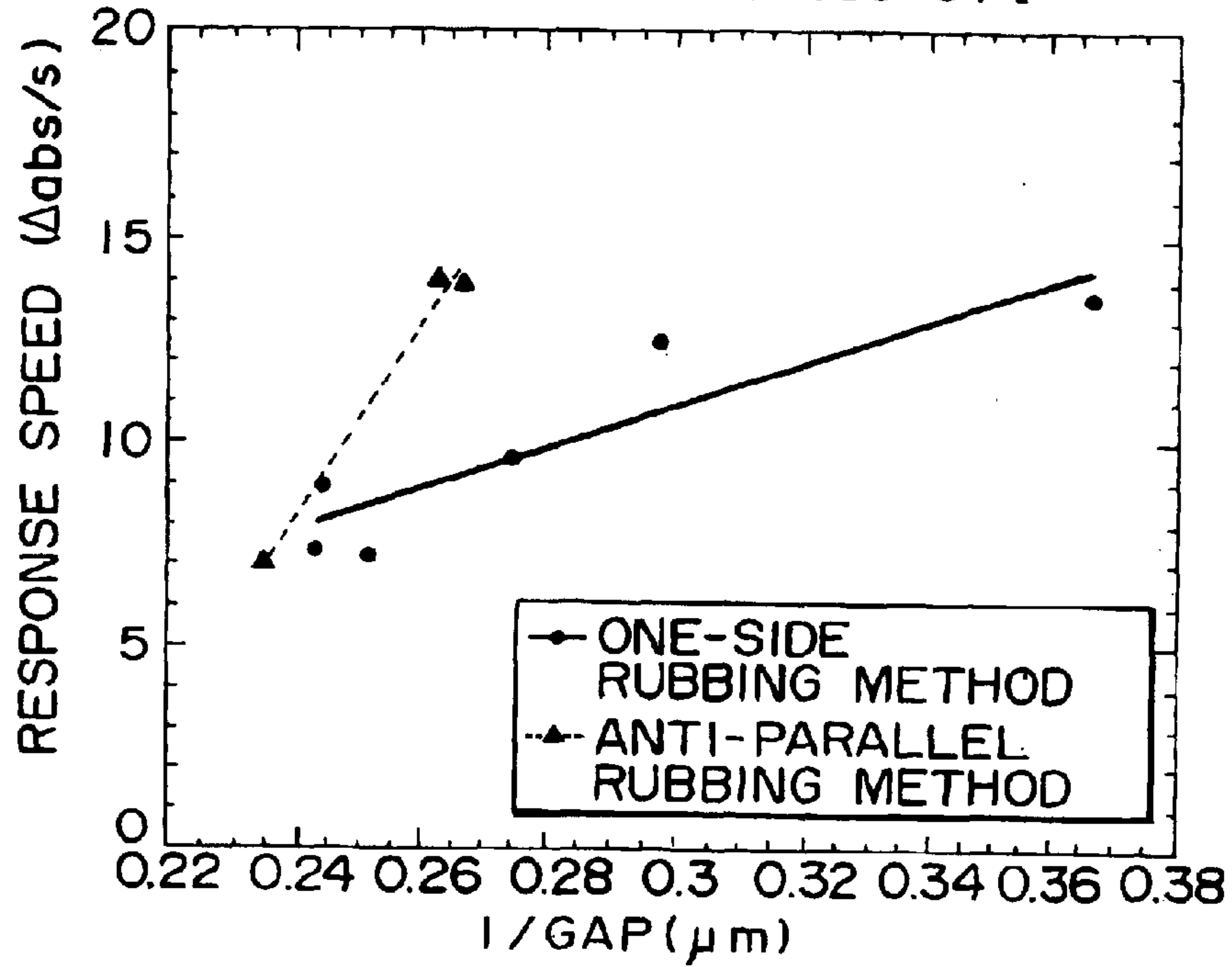
[ COMPARISON IN RESPONSE SPEED AT 0-5V (65°C) ]
