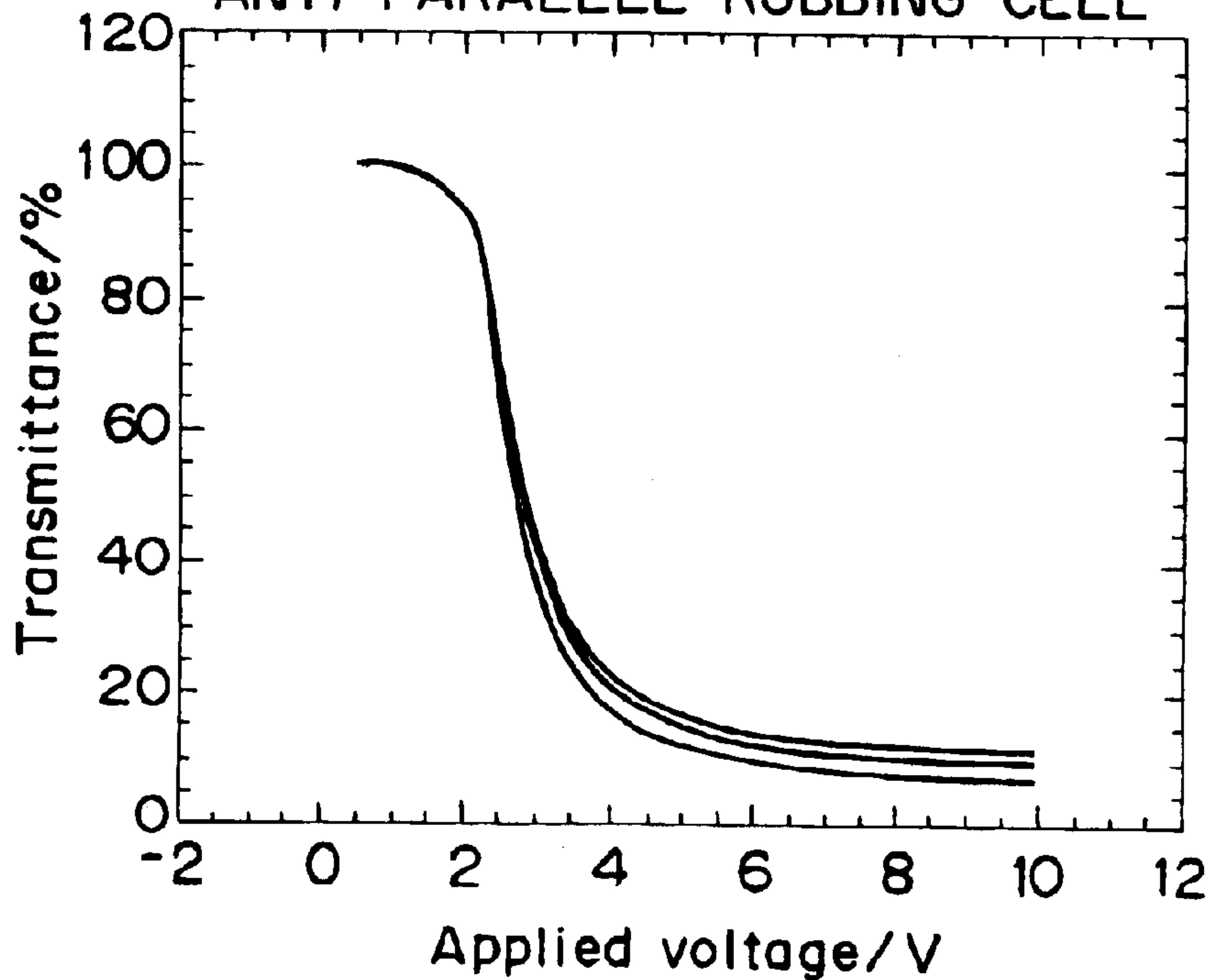
FIG. 6B ANTI-PARALLEL RUBBING CELL
