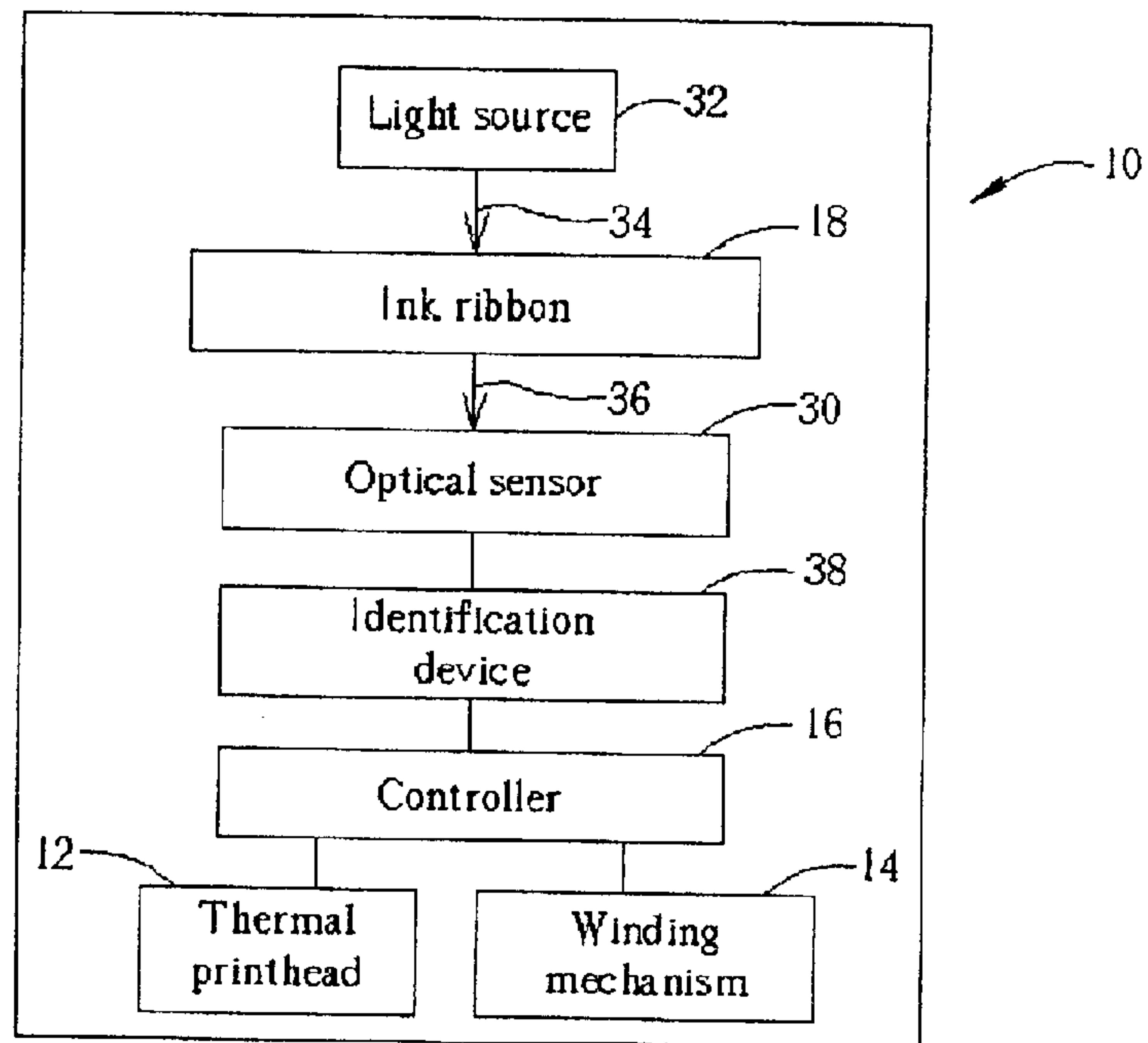
Fig. 2 Prior art
