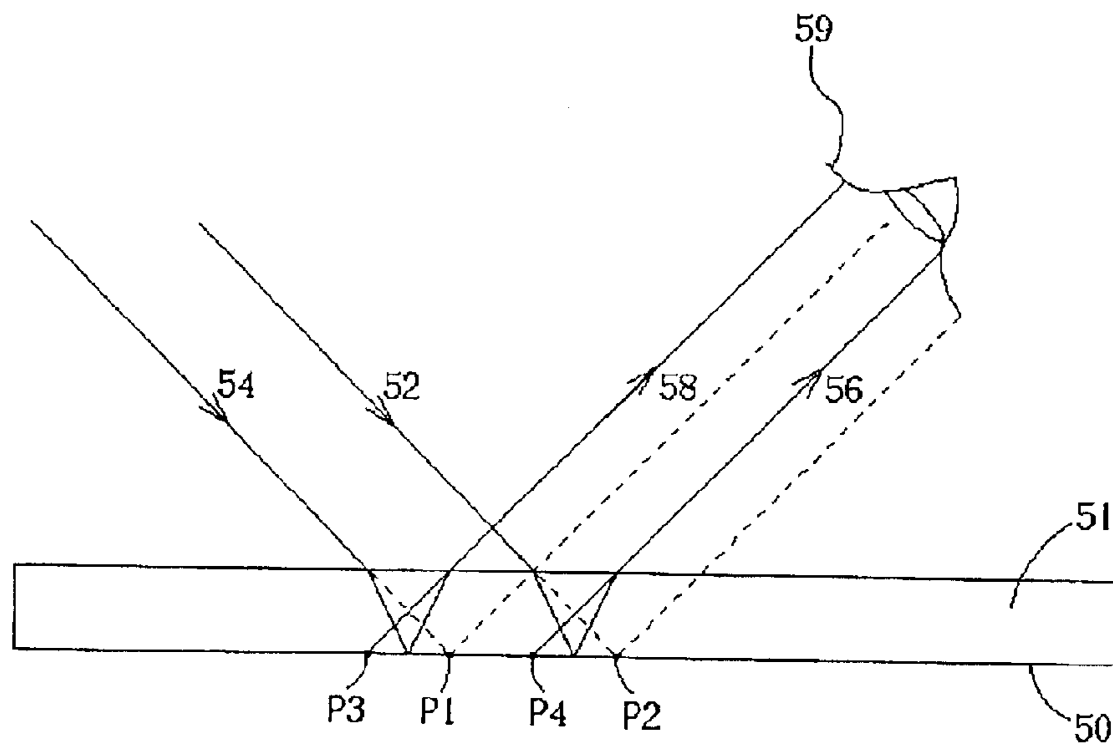
Fig. 5 Prior art
