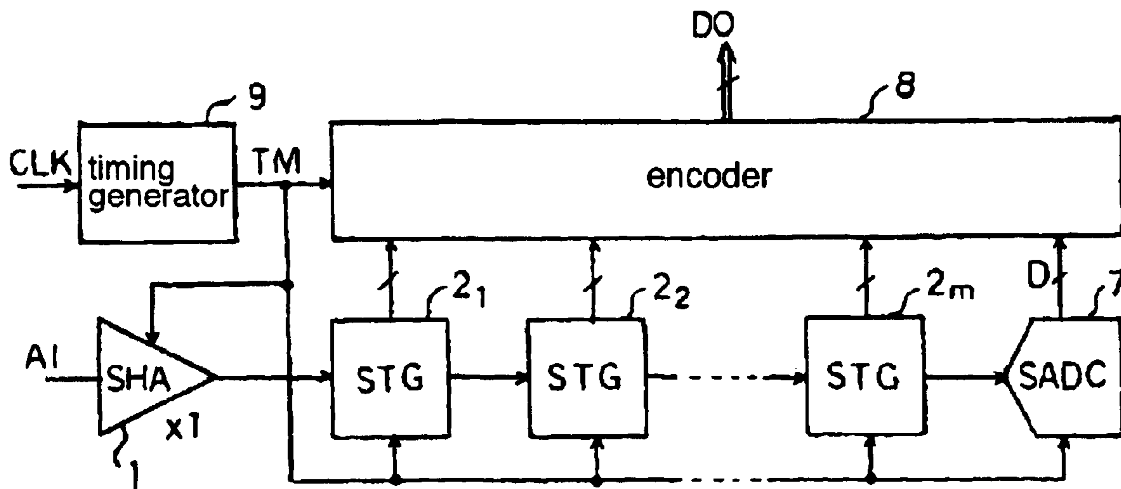
FIG. 1 (PRIOR ART)
