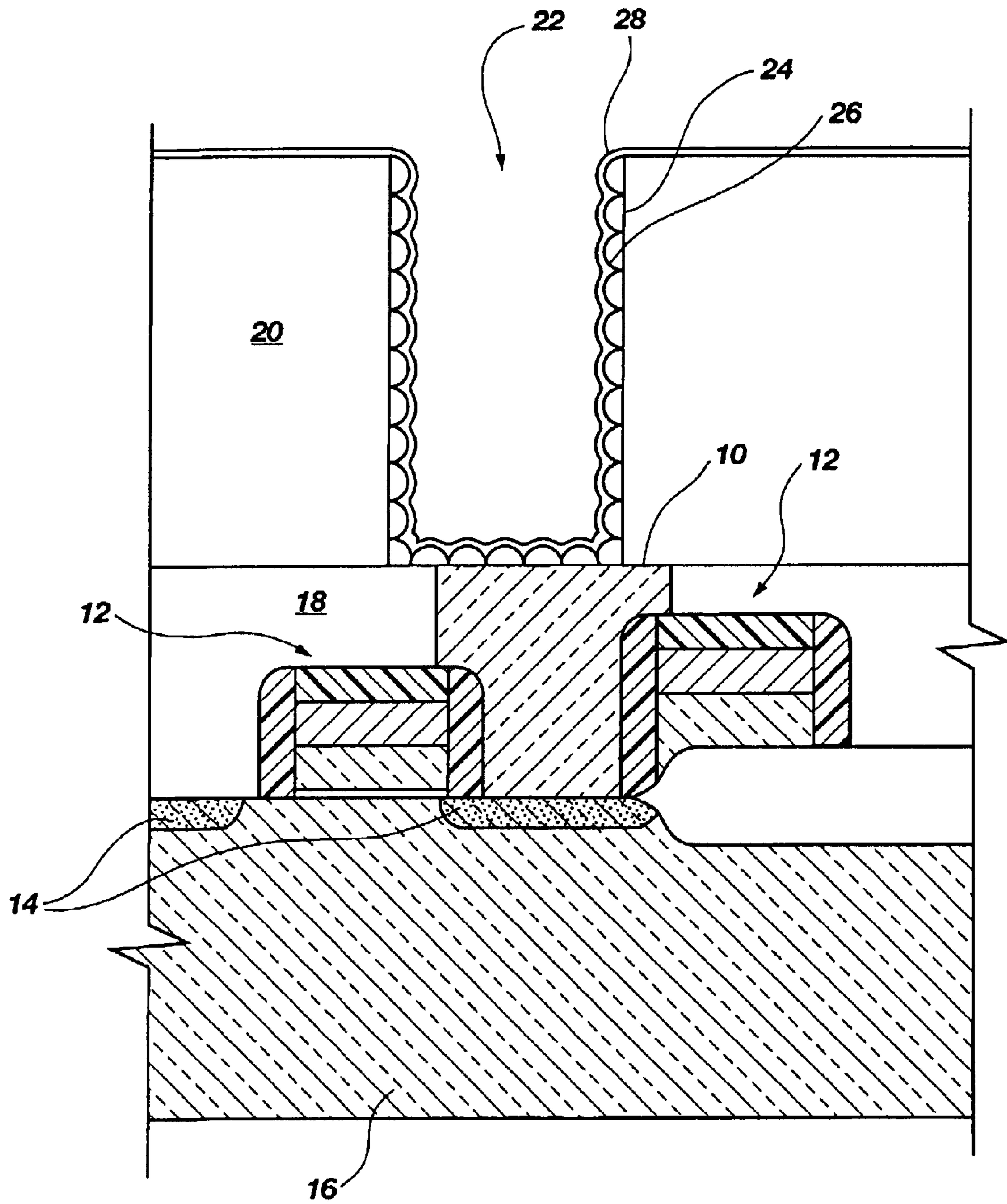
Fig. 1 (PRIOR ART)
