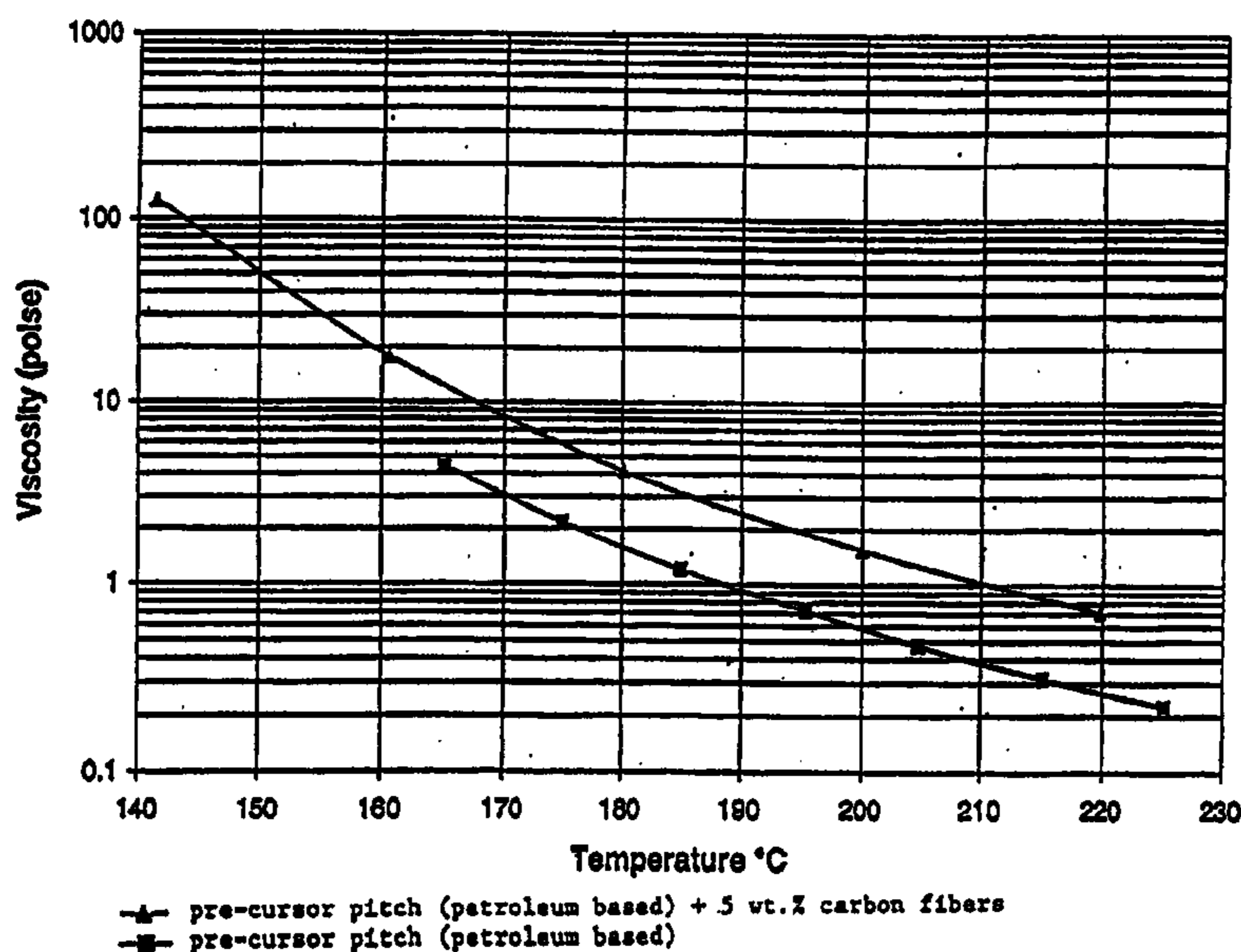
VISCOSITY v. TEMPERATURE
