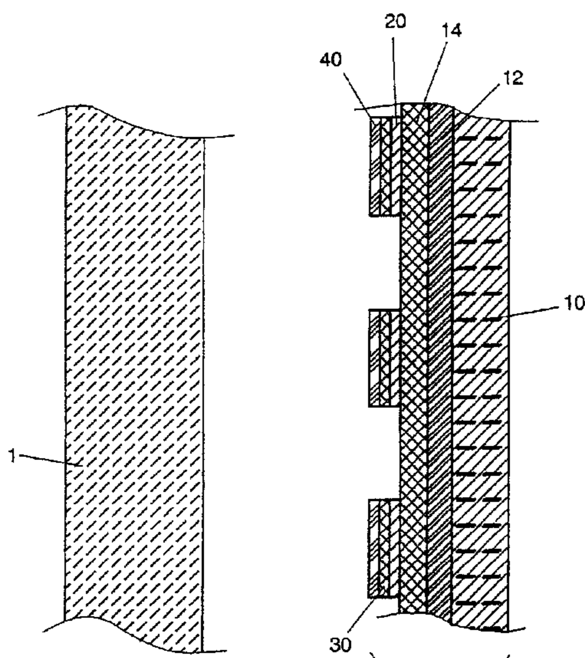
LABEL & SUBSTRATE EXPLODED VIEW
