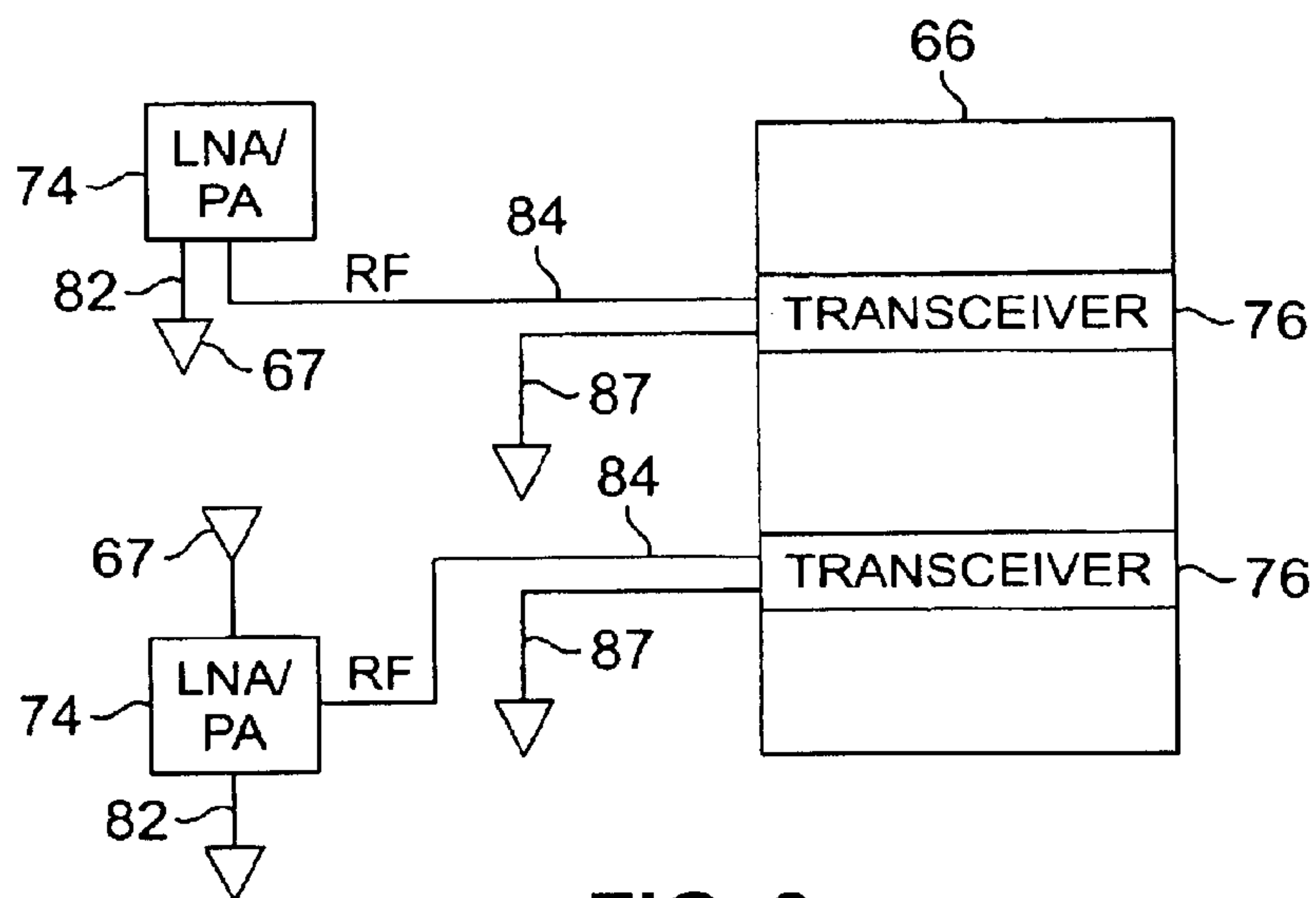
FIG. 6 (PRIOR ART)
