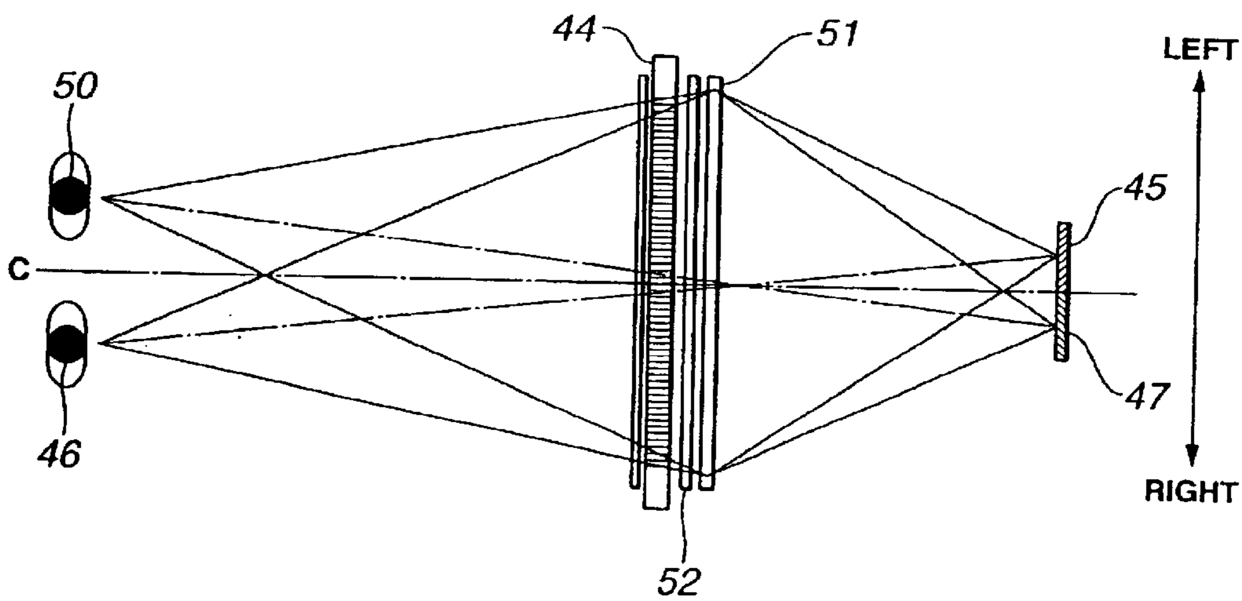
FIG.4 (PRIOR ART)
