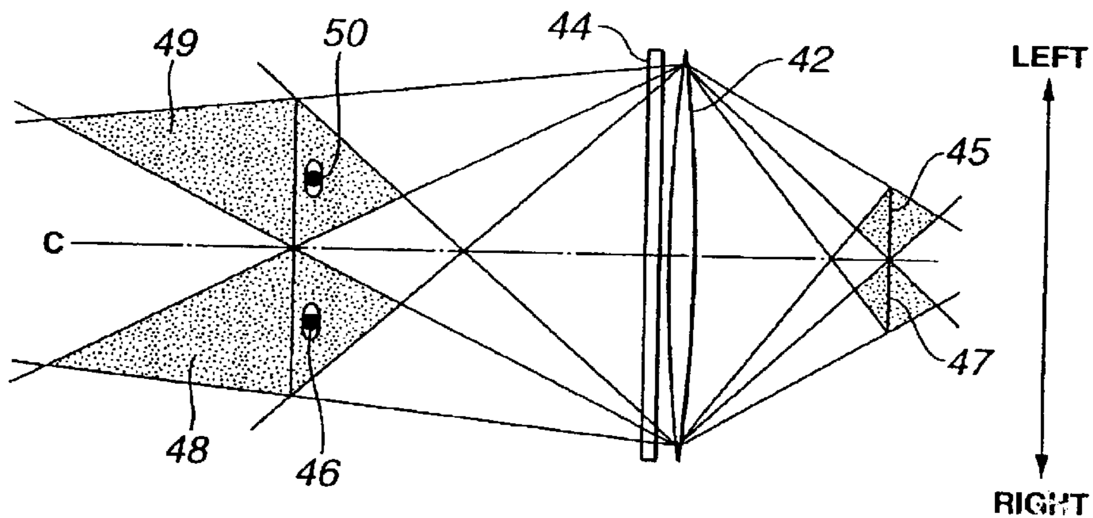
FIG.3 (PRIOR ART)
