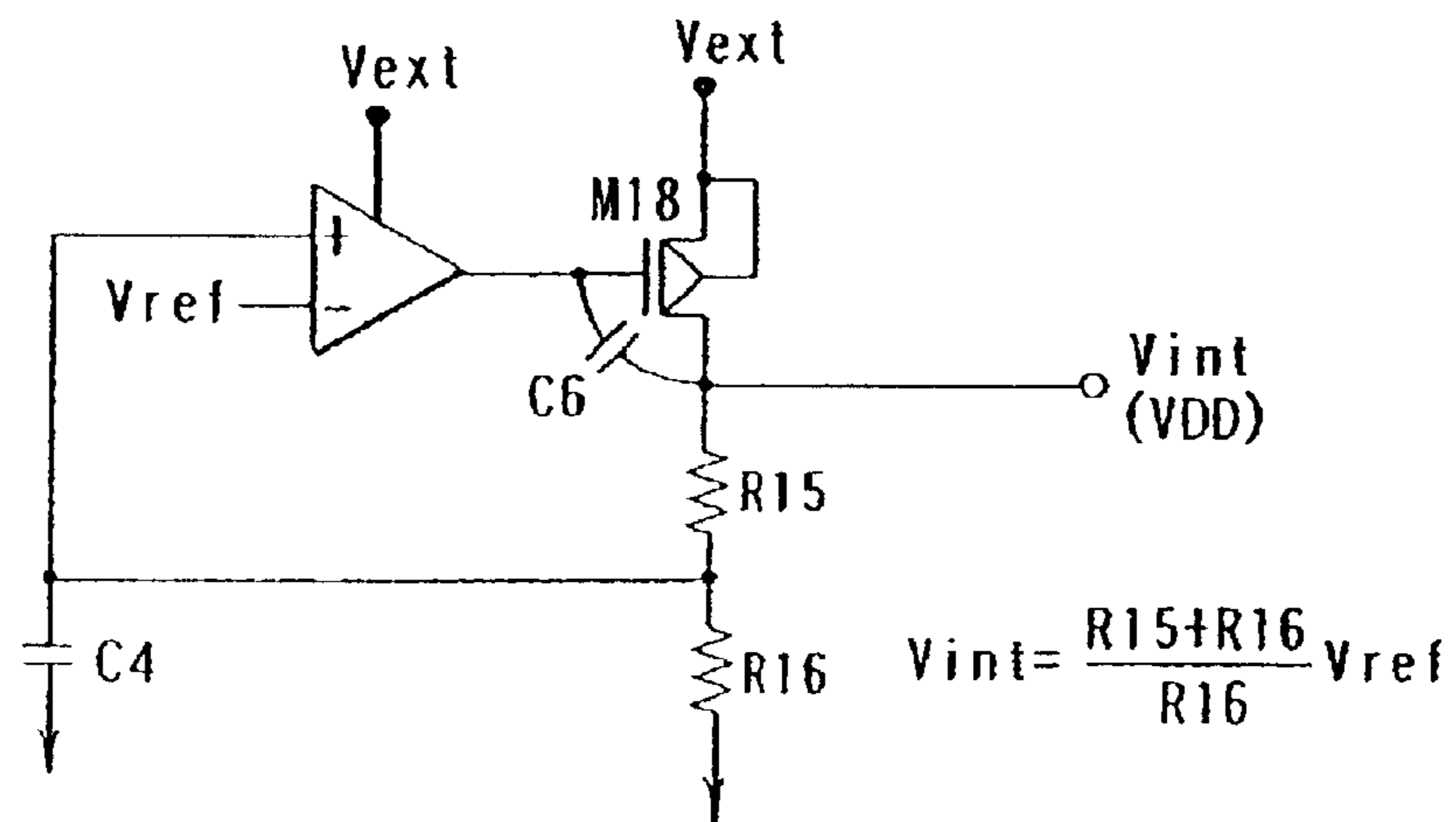
FIG. 29 (PRIOR ART)
