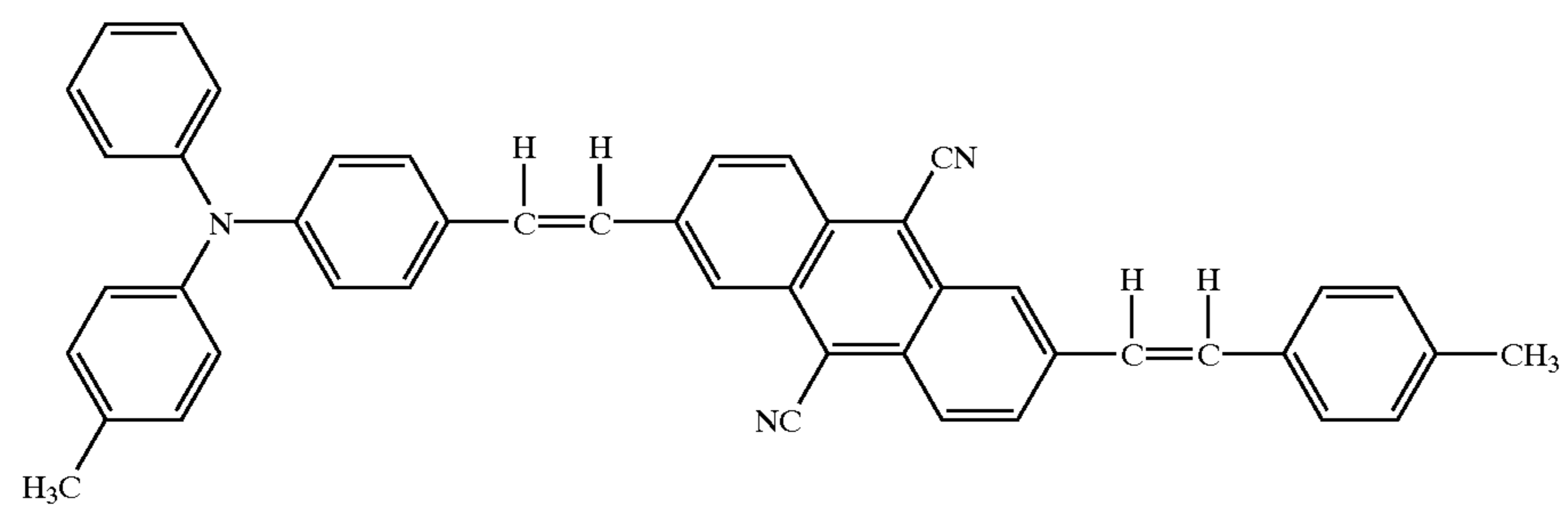
Structural formula (10)-4:
