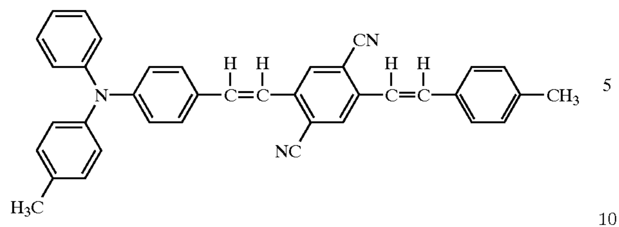
Structural formula (10)-3:
