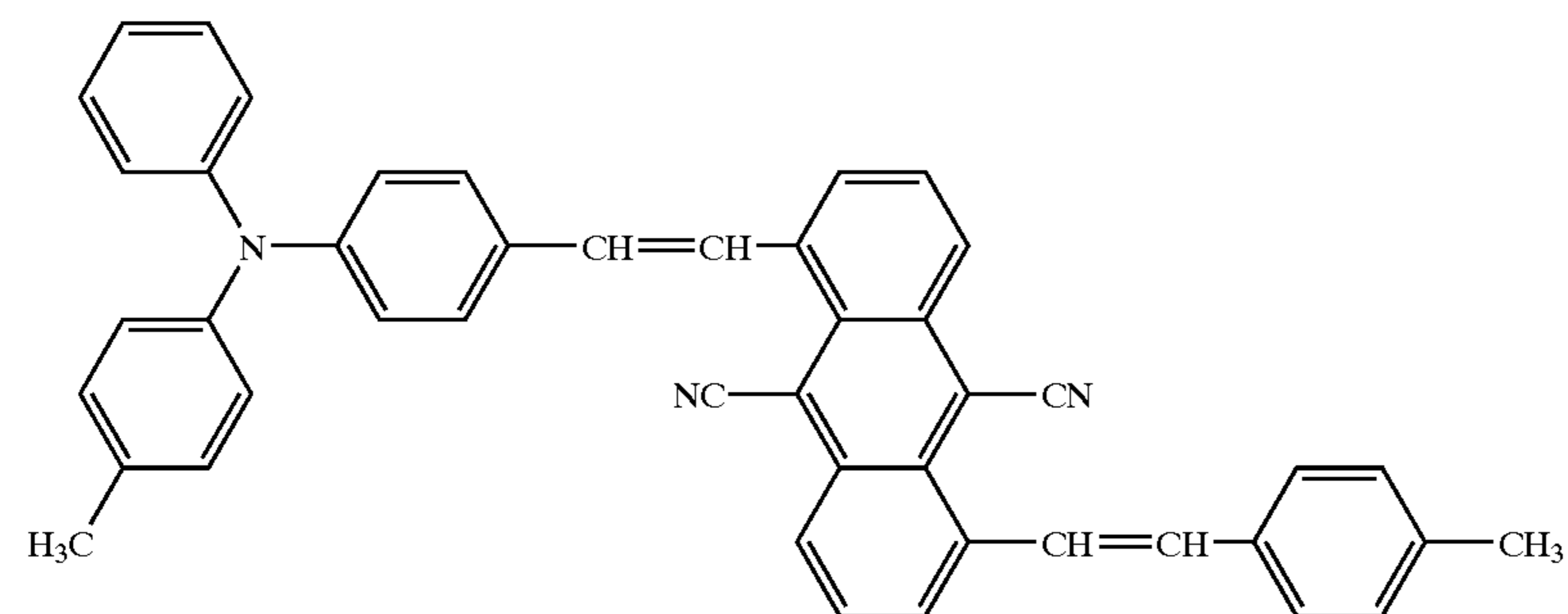
Structural formula (10)-7:
