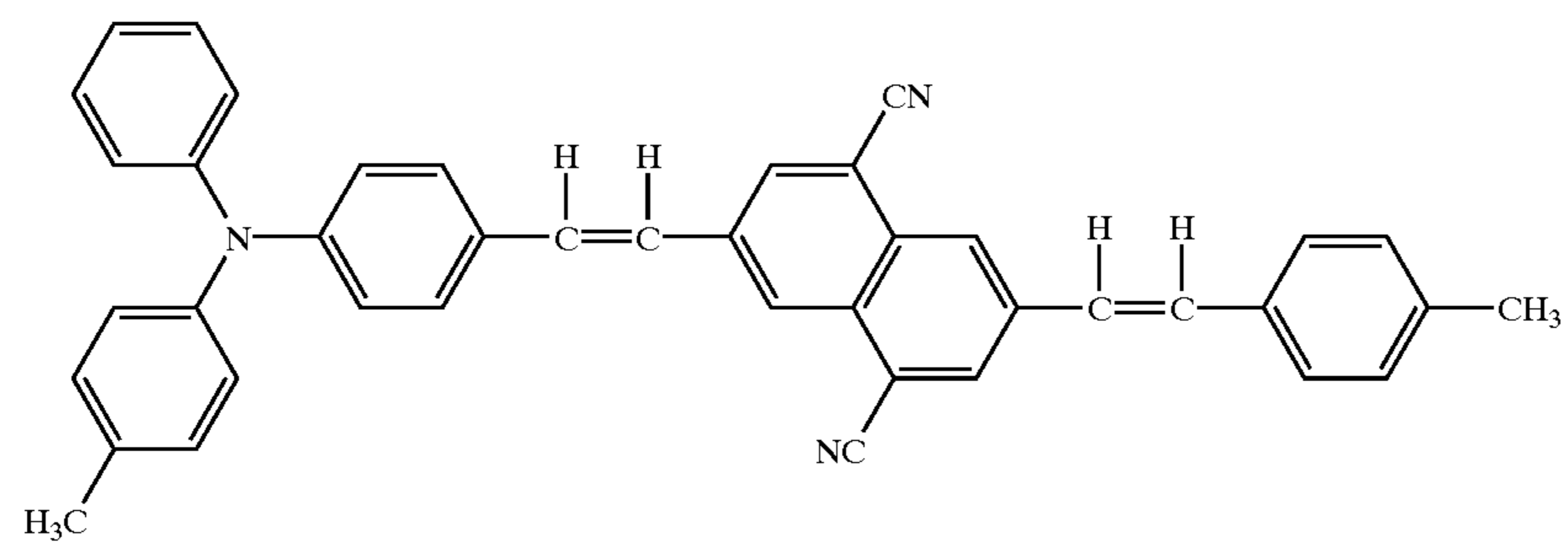
Structural formula (10)-3:
