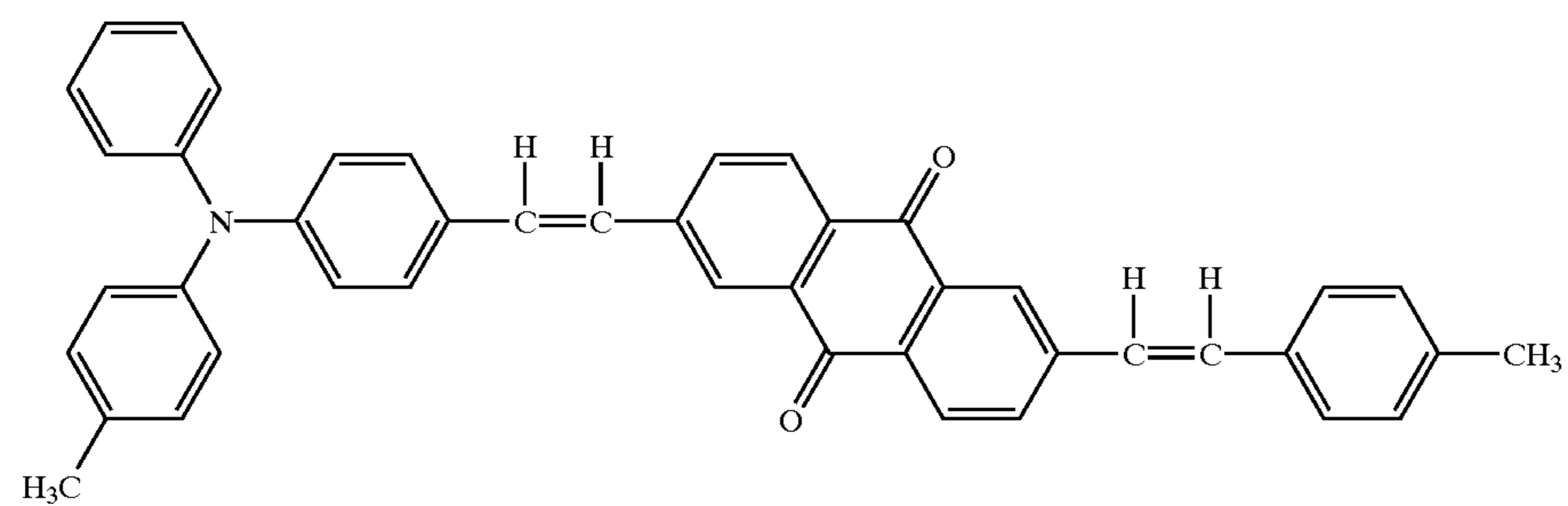
Structural formula (10)-9:
