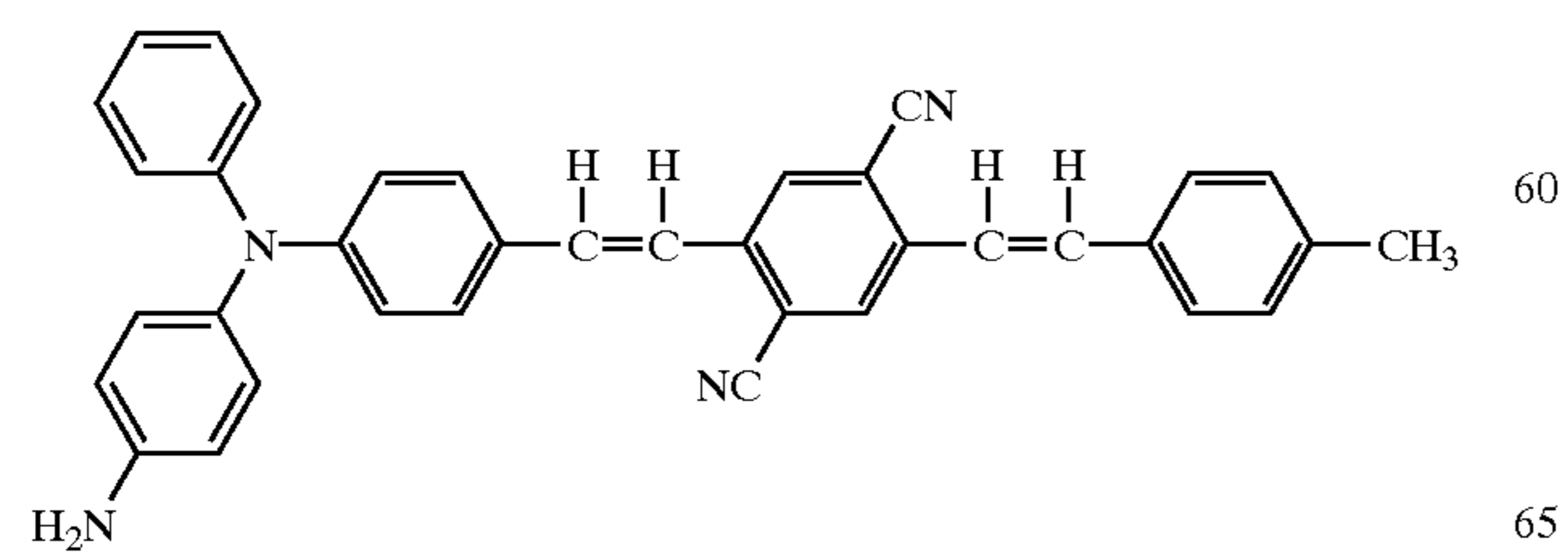
Structural formula (10)-11:
