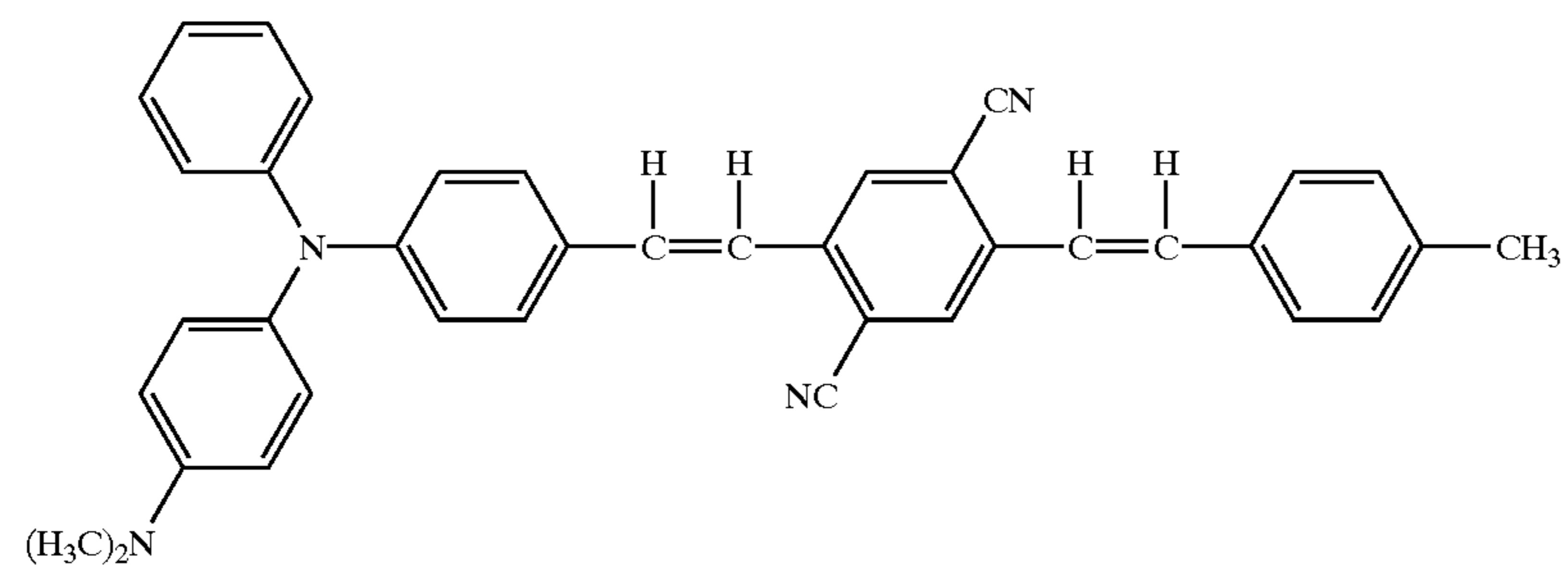
Structural formula (10)-10:
