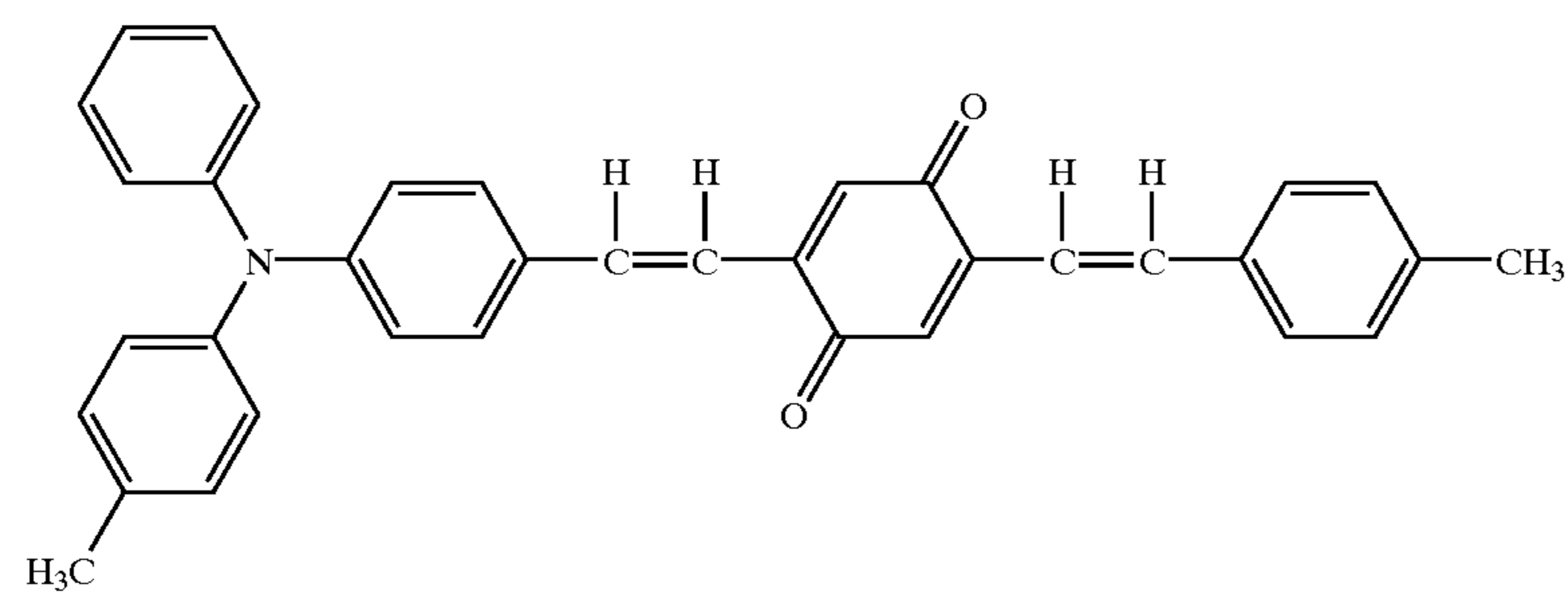
Structural formula (10)-8:
