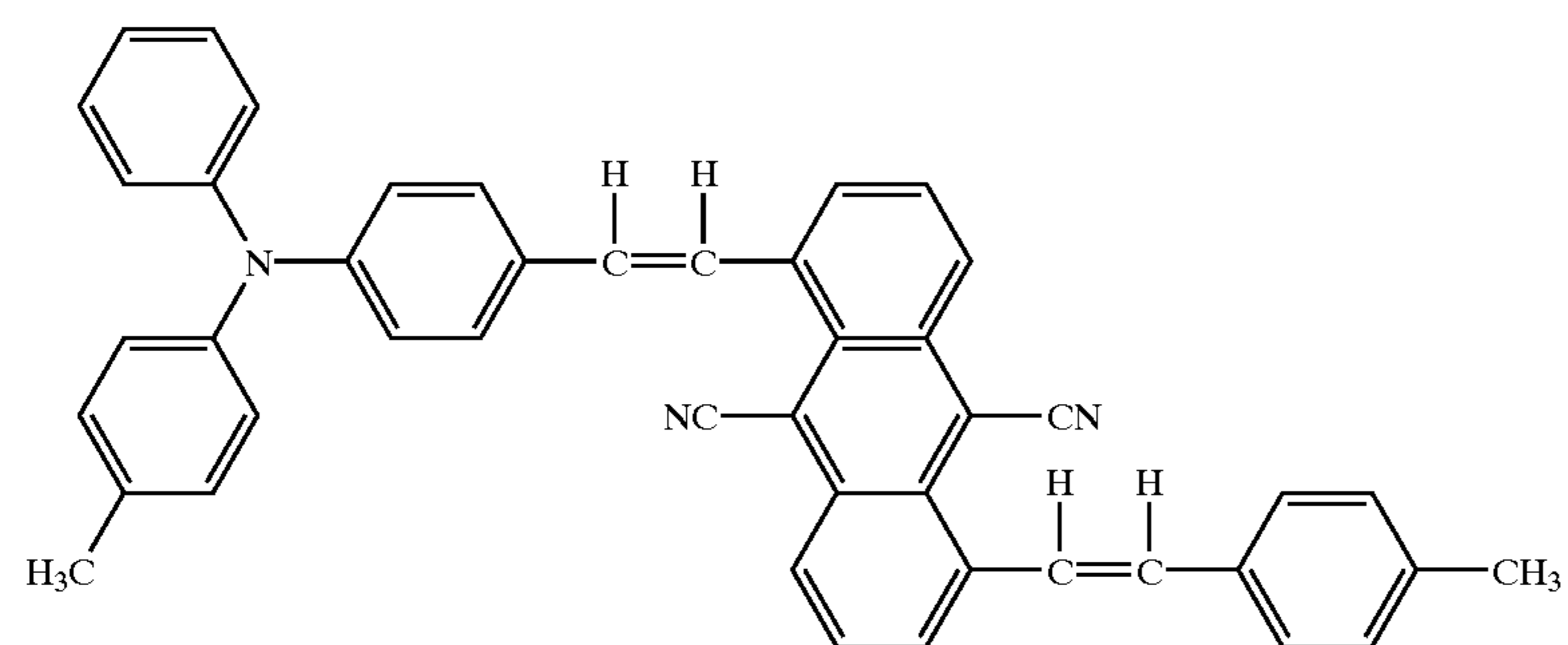
Structural formula (10)-6:
