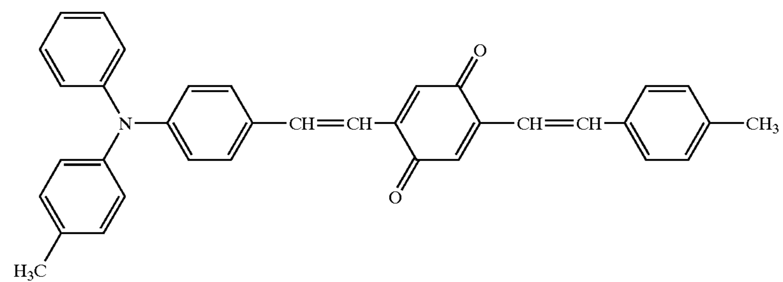
Structural formula (10)-8:
