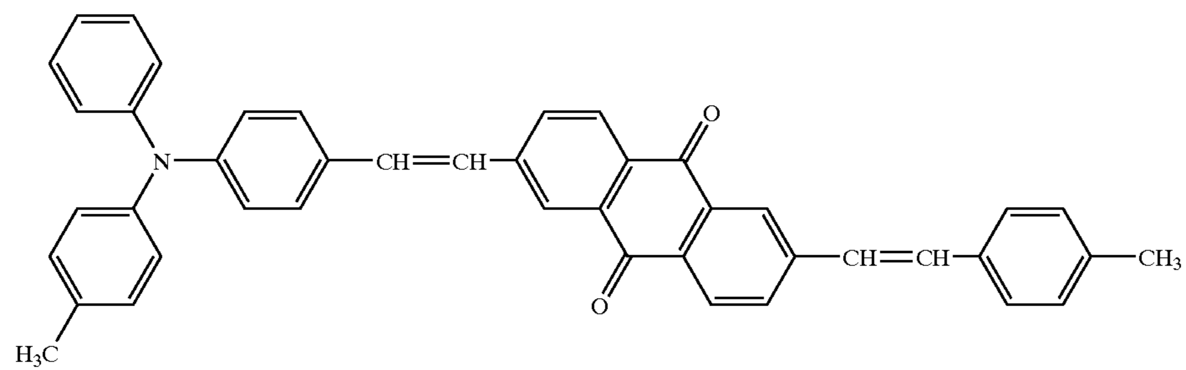
Structural formula (10)-8:
