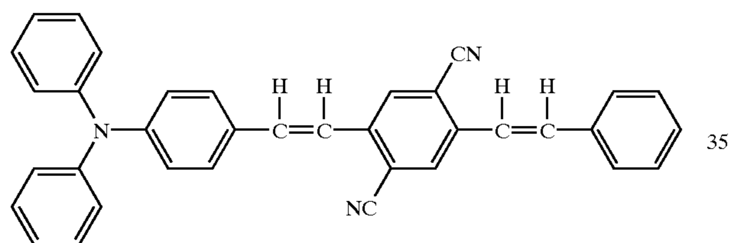
Structural formula (10)-10:
