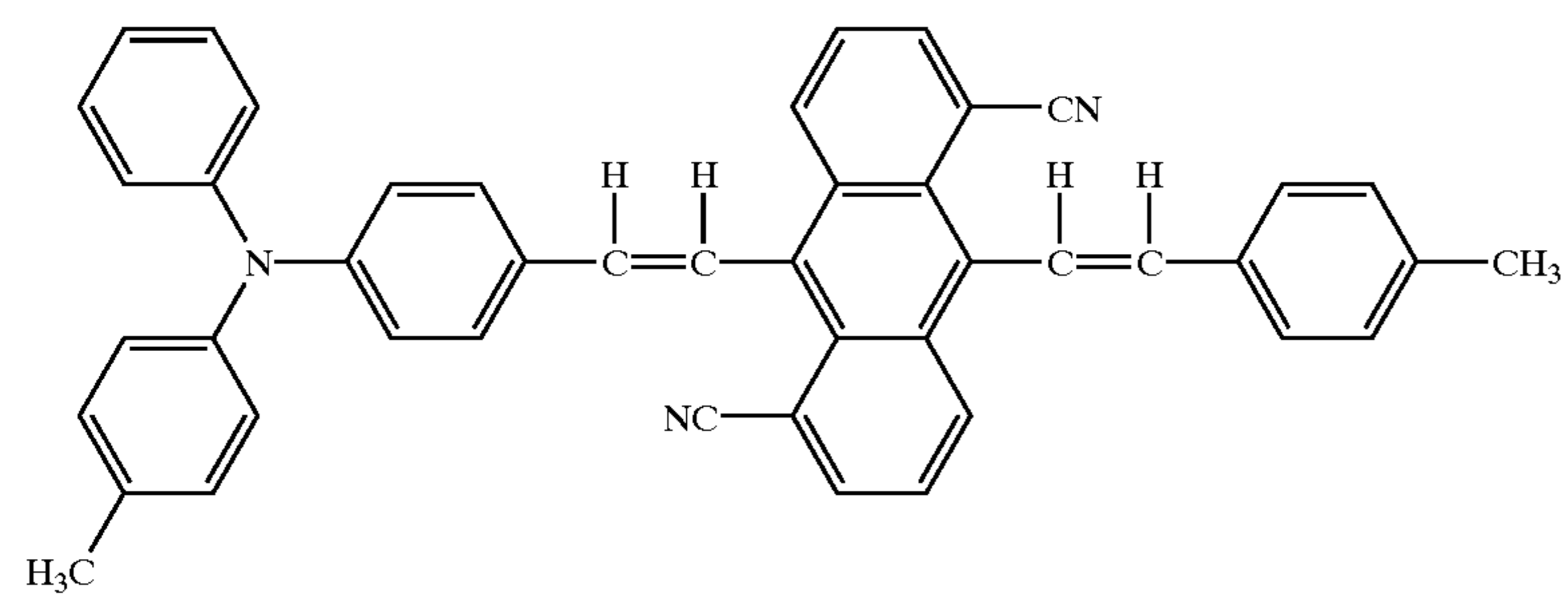
Structural formula (10)-6:
