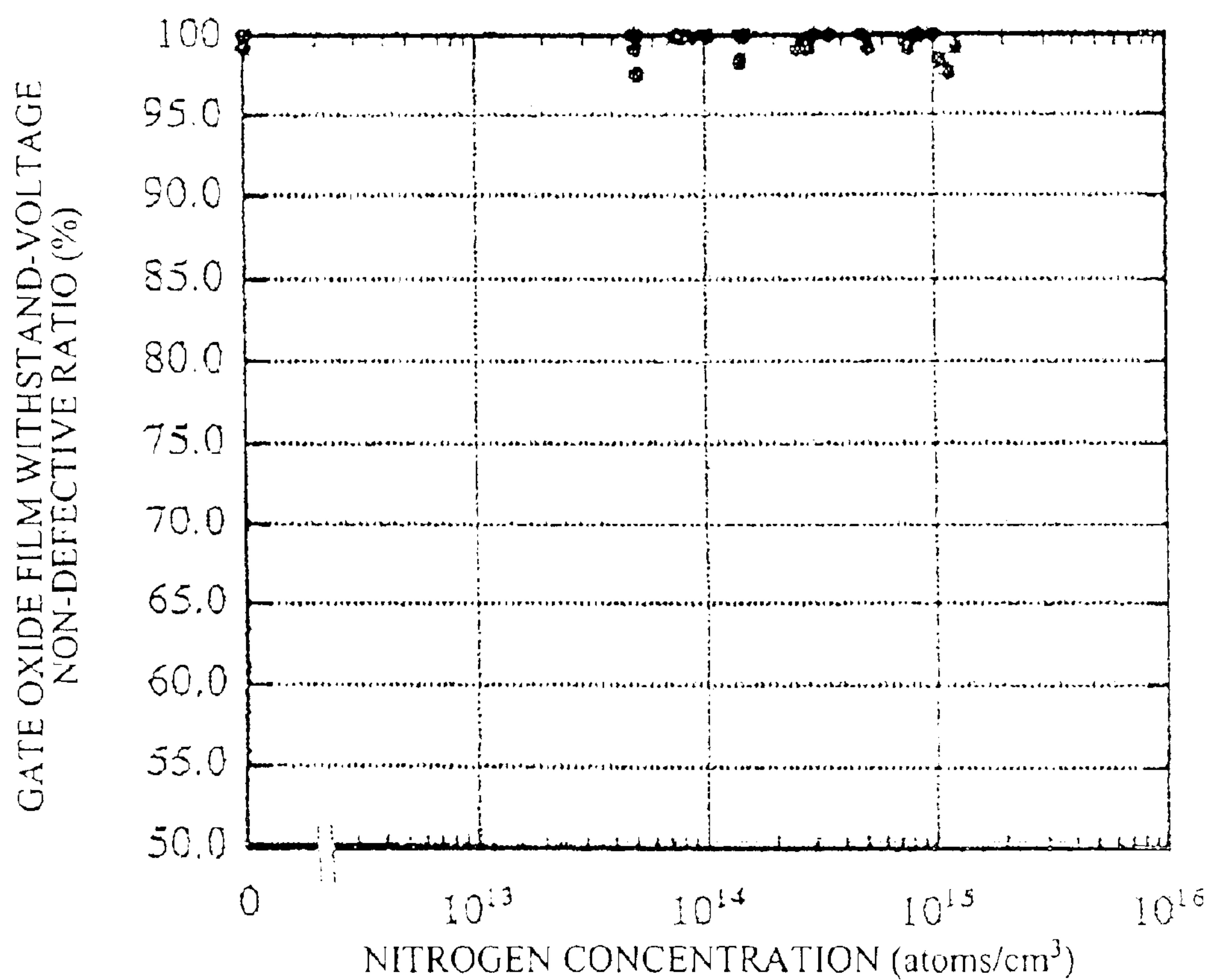
RELATIONSHIP BETWEEN ADDED NITROGEN CONCENTRATION AND OXIDE FILM WITHSTAND-VOLTAGE NON-DEFECTIVE RATIO AFTER HYDROGEN ANNEALING
