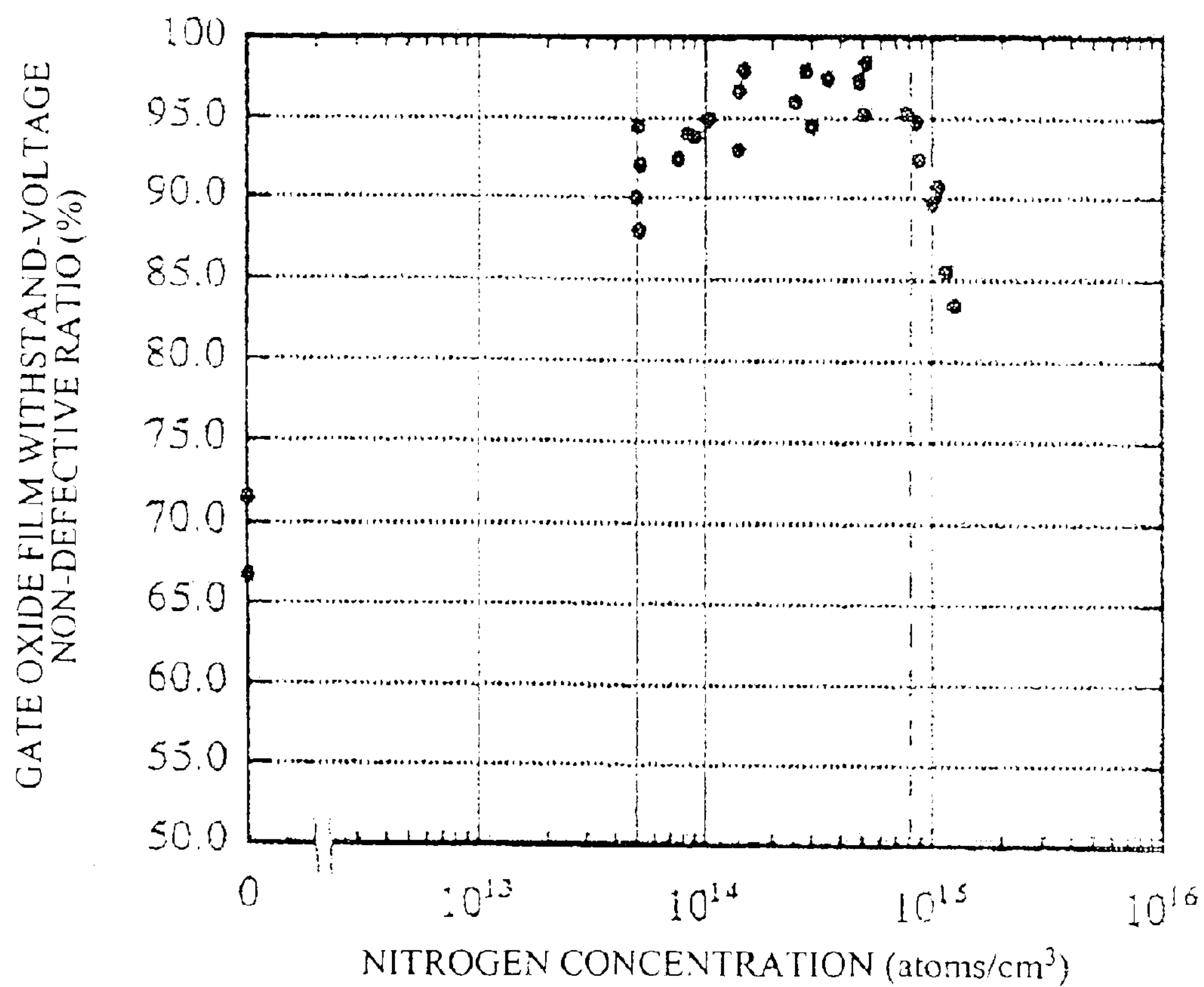
RELATIONSHIP BETWEEN ADDED NITROGEN CONCENTRAION AND OXIDE FILM WITHSTAND-VOLTAGE NON-DEFECTIVE RATIO AFTER REMOVAL BY POLISHING SURFACE LAYER OF 3 \mu\text{m} AFTER HYDROGEN ANNEALING
