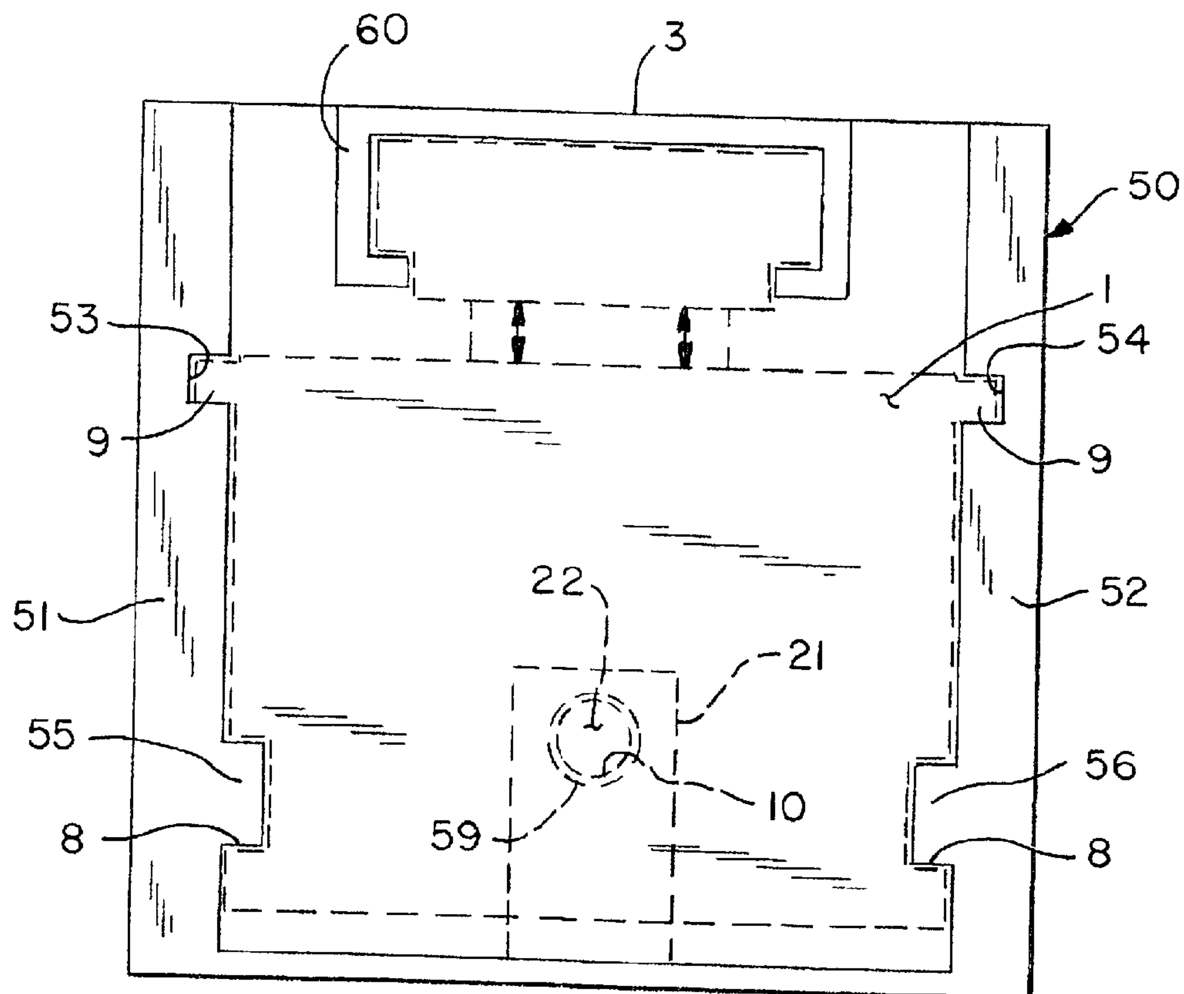
FIG. 5 (PRIOR ART)
