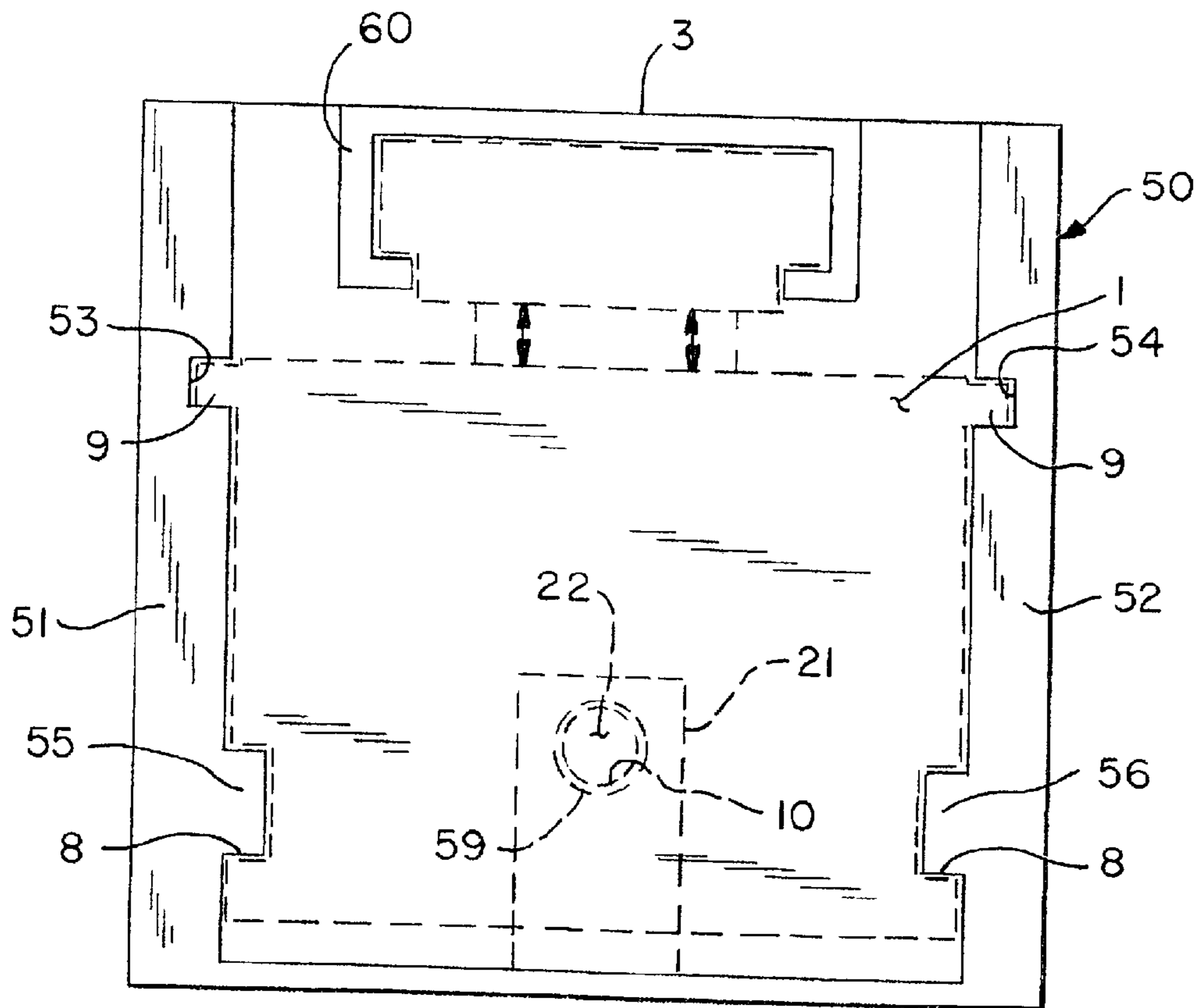
FIG. 5 (PRIOR ART)
