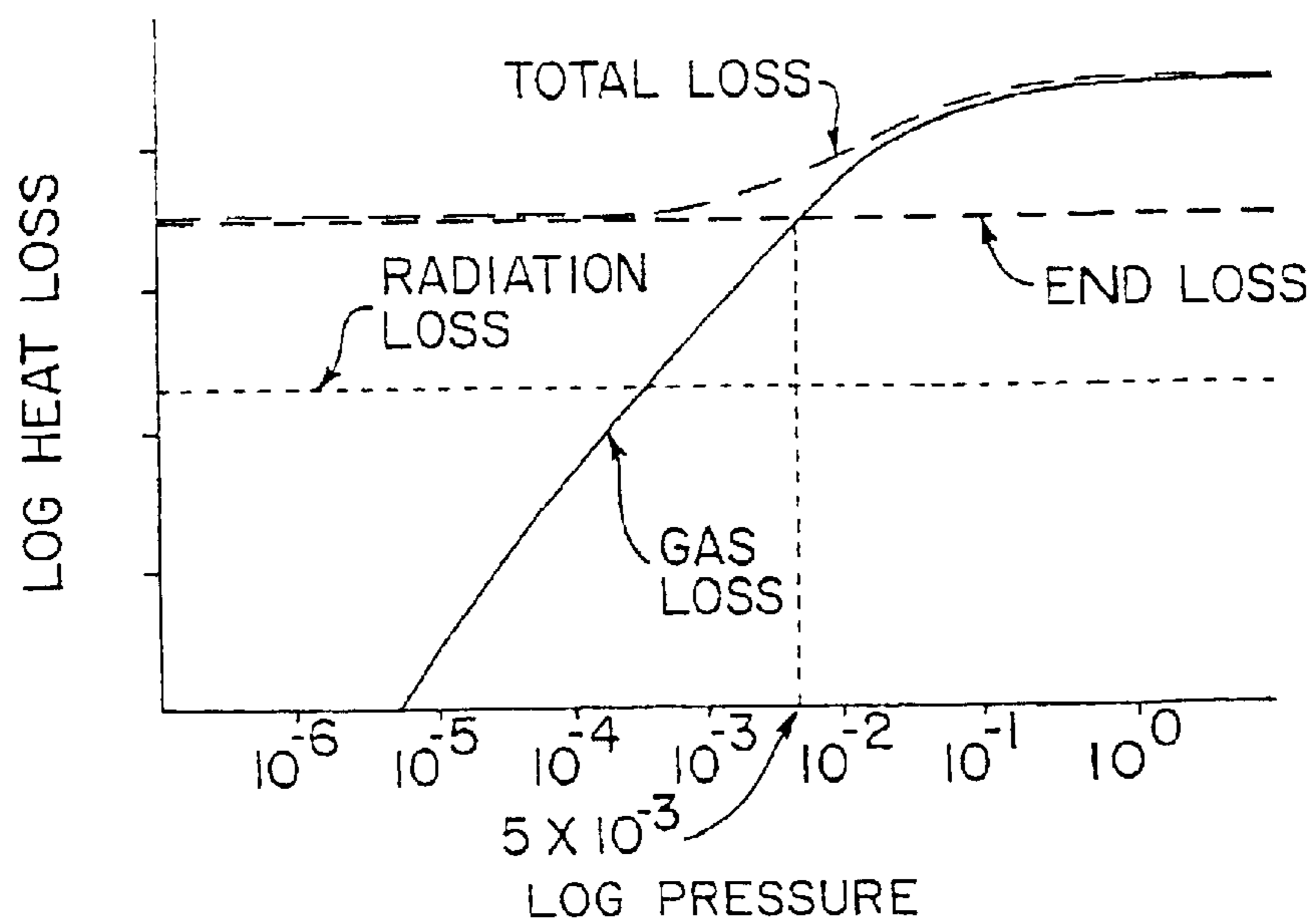
FIG. 2 PRIOR ART
